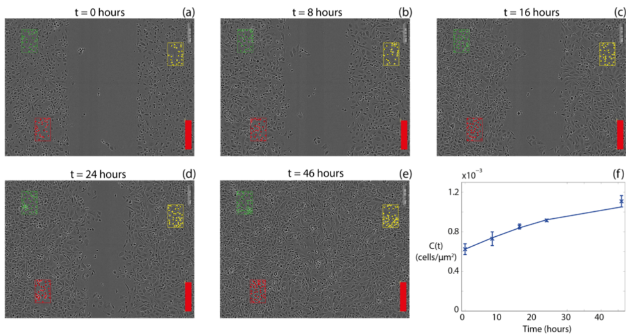
Fig. 3 a-e Time evolution of an EGF-75 IncuCyte ZOOM™ assay. Images taken after (a) 0, (b) 8, (c) 16, (d) 24, and (e) 46 h after the scratch was performed. The three coloured boxes indicate the location of the three subregions used to calculate K and \lambda . Each coloured square within the subregions indicates the centre of an individual cell in the cell counting step. Scale bar corresponds to 300 μm. f Comparison of the average experimental cell density C(t) (crosses) and the logistic growth curve using our estimates of K and \lambda (solid)
