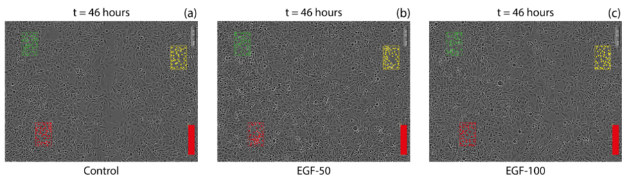
Fig. 2 Final time experimental images ( t = 46 hours) for three IncuCyte ZOOM™ assays for (a) Control, (b) EGF-50, and (c) EGF-100. The three coloured boxes indicate the location of the three subregions used to estimate K and \lambda . Each coloured square within the subregions indicates the centre of an individual cell in the cell counting step. Scale bar corresponds to 300 \mu\text{m}
