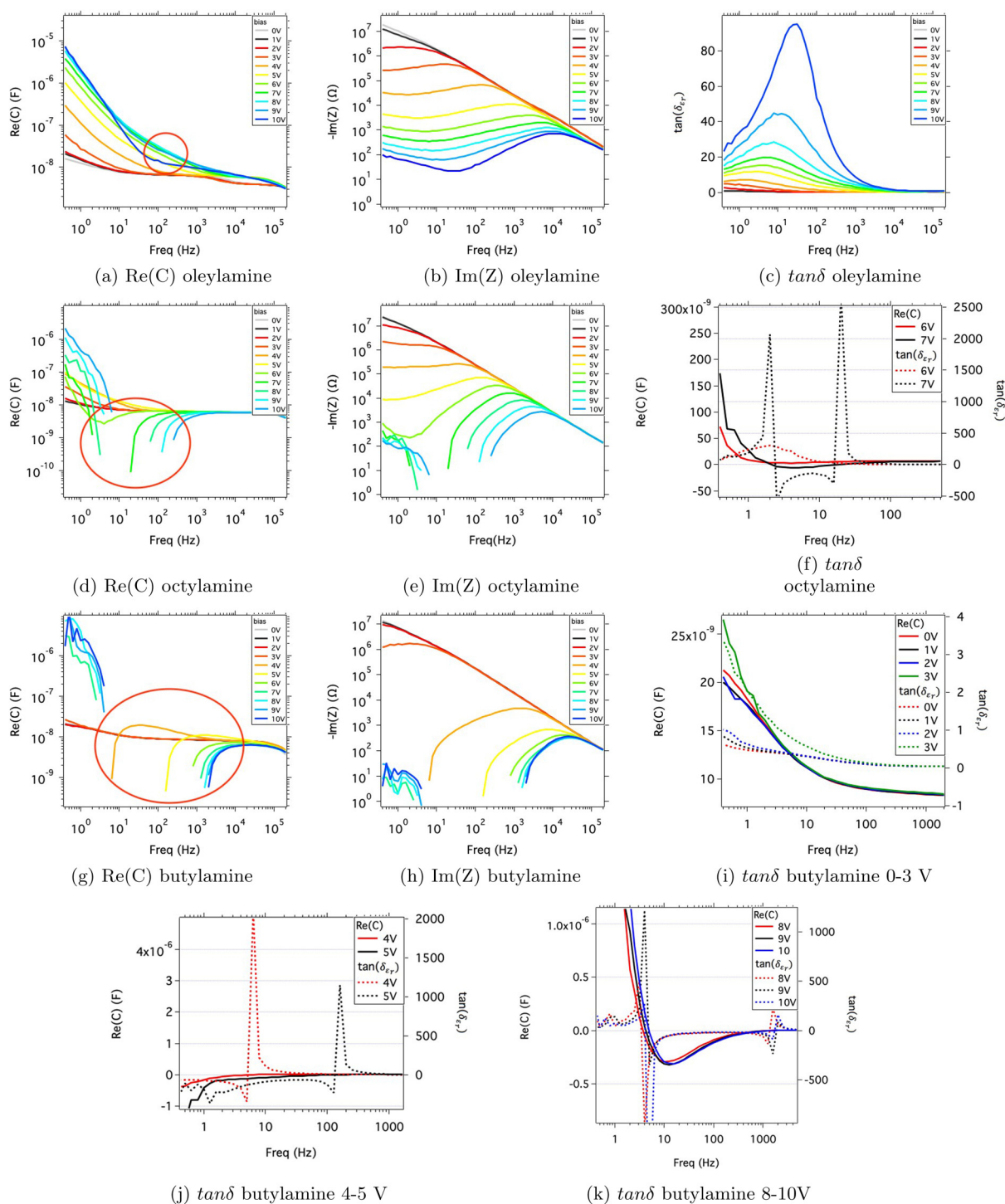
FIG. 2. Summary of the real part of the capacitance, the imaginary part of the impedance, and the capacitance loss factor of a QLED with insulating ligands of different length. Figures 2(a)–2(c) summarise the oleylamine case. Figures 2(d)–2(f) sum up the octylamine case. Figures 2(g)–2(k) conclude the butylamine case.
