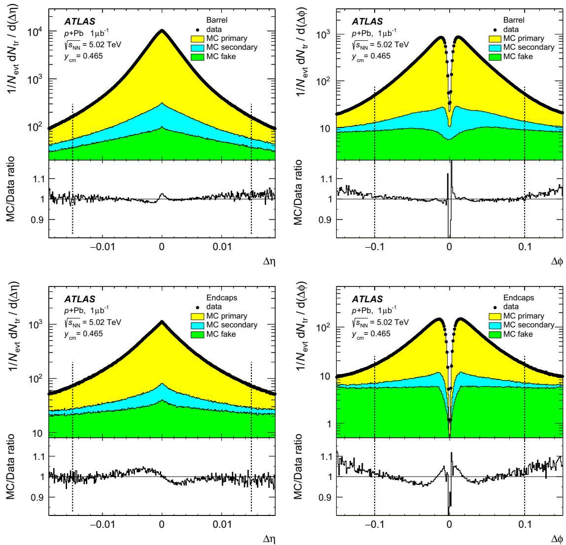
Fig. 4 Stacked histograms for the differences between the hits of the tracklet in outer and inner detector layers in pseudorapidity \Delta\eta (left) and in azimuth \Delta\phi (right) for the tracklets reconstructed with Method 1 measured in the data (points) and simulation (histograms) in p + \text{Pb}
