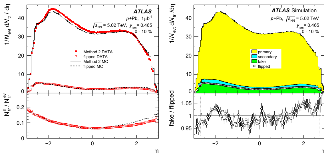
Fig. 5 \eta -distribution of the number of tracklets reconstructed with Method 2. Left top panel comparison of the simulation (lines) to the data (markers). The results of the flipped reconstruction are shown with open markers for data and dashed line for simulation. Right top panel the simulated result for three contributions: primary, secondary and fake
