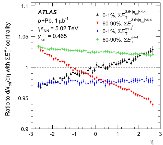
Fig. 9 Ratios of dN_{\text{ch}}/d\eta obtained using alternative centrality definitions to the nominal results presented in this paper as a function of \eta for the 0–1 and 60–90 % centrality bins
