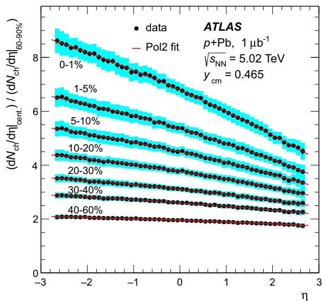
Fig. 8 Ratios of dN_{\text{ch}}/d\eta distributions measured in different centrality intervals to that in the peripheral (60–90 %) centrality interval. Lines show the results of second-order polynomial fits to the data points
