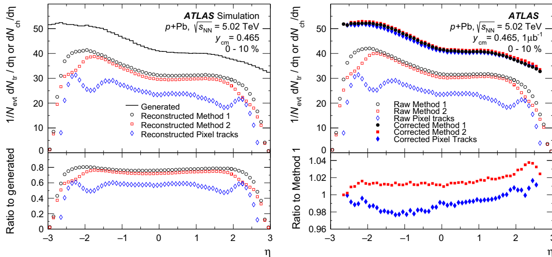
Fig. 6 Left top distribution from the MC simulation for the generated number of primary charged particles per event ( dN_{\text{ch}}/d\eta ) shown with line, reconstructed number per event ( 1/N_{\text{evt}}dN_{\text{tr}}/d\eta ) of tracklets from Method 1 shown with circles, tracklets from Method 2 after flipped event subtraction shown with squares, and pixel tracks shown with diamonds. Left bottom the ratio of reconstructed to generated tracklets and pixel
