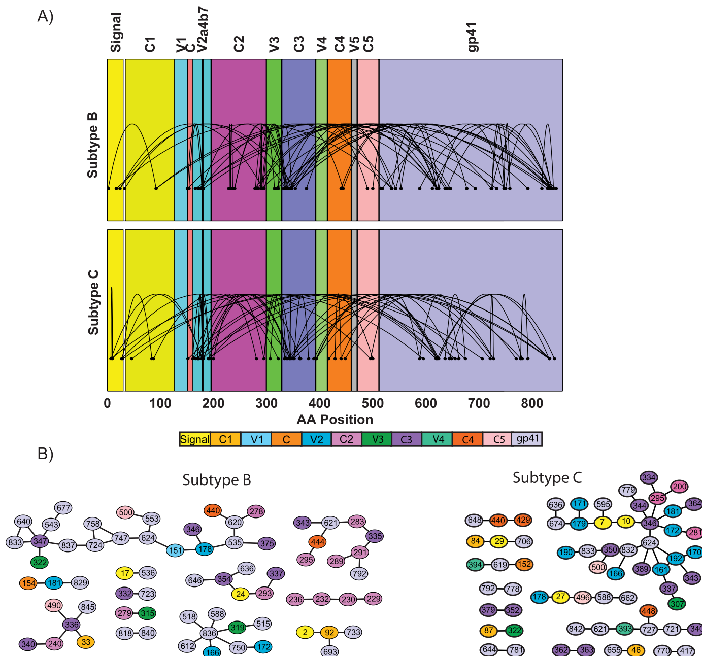
Fig 3. The collection of optimal pairs displayed relative to the domains of Env. A) over a linear representation and B) as networks.
