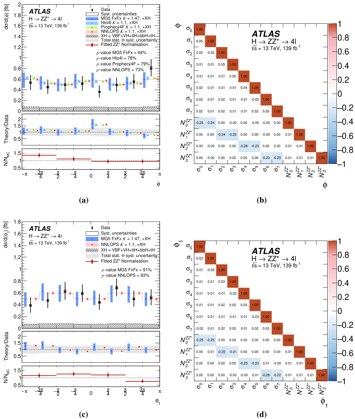
Fig. 23 Differential fiducial cross sections for a the azimuthal angle, \phi , between the decay planes of the two reconstructed Z bosons and c the azimuthal angle, \phi_1 , between the decay plane of the leading Z boson
