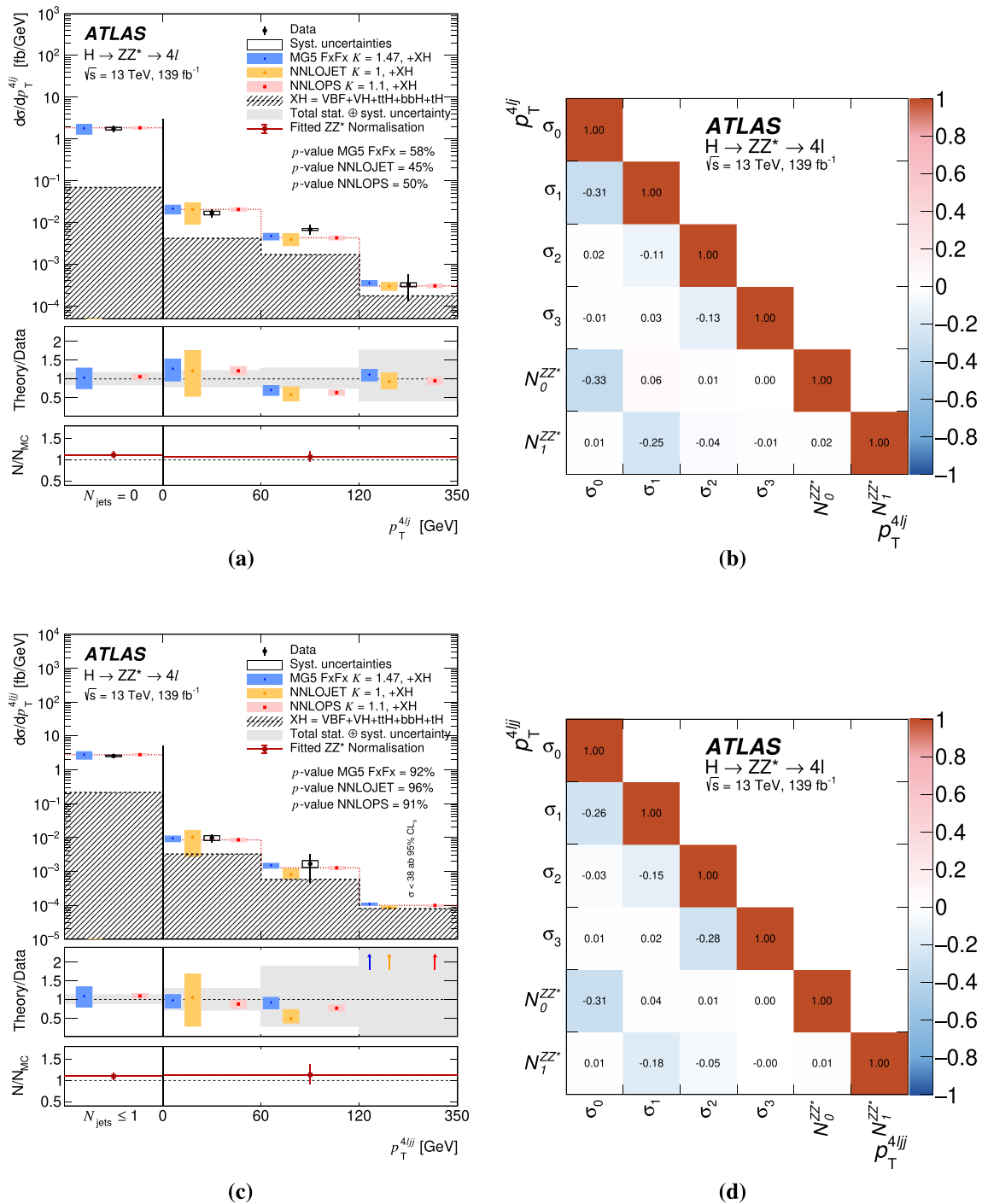
Fig. 29 Differential fiducial cross sections for a the transverse momentum of the four-lepton plus jet system, in events with at least one jet, and c the transverse momentum of the four-lepton plus dijet system,
