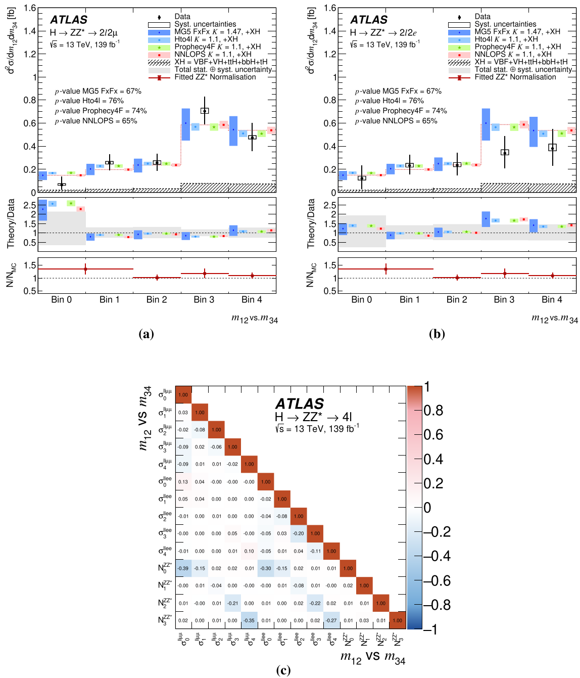
Fig. 32 Differential fiducial cross sections for the leading vs. subleading Z boson mass, m_{12} vs. m_{34} , in a \ell\ell\mu\mu and b \ell\ell ee final states, along with c their corresponding correlation matrix between the measured cross sections and the ZZ^* background normalisation factors. The bin boundaries are defined in Fig. 12
