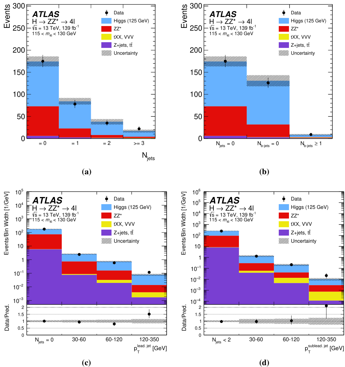
Fig. 7 The observed and expected (pre-fit) distributions of a N_{\text{jets}} , b N_{b\text{-jets}} , c p_T^{\text{lead.j}} , and d p_T^{\text{sublead.j}} in the mass region 115 < m_{4\ell} < 130 GeV, for an integrated luminosity of 139 \text{ fb}^{-1} collected at \sqrt{s} = 13 TeV. A SM Higgs boson signal with a mass m_H = 125 GeV is assumed. In distribution c , the first bin contains events with zero jets,
