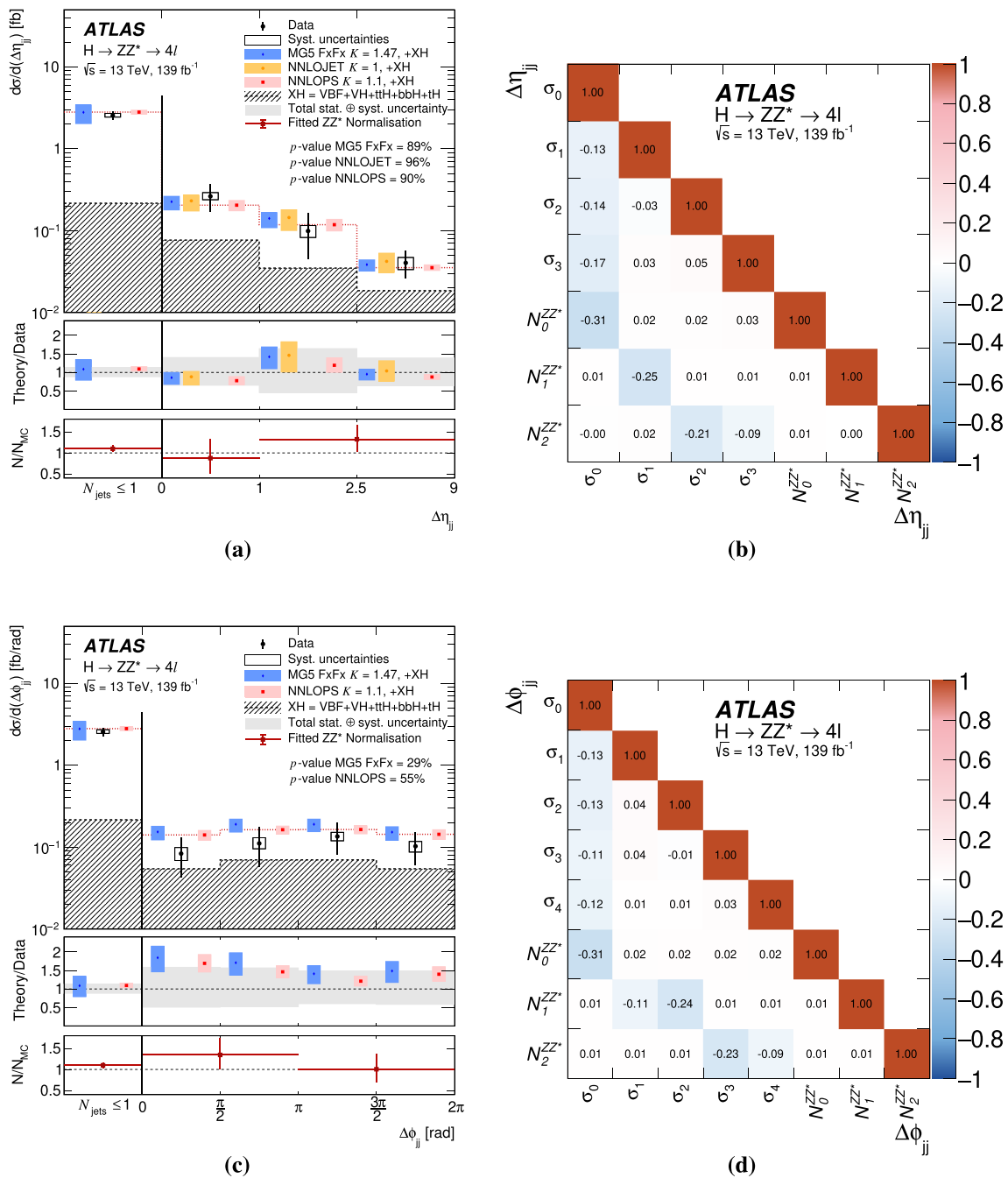
Fig. 28 Differential fiducial cross sections for a the distance between these two jets in pseudorapidity, \Delta\eta_{jj} , and c the distance between the two jets in \phi , \Delta\phi_{jj} . The first bin contains events with fewer than two
