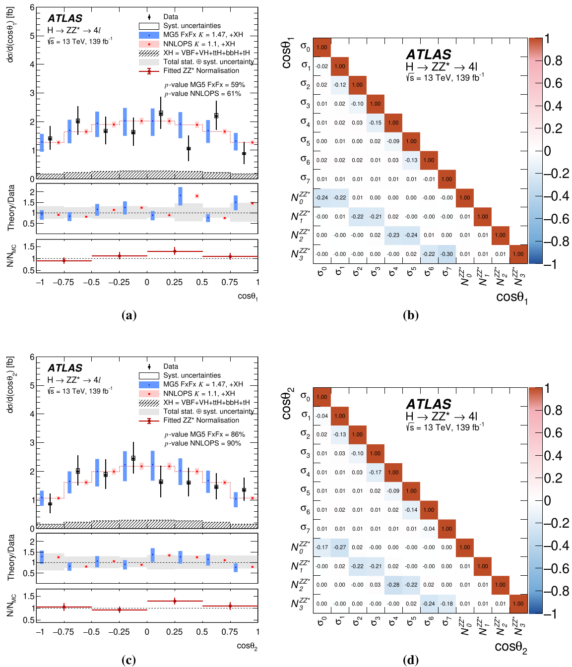
Fig. 22 Differential fiducial cross sections for a production angle, \cos\theta_1 , of the anti-lepton from the leading Z boson and c the production angle, \cos\theta_2 , of the anti-lepton from the subleading Z boson. The cor-
