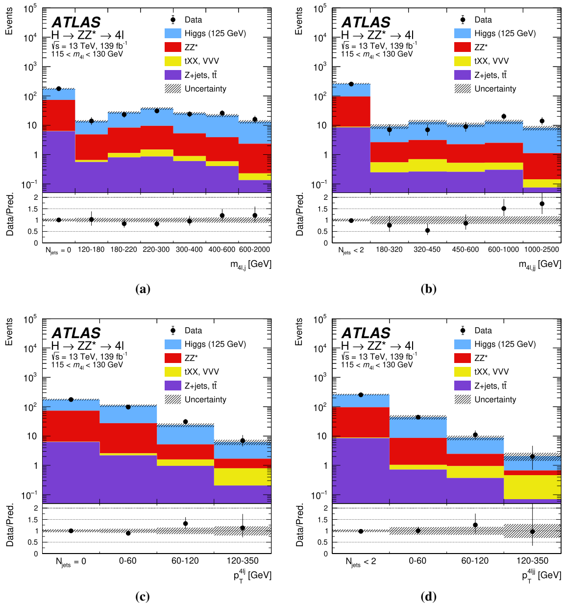
Fig. 9 The observed and expected (pre-fit) distributions of a m_{4\ell j} , b m_{4\ell jj} , c p_T^{4\ell j} , and d p_T^{4\ell jj} in the mass region 115 < m_{4\ell} < 130 GeV, for an integrated luminosity of 139 \text{ fb}^{-1} collected at \sqrt{s} = 13 TeV. A SM Higgs boson signal with a mass m_H = 125 GeV is assumed. The
