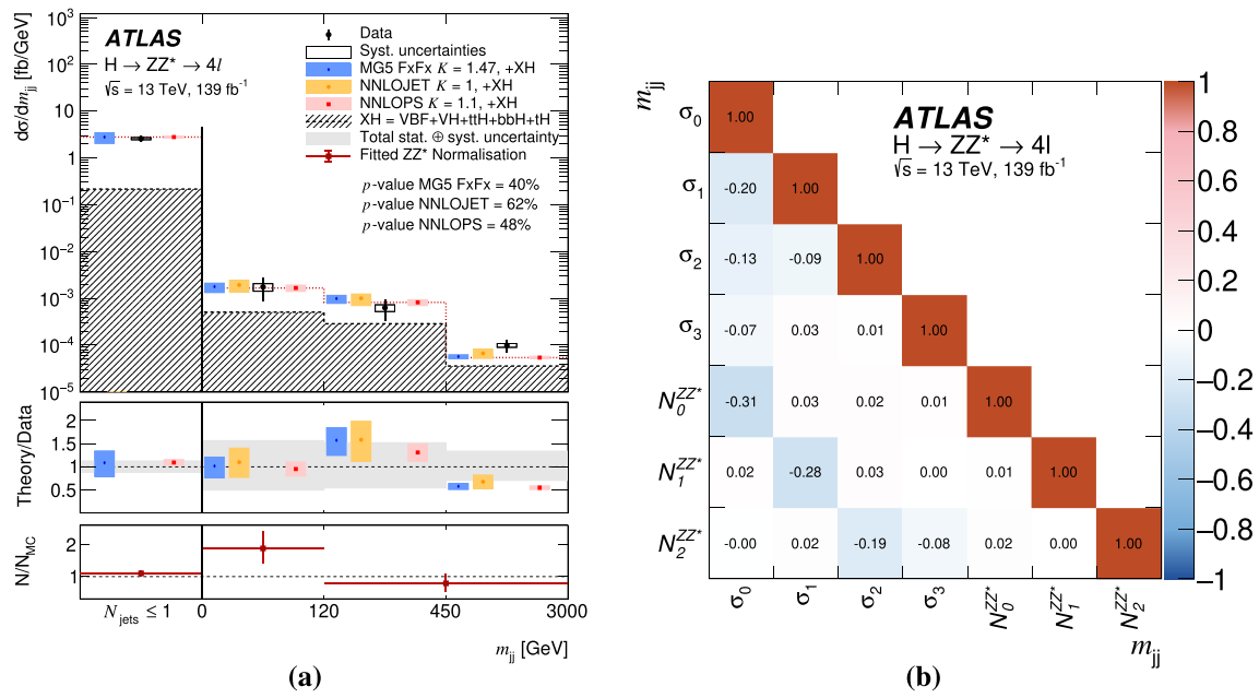
Fig. 27 Differential fiducial cross sections for a the invariant mass of the two highest- p_T jets, m_{jj} , in events with at least two jets. The corresponding correlation matrix between the measured cross sections and the ZZ^* background normalisation factors is also provided ( b )
