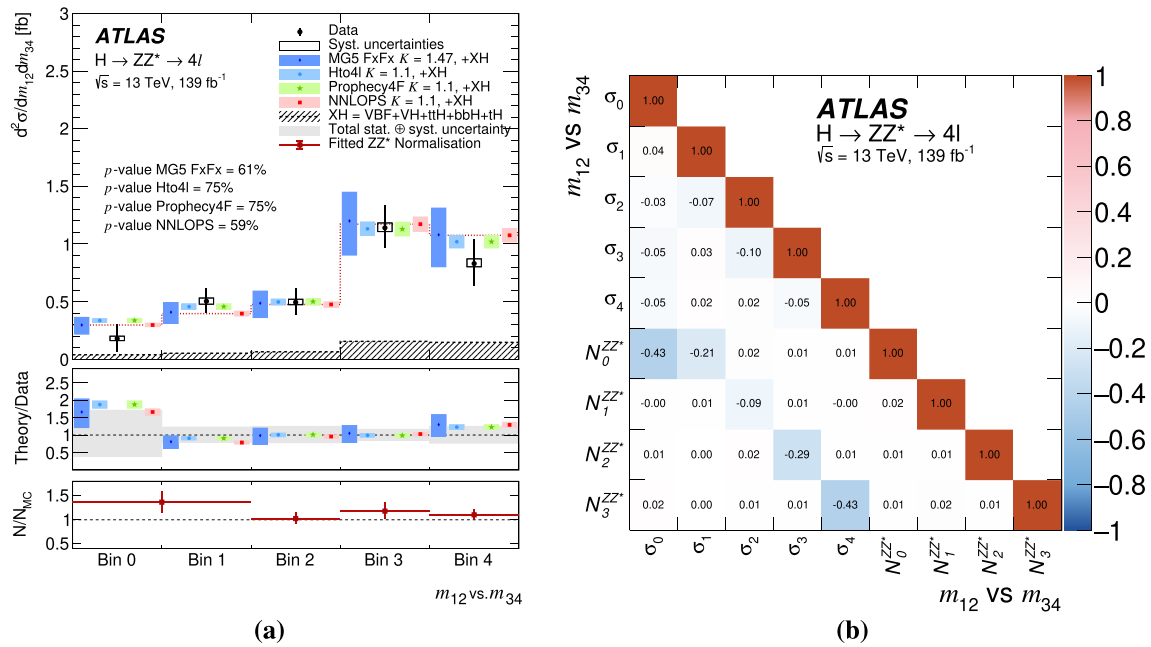
Fig. 31 a Differential fiducial cross section for the leading vs. subleading Z boson mass, m_{12} vs. m_{34} , and b the corresponding correlation matrix between the measured cross sections and the ZZ^* background normalisation factors. The bin boundaries are defined in Fig. 12
