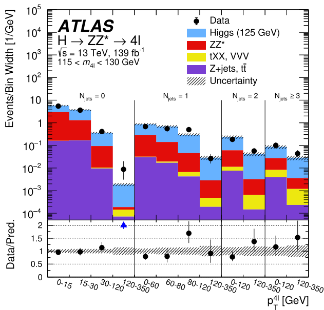
Fig. 10 The observed and expected (pre-fit) distributions of p_T^{4\ell} in N_{\text{jets}} bins in the mass region 115 < m_{4\ell} < 130 GeV, for an integrated luminosity of 139 \text{ fb}^{-1} collected at \sqrt{s} = 13 TeV. A SM Higgs boson signal with a mass m_H = 125 GeV is assumed. The uncertainty in the prediction is shown by the hatched band, which includes the theoretical uncertainties of the SM cross section for the signal and the ZZ^* background
