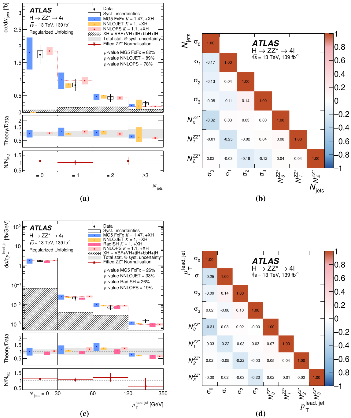
Fig. 42 a, c Differential fiducial cross sections as a function of the jet multiplicity, N_{\text{jets}} , and leading jet p_T in events with at least one jet, using a regularised matrix unfolding with the \tau parameters set to 0.6
