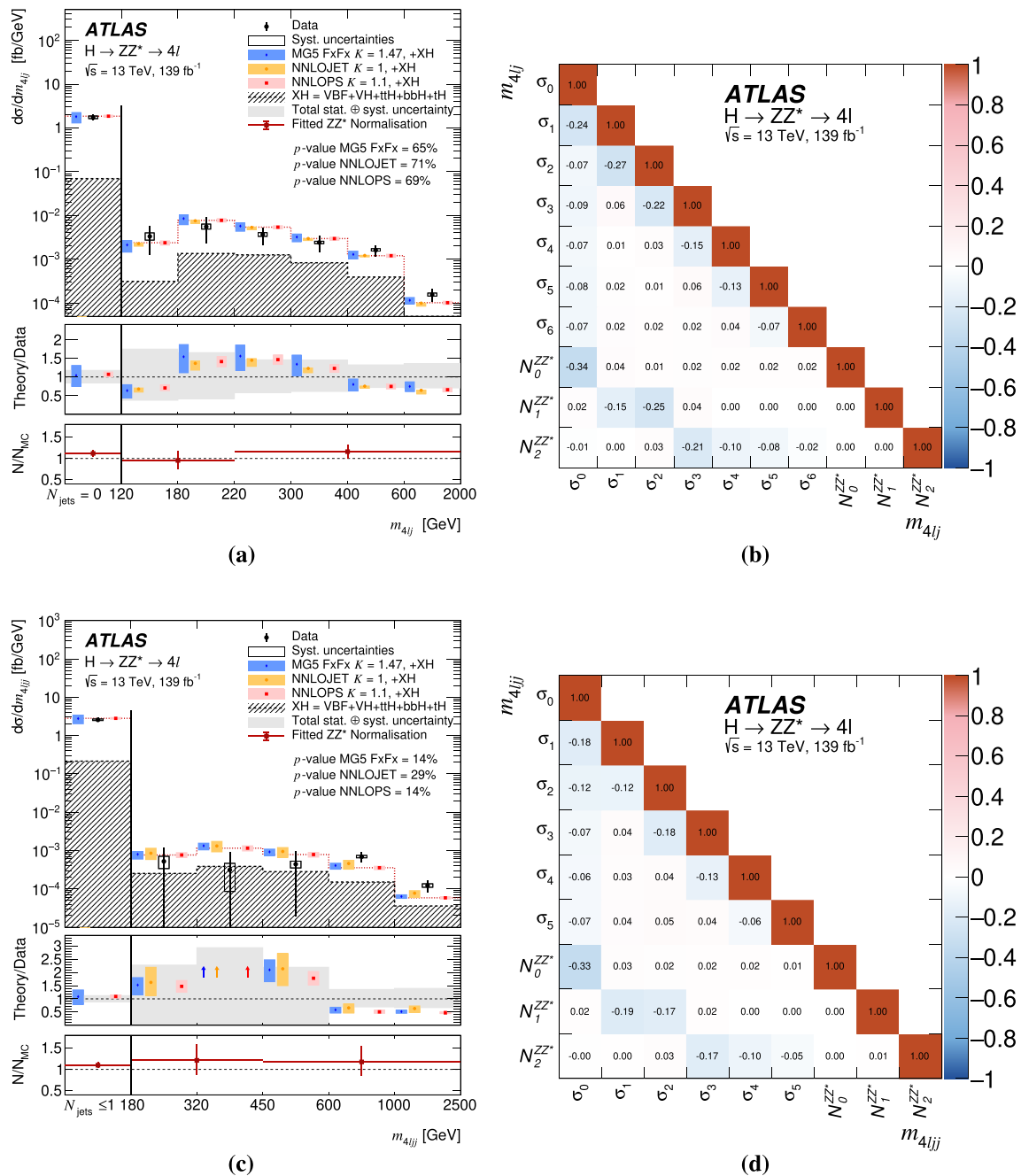
Fig. 30 Differential fiducial cross sections for a the invariant mass of the four-lepton plus jet system, in events with at least one jet, and c the invariant mass of the four-lepton plus dijet system, in events with
