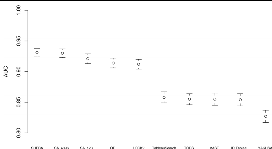
Figure 1 AUC for different methods for 200 queries in the ASTRAL 95% data set. Area under the ROC curve (AUC) for different methods on the 200 query set against the ASTRAL SCOP 95% sequence identity non-redundant database, excluding comparisons of a structure against itself. Each AUC value is shown with a 95% confidence interval. SA refers to SA Tableau Search (followed by number of restarts) and QP refers to QP Tableau Search. SARF2 is not present in this graph, as it is unable to process a data set this large, and DaliLite is not present as it exceeds the CPU time limit.
