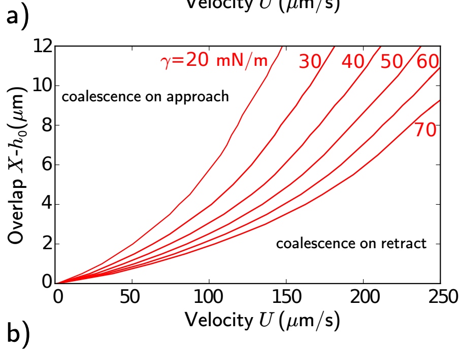
Figure 6 Interaction between two air bubbles in water containing 10 mM salt solution for varying drive velocities U and overlap X - h_0 . a) Stability map for interfacial tension 70 mN/m. The red and blue regions indicate coalescence on approach and retract respectively. b) Curves showing the boundary between coalescence on approach and coalescence on retract for varying interfacial tensions. The bubbles are initially separated by a distance h_0 , before being driven together over a distance X = 20 \mu\text{m} with velocity U , and then pulled apart with velocity -U . The bubble radii R_1 and R_2 are 59.5 and 45 \mu\text{m} respectively, and the surface potential of the air-water interface is -72 mV. All other parameters are listed in Table S3.
