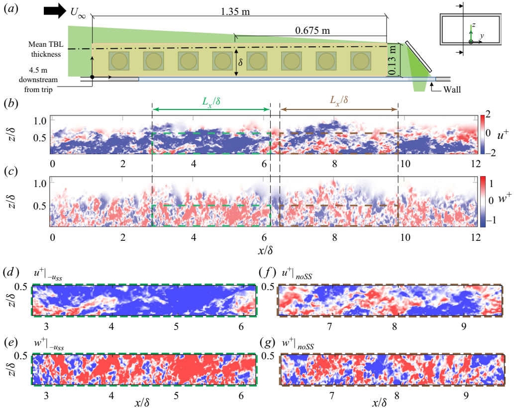
Figure 3. Schematic of the experimental set-up used to conduct LFOV PIV experiments in the streamwise wall-normal plane ( x – z ) in the HRNBLWT. Green shading indicates flow illuminated by the laser while the orange shading indicates the flow field cumulatively captured by the PIV cameras (shown in the background). Dash-dotted black line represents the streamwise evolution of the boundary layer thickness, with \delta defined at the centre of the full flow field. (b,c) Instantaneous (b) u^+ and (c) w^+ -fluctuations from the LFOV PIV dataset at Re_\tau \approx 2500 . The dashed green box in (b,c) identifies a low-momentum turbulent superstructure ( -u_{ss} ) of length L_x based on the superstructure extraction algorithm described in § 2.2. (d,e) Show an expanded view of the u - and w -fluctuations within -u_{ss} , as identified in (b,c), respectively. Alternatively, the dashed brown box in (b,c) represents flow field of the same length \times height as the dashed green box, but not associated with a turbulent superstructure ( noSS ). (f,g) Show an expanded view of the u - and w -fluctuations within the noSS region identified in (b,c), respectively.
