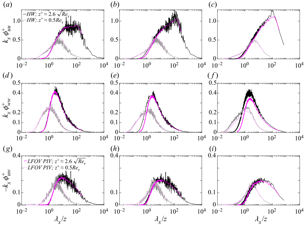
Figure 14. Premultiplied 1-D spectra of (a–c) u -fluctuations, (d–f) w -fluctuations and (g–i) co-spectra of the Reynolds shear stress at Re_\tau \approx (a,d,g) 2500, (b,e,h) 5000 and (c,f,i) 7500. Lines in magenta correspond to the spectra estimated from the LFOV PIV datasets documented in table 1 , while the lines in black correspond to the same computed from the multi-wire data acquired by Baidya et al. (2017) (at Re_\tau \approx 2500 and 5000) and Morrill-Winter et al. (2015) (at Re_\tau \approx 7500 ), in the same wind tunnel facility. Dark shaded lines correspond to spectra at z^+ \approx 2.6\sqrt{Re_\tau} , while light shaded lines correspond to z^+ \approx 0.5Re_\tau .
