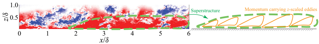
Figure 13. Conceptual representation of the main conclusion of this study: z -scaled eddies are likely the constituent motions forming the turbulent superstructures.
