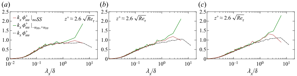
Figure 8. Premultiplied 1-D spectra of the u -fluctuations plotted vs \lambda_x/\delta at z^+ \approx 2.6\sqrt{Re_\tau} for Re_\tau \approx (a) 2500, (b) 5000 and (c) 7500. The mean spectrum estimated from the full flow field (in black lines) is ensembled across all 3000 fields. While, the conditional spectrum corresponds to extracted flow fields ( \sim 300 ) of the same length \times height associated (in green) and not associated (in brown) with the superstructures.
