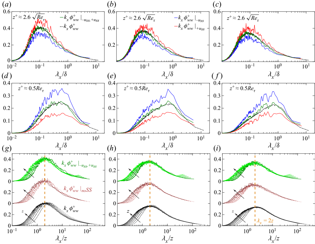
Figure 9. (a–f) Premultiplied 1-D spectra of the w -fluctuations plotted vs \lambda_x/\delta at (a–c) z^+ \approx 2.6\sqrt{Re_\tau} and (d–f) z^+ \approx 0.5Re_\tau for large FOV PIV data at Re_\tau \approx (a, d, g) 2500, (b, e, h) 5000 and (c, f, i) 7500. Dashed black lines correspond to the mean spectra obtained by ensembling across 3000 PIV images of the full flow field while the solid blue and red lines represent conditional spectra computed from the extracted w -flow fields associated with -u_{ss} and +u_{ss} , respectively. The spectrum in green corresponds to all extracted w -flow fields, associated with both -u_{ss} and +u_{ss} . (g–i) Premultiplied 1-D spectra of w -velocity plotted vs \lambda_x/z at various z^+ within the log region ( 2.6\sqrt{Re_\tau} \lesssim z^+ \lesssim 0.15Re_\tau ). Colour coding is the same as that defined for plots (a–f). Line plots in brown correspond to conditional spectra k_x\phi^+_{ww}|_{noSS} computed from extracted flow fields of the same length \times height as the k_x\phi^+_{ww}|_{-u_{ss}, +u_{ss}} , but not associated with the superstructures. Dashed golden lines represent the linear scaling, \lambda_x = 2z .
