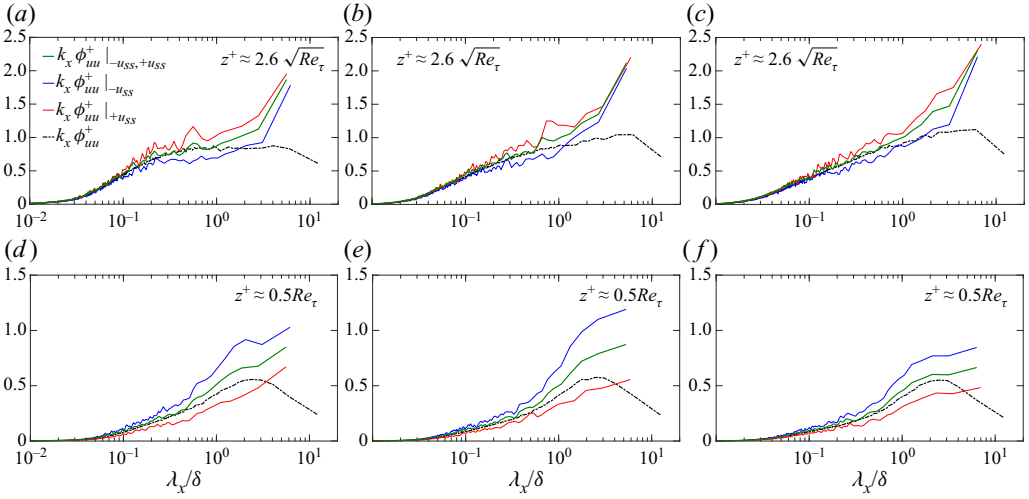
Figure 7. (a–f) Premultiplied 1-D spectra of the u -fluctuations plotted vs \lambda_x/\delta at (a–c) z^+ \approx 2.6\sqrt{Re_\tau} and (d–f) z^+ \approx 0.5Re_\tau for LFOV PIV data at Re_\tau \approx (a, d) 2500, (b, e) 5000 and (c, f) 7500. Dashed black lines correspond to the mean spectra obtained by ensembling across 3000 PIV images of the full flow field. While, the solid blue and red lines represent conditional spectra computed from the u -flow field extracted based on identification of a -u_{ss} and +u_{ss} , respectively. The spectrum in green is computed by ensembling across both -u_{ss} and +u_{ss} .
