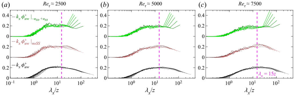
Figure 10. (a–c) Premultiplied 1-D co-spectra of the Reynolds shear stress plotted vs \lambda_x/z at various z^+ within the log region ( 2.6\sqrt{Re_\tau} \lesssim z^+ \lesssim 0.15Re_\tau ). Dashed black lines correspond to the mean spectra obtained by ensembling across 3000 PIV images of the full flow field. The spectra in green correspond to all extracted u, w -flow fields, associated with both -u_{ss} and +u_{ss} . Line plots in brown correspond to conditional spectra k_x \phi_{uw}^+|_{noSS} computed from extracted flow fields of the same length \times height as the k_x \phi_{uw}^+|_{-u_{ss}, +u_{ss}} , but not associated with the superstructures. Dashed magenta lines represent the linear scaling, \lambda_x = 15z .
