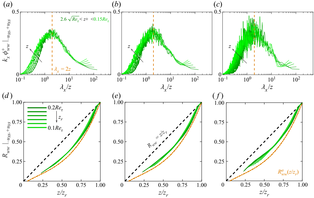
Figure 15. (a–c) Conditionally averaged premultiplied 1-D spectra of w -fluctuations plotted vs \lambda_x/z at various z^+ within the log region. (d–f) Correlation between w -fluctuations at z and z_r , normalized by \overline{w^2}(z_r) for various z_r . Here, both the spectra and the cross-correlations are computed from the extracted w -flow fields associated with -u_{ss} and +u_{ss} detected in the LFOV PIV data at Re_\tau \approx 7500 , for varying thresholds of the streamwise lengths associated with the superstructures: (a,d) L_x \gtrsim 3\delta , (b,e) L_x \gtrsim 3.8\delta and (c,f) L_x \gtrsim 4.5\delta . In (a–c), the dashed golden line represents the linear scaling, \lambda_x = 2z . In (d–f), the dashed black line corresponds to the linear relationship, z/z_r while the dash-dotted golden line corresponds to R_{ww}^a defined in (3.2).
