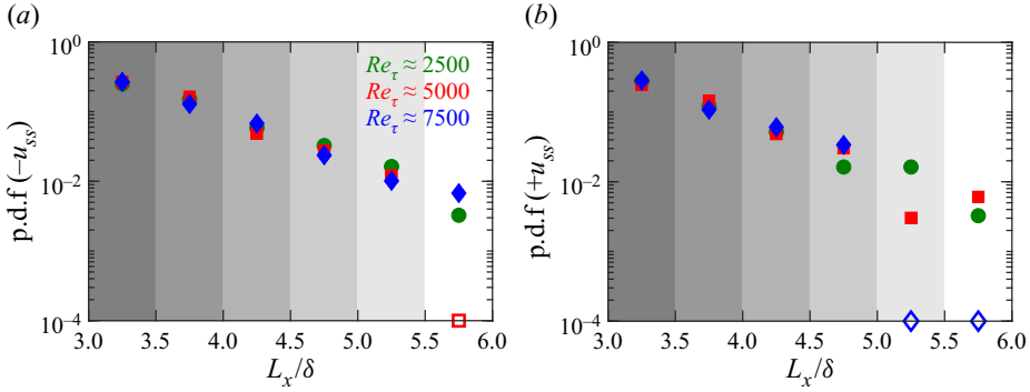
Figure 4. Probability density function (p.d.f.) of the lengths of the large and intense, (a) low and (b) high streamwise momentum motions detected by the superstructure extraction algorithm in PIV flow fields of various Re_\tau . Background shading indicates the bin sizes used to estimate the p.d.f., for which the total number of detected superstructures (i.e. addition of +u_{ss} and -u_{ss} ) was used for normalization. Empty symbols indicate zero probability for the respective bin.
