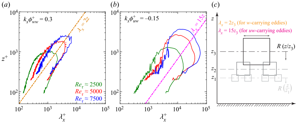
Figure 5. Iso-contours of the premultiplied streamwise 1-D (a) energy spectra of w -fluctuations and (b) co-spectra of the Reynolds shear stress plotted against z^+ and \lambda_x^+ , computed from the LFOV PIV dataset at various Re_\tau . Dash-dotted golden and magenta lines represent the relationships \lambda_x \approx 2z and \lambda_x \approx 15z , respectively following Baidya et al. (2017). (c) Schematic of representative w and uw -carrying eddies centred at various distances from the wall ( z_r ) in the log region, with light to dark shading used to suggest an increase in z_r . Here, R_{ww}(z/z_r) and R_{uw}(z/z_r) respectively represent the vertical coherence of the w - and uw -carrying eddies centred at z_r .
