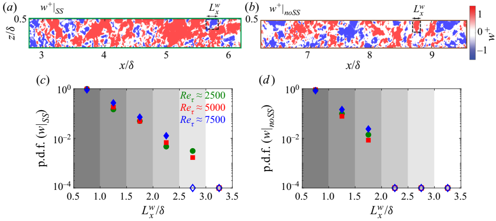
Figure 12. (a,b) Examples of intense w -fluctuations ( |w_{SS}|, |w_{noSS}| > 1.3\sqrt{w^2(z)} ) present within flow fields associated (a) with superstructures ( w|_{SS} ) and (b) not associated with superstructures ( w|_{noSS} ). The w|_{SS} and w|_{noSS} flow fields used as examples in (a,b) essentially correspond to the extracted fields shown in figure 3(e,g). (c,d) Probability density function (p.d.f.) of the lengths ( L_x^w ) of intense (c) w|_{SS} and (d) w|_{noSS} motions extracted from the corresponding flow fields at various Re_\tau . Background shading indicates the bin size used to estimate the p.d.f., for which the total number of detected w|_{SS} and w|_{noSS} were used for normalization. Empty symbols indicate zero probability for the respective bin.
