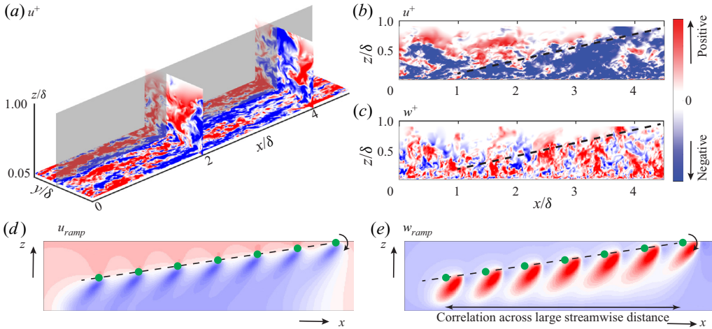
Figure 2. Colour contours of the instantaneous (a,b) streamwise, u and (c) wall-normal velocity fluctuations, w , in a boundary layer at Re_\tau \approx 2000 . These data have been extracted from a particular three-dimensional (3-D) time block of the publicly available DNS dataset of Sillero, Jiménez & Moser (2013). In (a), u is plotted on a wall-parallel plane at z \approx 0.05\delta , as well as on the cross-planes at x \approx 2\delta and 4\delta . Panels (b) and (c) respectively plot the u and w fluctuations in the streamwise wall-normal plane shaded in grey in (a). Dashed black line in (b,c) traces the top part of a long -u ramp type structure. Panels (d,e) respectively plot an idealized distribution of u and w flow field induced by multiple prograde vortices (in green) positioned along the ramp (Adrian et al. 2000; de Silva et al. 2016).
