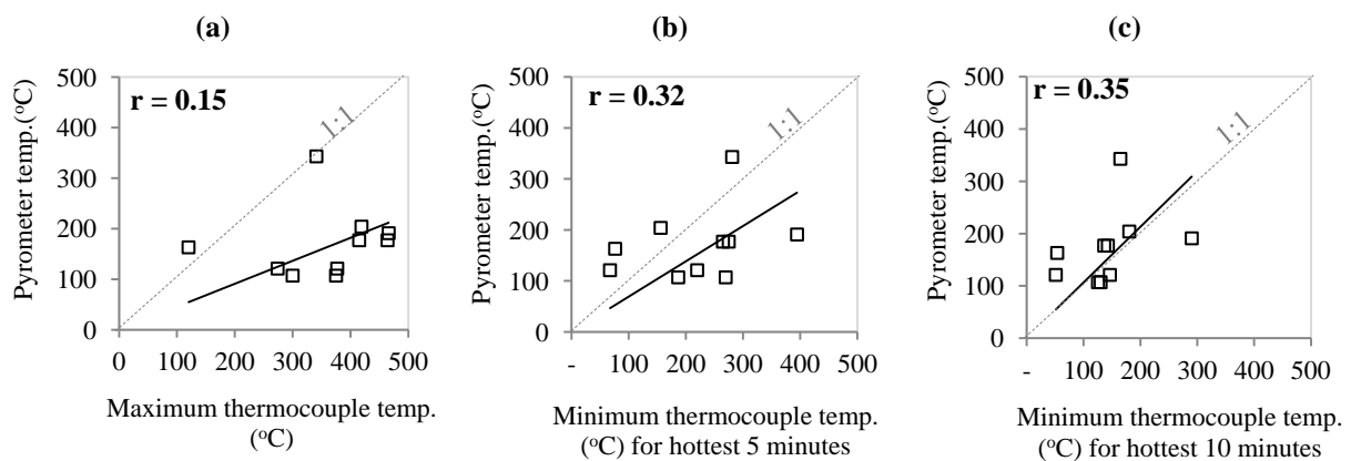
Figure 22: Pyrometer temperatures versus (a) maximum thermocouple temperatures, (b) minimum thermocouple temperatures for hottest five minutes and (c) minimum thermocouple temperature for hottest 10 minutes. Data are for paired pyrometers and thermocouples (spaced within 100 mm horizontally of each other) on the soil surface at Mt Cole.
