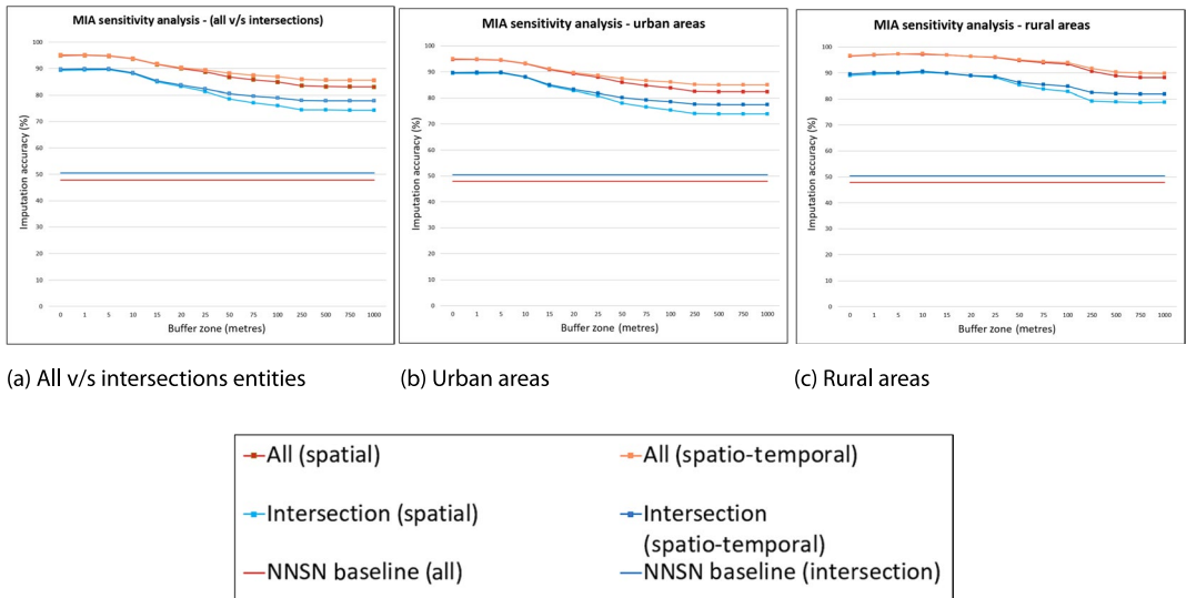
FIGURE 14 MIA sensitivity analysis, all environments, urban, and rural
