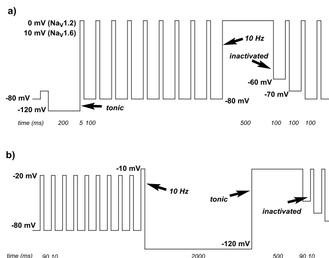
Figure 3. Patch clamp voltage protocols. a) Protocol 1 used for assessing state dependence of Na v 1.2 and 1.6 channels. The test-pulse potential was 0 mV for Na v 1.2; 10 mV for Na v 1.6. b) Protocol 2 allows assessment of contribution of binding to slow inactivated channels.
