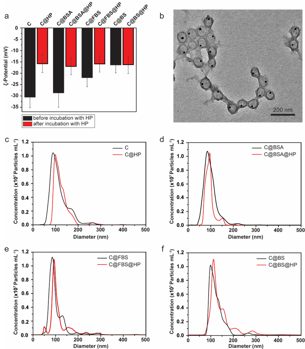
Figure 2. (a) \zeta -potential of the uncoated nanocapsules (C), and BSA-, FBS-, and BS-precoated Au@MPN nanocapsules before (C@BSA, C@FBS, and C@BS) and after (C@HP, C@BSA@HP, C@FBS@HP, and C@BS@HP) incubating for 1 h with HP. Data are shown as the mean \pm standard deviation (SD) of three independent measurements. (b) TEM image of the Au@MPN nanocapsules after incubating for 1 h with HP (C@HP). (c–f) Size distribution of the uncoated and precoated Au@MPN nanocapsules before (C, C@BSA, C@FBS, and C@BS) and after (C@HP, C@BSA@HP, C@FBS@HP, and C@BS@HP) incubating with HP, as determined by NTA.
