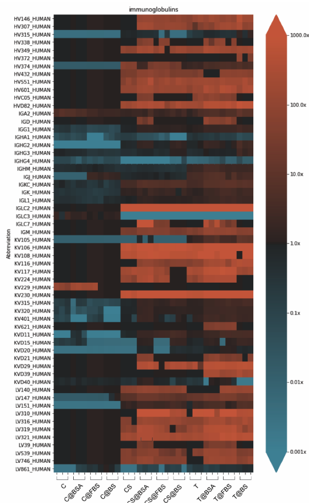
Figure 6. Heatmap of the differential enrichment of immunoglobulins in the biomolecular coronas of the Au@BDT templates (T, T@BSA, T@FBS, and T@BS), Au@BDT@MPN core–shell nanoparticles (CS, CS@BSA, CS@FBS, and CS@BS), and Au@MPN nanocapsules (C, C@BSA, C@FBS, and C@BS) without and with precoating. The proteins are listed alphabetically in a colorized log scale. Three replicates of each nanoparticle system were examined.
