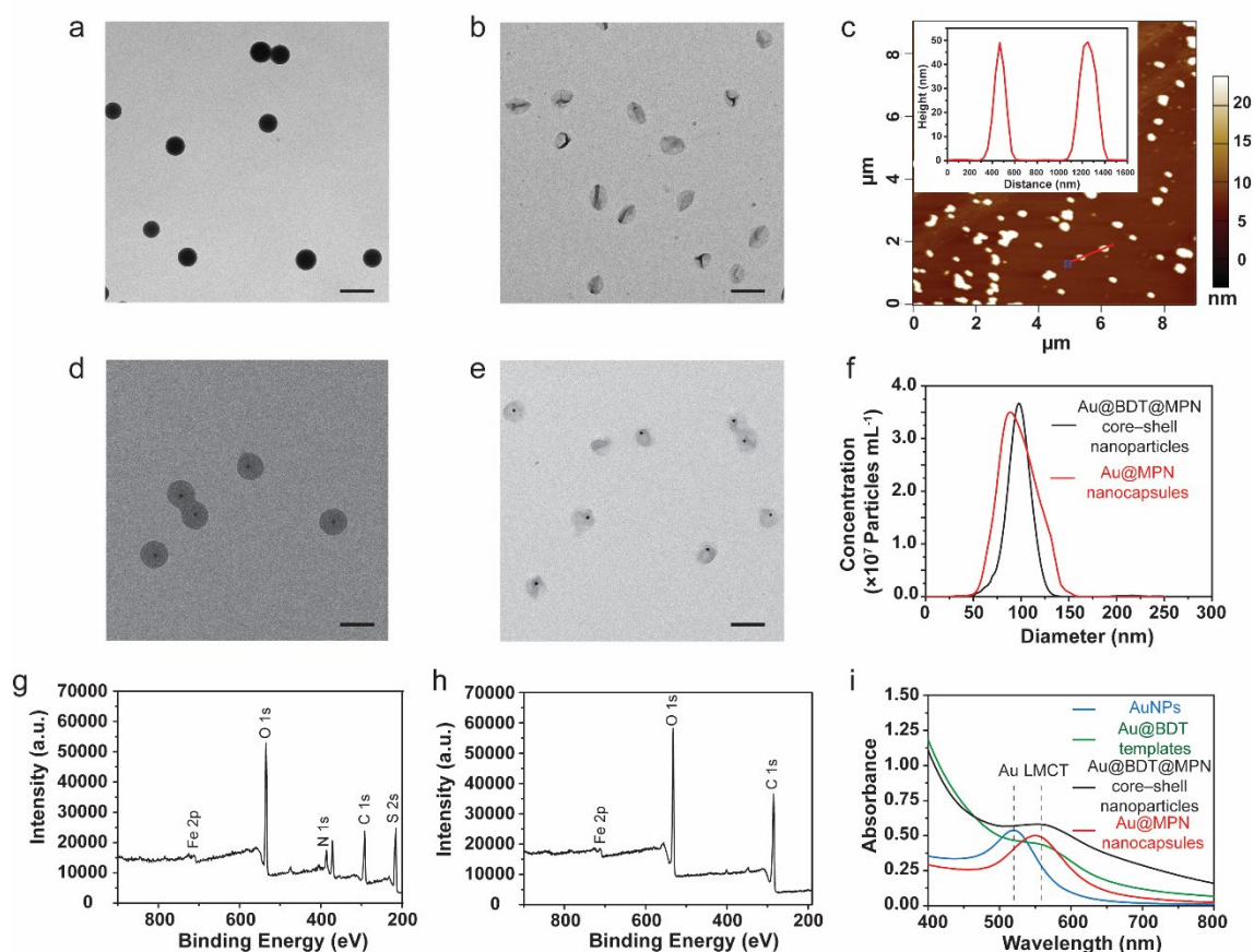
Figure 1. (a,b) TEM images of 100 nm BDT@MPN core-shell nanoparticles (a) and 100 nm MPN nanocapsules (b); scale bars are 200 nm. (c) AFM measurements of 100 nm MPN nanocapsules. (d,e) TEM images of 100 nm Au@BDT@MPN core-shell nanoparticles (d) and 100 nm Au@MPN nanocapsules (e). (f) Size distribution of Au@BDT@MPN core-shell nanoparticles and Au@MPN nanocapsules determined by NTA. (g,h) XPS patterns of 100 nm BDT@MPN core-shell nanoparticles (g) and MPN nanocapsules (h). (i) UV-vis absorption spectra of AuNPs, and 100 nm Au@BDT templates, Au@BDT@MPN core-shell nanoparticles, and Au@MPN nanocapsules dispersed in water.
