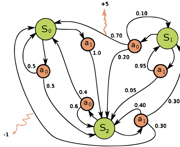
FIGURE 2.1: An example of an MDP with three states (green circles), two actions (orange circles), and two rewards (orange arrows) by Waldoalvarez , licensed under CC BY-SA 4.0 .
