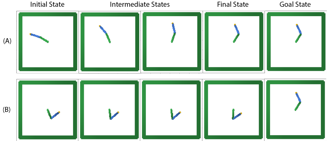
FIGURE 4.8: An example of policy execution for the latent space with the action regularisation and the state-similarity reward function. (A) - the angle of the bottom joint differs less than 90^\circ from the goal state. (B) - the angle of the bottom joint differs more than 90^\circ from the goal state.
