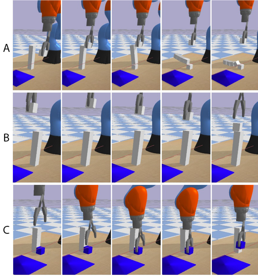
FIGURE 3.8: (A) A demo showing the policy execution of sens, absolute on place 4 on 5 with \lambda = 0 . (B) A demo showing the policy execution of sens, relative on place 4 on 5 with \lambda = 0 . (C) A demo showing sens policy execution in the task pick 3 on 4 with \lambda = 0 .
