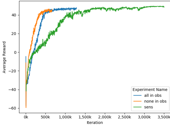
FIGURE 3.9: The cumulative rewards for the 'Pick' task with \lambda = 0 .
