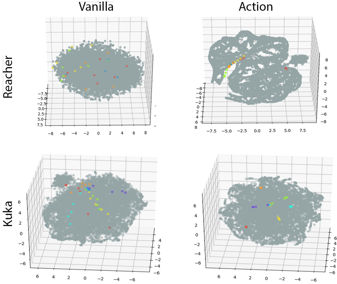
FIGURE 4.5: A visual representation of the vanilla and action regularised latent spaces. The spaces are reduced from 256 dimensions by t-SNE, where the colours represent distinct unit actions. The blue dots are the same initial state.
