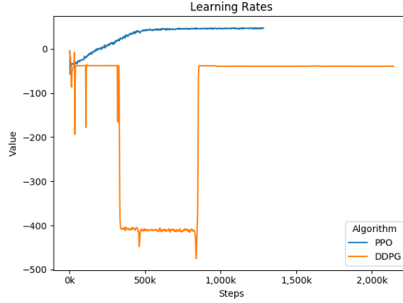
FIGURE 3.5: PPO vs DDPG performance. The cummulative rewards for 'Pick' task.
