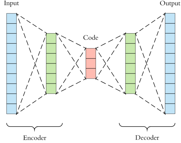
FIGURE 2.3: The structure of an autoencoder.
