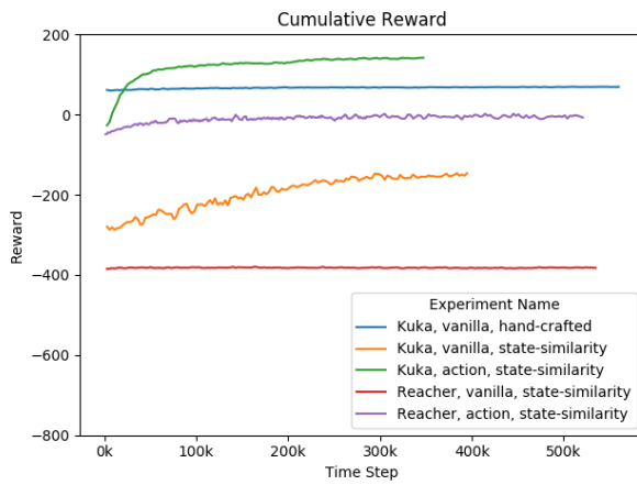
FIGURE 4.6: The cumulative reward for the Kuka and Reacher environments
