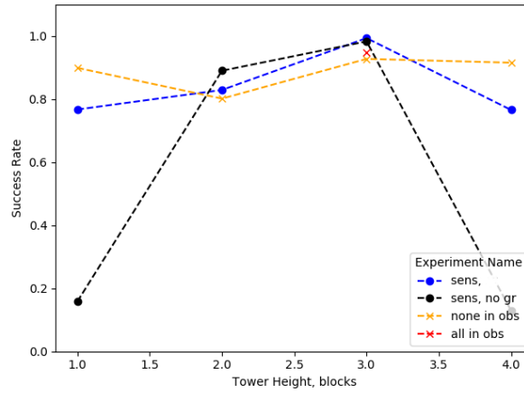
FIGURE 3.10: The experimental results for the task of picking a goal block adjacent to a tower. In this experiment, we treated a trial as successful if the agent had picked the block regardless the state of the tower. The experiment names represent different observation spaces. The notations are: none in obs - no blocks in observations; all in obs - all the blocks in observations; sens - a sensing sphere; no gr - no gripper coordinates in the observations. We used \lambda = 0 in the reward function.
