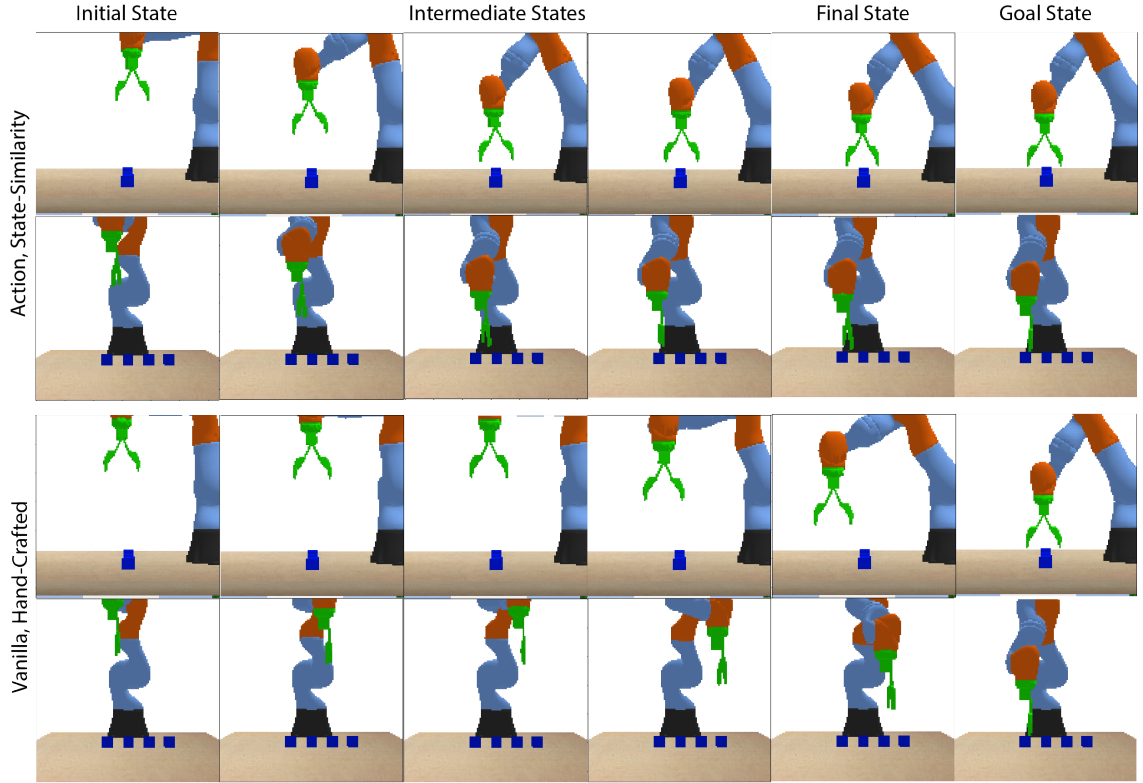
FIGURE 4.7: An example of policy execution for the latent space with the action regularisation and the state-similarity reward function (at the top), and the latent space with the vanilla regularisation and the hand-crafted reward function (at the bottom). The final state is the last state of the trial. The policy were executed for the ball radius of four blocks.
