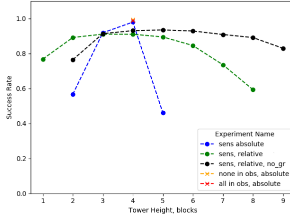
FIGURE 3.7: The experimental results for the task of placing a goal block on the top of a tower. The experiment names represent different observation spaces. The notations are: none in obs - no blocks in observations; all in obs - all the blocks in observations; sens - a sensing sphere; absolute - a subtask with the gripper’s absolute initial configuration; relative - a subtask with the gripper’s relative initial configuration; no gr - no gripper coordinates in the observations.
