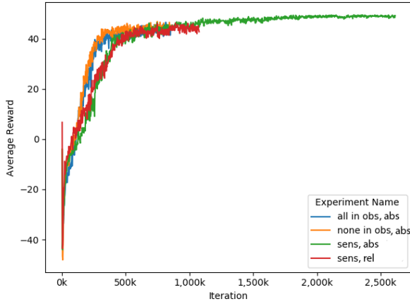
FIGURE 3.6: The cumulative reward for the 'Place' task with \lambda = 0 .
