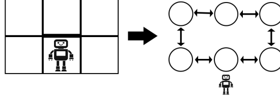
FIGURE 4.1: An example of a state space \mathcal{S} (to the right) modelling the environment to the left, where the further the physical distance to a state (a circle), the further distance in the environment.
