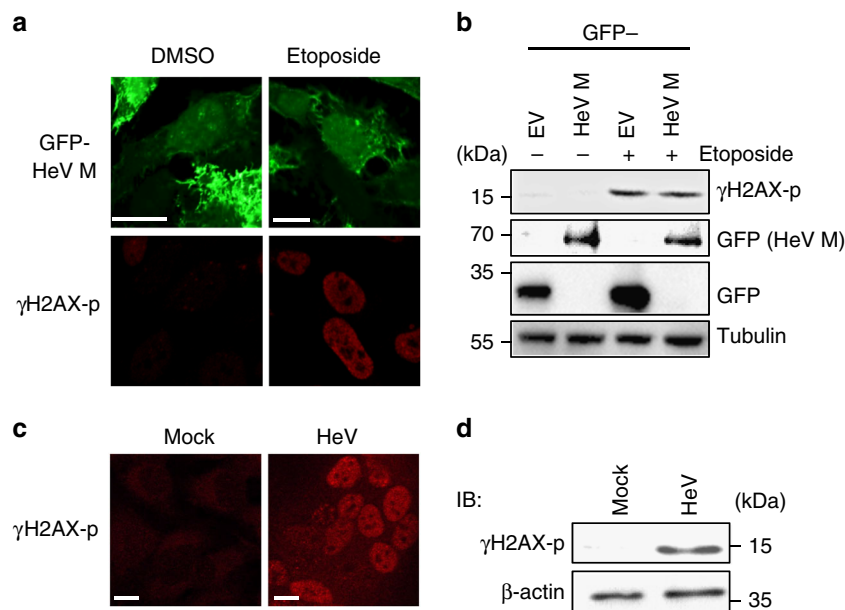
Fig. 8 HeV infection but not HeV M protein expression induces DNA damage. a HeLa cells transfected to express GFP-HeV M protein without (DMSO) or with etoposide treatment were fixed 16 h p.t., immunostained for \gamma H2AX phosphorylated at S139 ( \gamma H2AX-p) and imaged by CLSM. Images are representative of \geq 15 fields of view. b Lysates of HEK-293T cells transfected to express GFP alone (empty vector (EV)) or GFP-HeV M protein and treated at 16 h p.t. without or with etoposide (3 h), were analyzed by IB using the indicated antibodies (data are representative of two independent experiments). c HeLa cells infected with HeV (MOI 5; which results in c. 100% cells infected) were fixed 24 h p.i. and immunostained for \gamma H2AX-p prior to imaging by CLSM (images representative of \geq 15 fields of view from three biological replicates). d Lysates of mock or HeV-infected HeLa cells were collected at 24 h p.i. and analyzed by IB using the indicated antibodies (data representative of three biological replicates). Scale bars correspond to 15 \mu m
