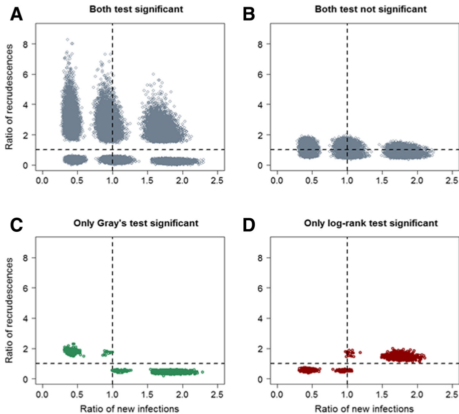
Fig. 6 Ratio of recrudescence and new infection in simulation study II ( n = 500 subjects/arm). The ratio of recrudescence for drug B relative to drug A plotted against the ratio of new infection for drug B relative to drug A for 1000 simulated dataset
