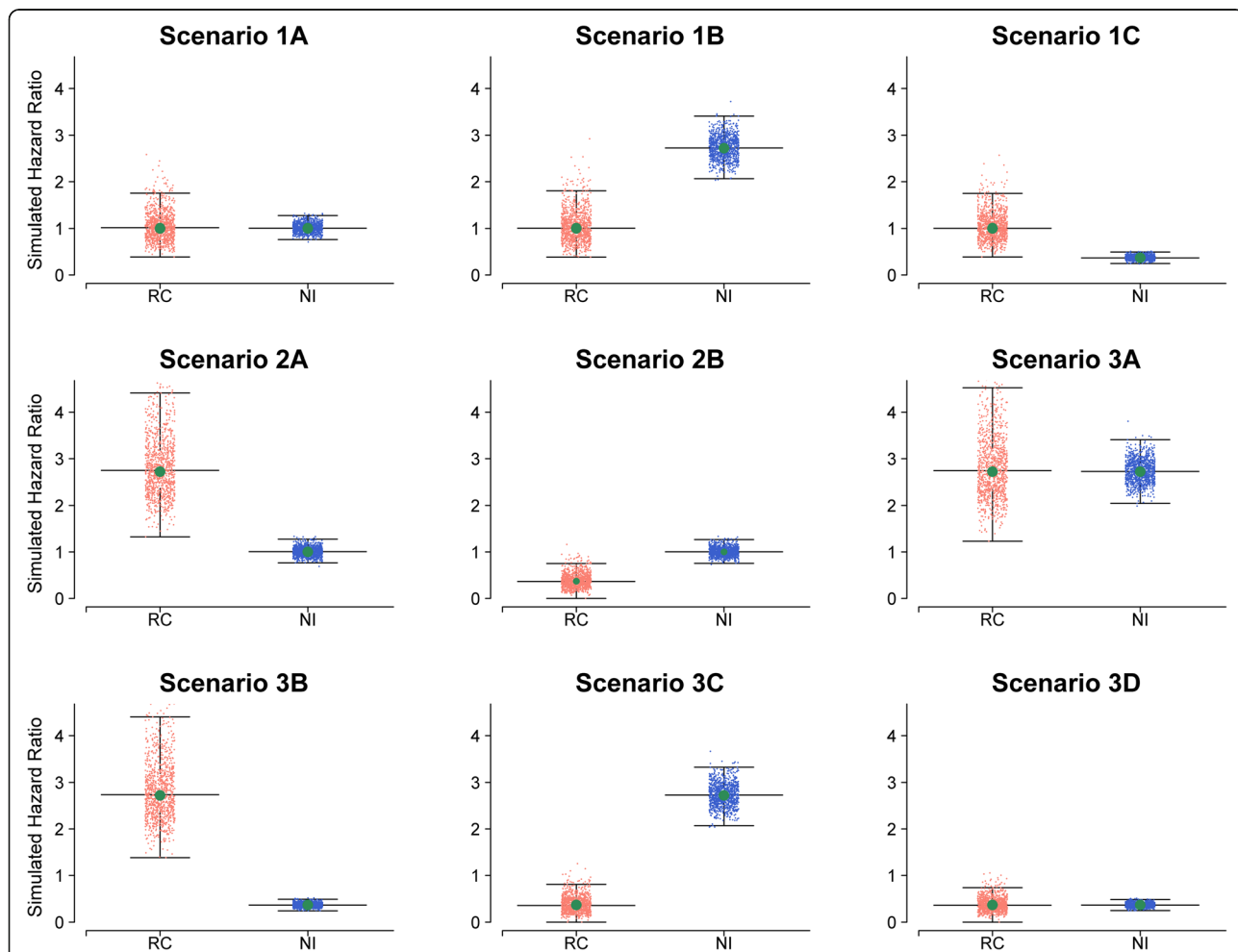
Fig. 5 Distribution of simulated hazard ratio ( n = 500 subjects) in simulation study II. The scatterplot of estimated hazards ratio for recrudescence and new infection for drug B relative to drug A from 1000 simulation runs. The median and interquartile range is shown. The centre green dot depicts the true hazard ratio which was used to simulate the respective datasets (1, 2.72 or 0.37). RC = recrudescence, NI = New infection. The description of each of the individual scenario is provided in Table 1
