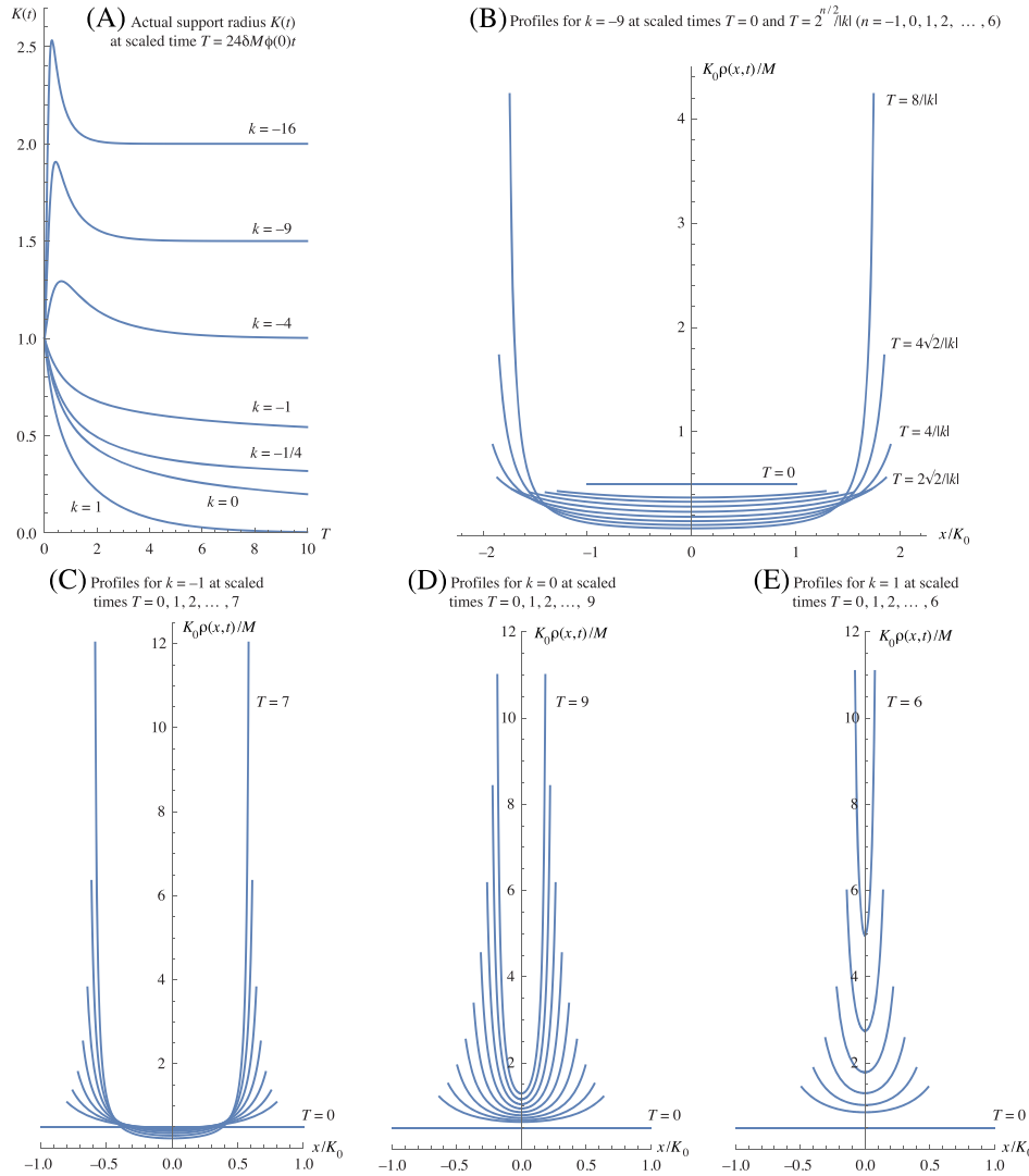
FIGURE 8 Evolution from the compact initial profile (84). (A) Actual support radius K(t) for seven values of k : horizontal asymptotes for k < 0 cases (top five curves) are the minimum equilibrium Dirac position \sqrt{|k|}/2 . (B-E) Scaled mass distribution K_0\rho(x, t)/M as a function of scaled position x/K_0 at times shown [Colour figure can be viewed at wileyonlinelibrary.com ]
