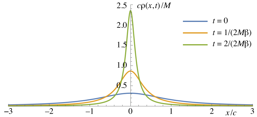
FIGURE 1 Collapse of the initial mass distribution \rho(x, 0) = Mc/[\pi(x^2 + c^2)] under the attractive potential W(x) = \beta x^2 . Horizontal axis is x/c ; vertical axis is c\rho(x, t)/M . Times are t = 0 (blue—the curve with the lowest peak), t = 1/(2M\beta) (brown) and t = 2/(2M\beta) (green—the curve with the highest peak) [Colour figure can be viewed at wileyonlinelibrary.com ]
