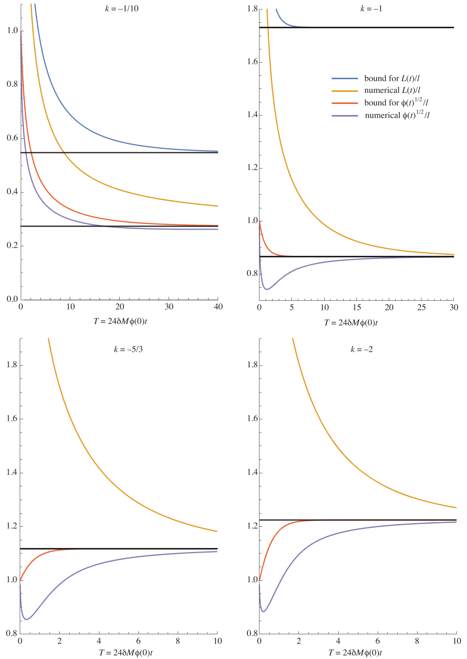
FIGURE 4 For the unbounded support initial distribution (84) with a repulsive quadratic potential component, we show in colour (ordered top to bottom) the upper bound (69) for the maximum support radius L(t) (off scale for k < -1 ), L(t) itself, the upper bound (70) for the root-mean-square spread \sqrt{\phi(t)} , and \sqrt{\phi(t)} itself. We also show (black lines) bounds (71) on the allowed equilibrium Dirac distance \xi from the origin. For k \leq -4/3 , the upper bound (70) and the lower bound for \xi coincide [Colour figure can be viewed at wileyonlinelibrary.com ]
