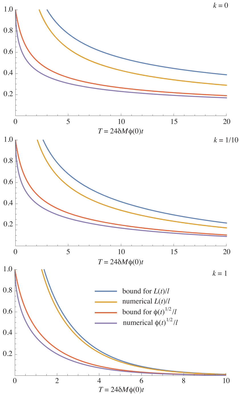
FIGURE 3 For the unbounded support initial distribution (84) when the quadratic term in the potential is non-negative (ie, purely attractive potential), we show four curves, listed here ordered from top to bottom: the upper bound (69) for the maximum support radius L(t) , L(t) itself, the upper bound (70) for the root-mean-square spread \sqrt{\phi(t)} , and \sqrt{\phi(t)} itself. For k > 1 , the top two curves become increasingly difficult to distinguish as k increases, as do the lower two curves [Colour figure can be viewed at wileyonlinelibrary.com ]
