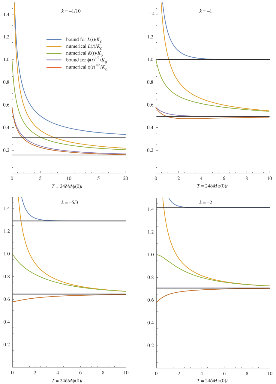
FIGURE 7 For the compact support initial distribution (84) in the case when the quadratic term in the potential is negative (a repulsive quadratic potential component), we show the following five curves, listed here ordered from top to bottom: the upper bound (94) for the maximum support radius L(t) , L(t) itself, the actual support radius K(t) , the upper bound (95) for the root-mean-square spread \sqrt{\phi(t)} , and \sqrt{\phi(t)} itself. We also show (black lines) bounds on the allowed equilibrium Dirac locations. For k \leq -4/3 , the upper bound (70) and the lower bound for \xi coincide [Colour figure can be viewed at wileyonlinelibrary.com ]
