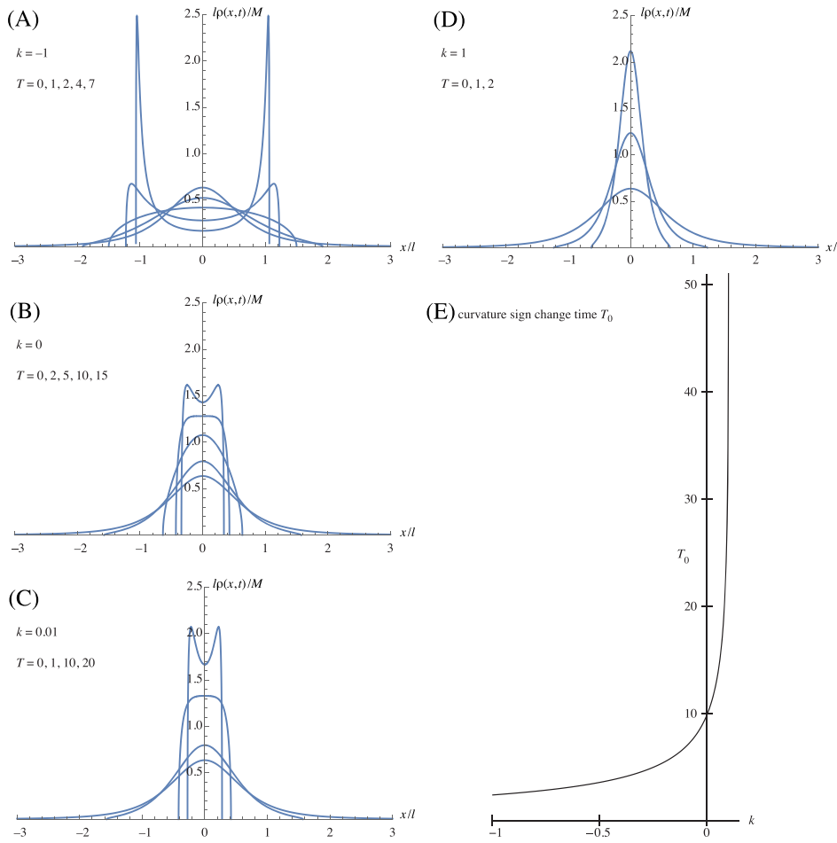
FIGURE 5 (A-D) The evolution of the scaled mass profile \ell\rho(x, t)/M with time for k \in \{-1, 0, 0.01, 1\} . For k = 1 , numerical solutions do not show a change in change in the sign of the curvature at the origin for T \leq 1000 , and if a sign change were to occur, the corresponding T would be enormous. (E) The time at which the curvature changes for -1 \leq k \leq 0.1012 . The curve becomes increasingly steep, and for k = 0.101781 , the sign change occurs for T \approx 1859.36 [Colour figure can be viewed at wileyonlinelibrary.com ]
