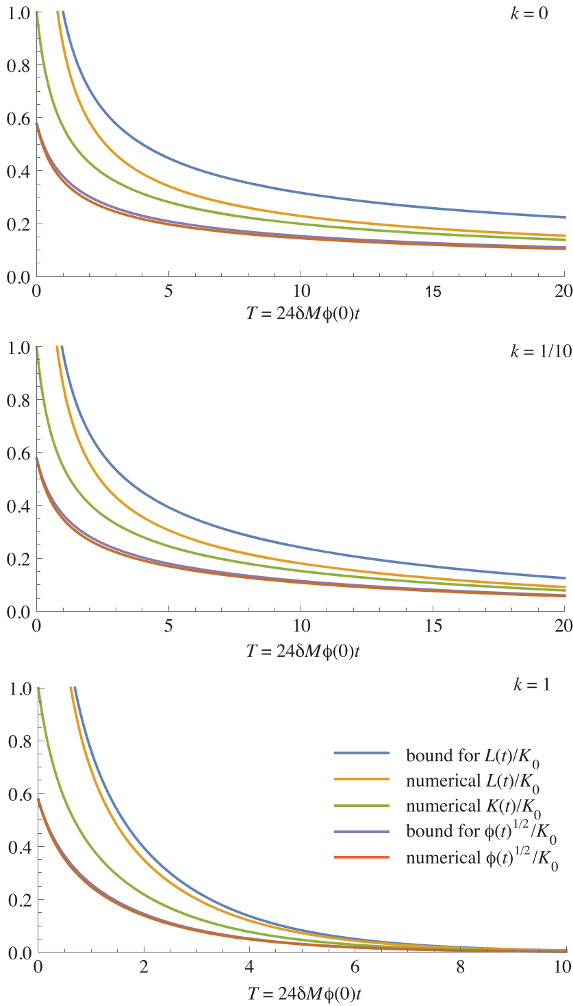
FIGURE 6 For the compact support initial distribution (84) when the quadratic term in the potential is non-negative (ie, purely attractive potential), we show in colour, ordered from top to bottom, the upper bound (94) for the maximum support radius L(t) , L(t) itself, the actual support radius K(t) , the upper bound (95) for the root-mean-square spread \sqrt{\phi(t)} , and \sqrt{\phi(t)} itself. For k > 1 , the top two curves become increasingly difficult to distinguish as k increases, as do the lower two curves [Colour figure can be viewed at wileyonlinelibrary.com ]
