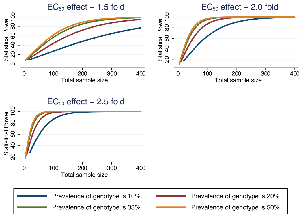
Figure 2. Statistical power by sample size for a comparison of EC_{50} (geometric mean) between two genotypes. doi:10.1371/journal.pone.0069505.g002
