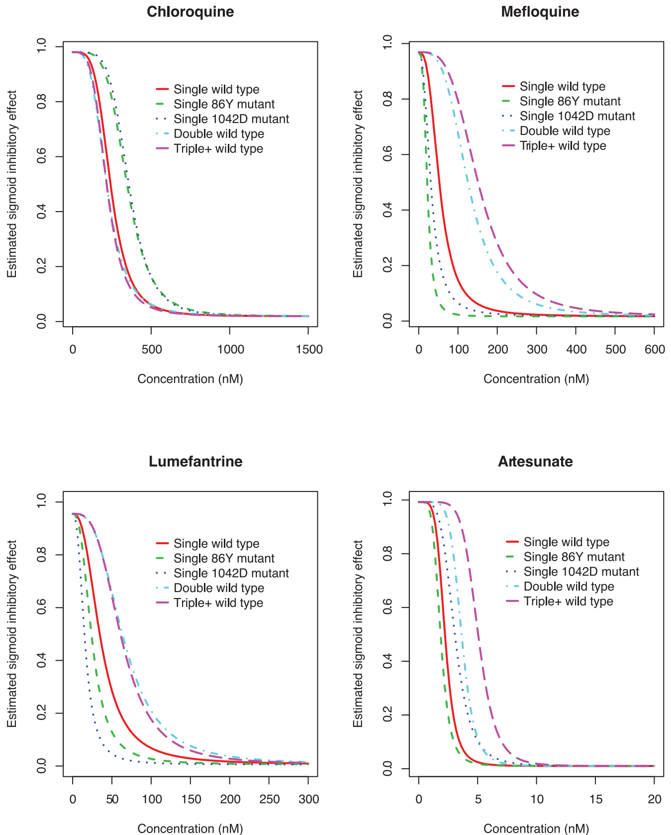
Figure 1. Estimated concentration-effect relationship (via nonlinear mixed-effects modelling) for chloroquine, mefloquine, lumefantrine and artesunate, by genotype grouping. doi:10.1371/journal.pone.0069505.g001
