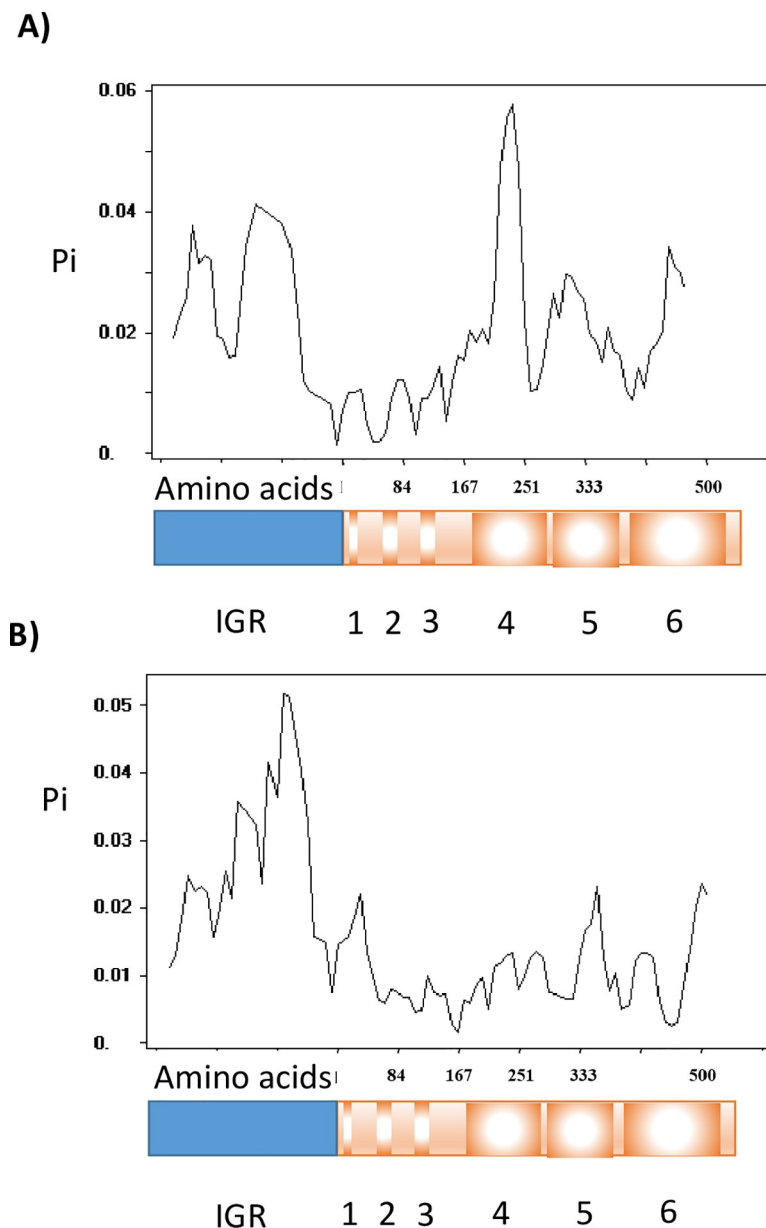
Fig 5. Observed nucleotide diversity ( \pi ) distribution within the intergenic region and functional domains of A) mga-1 ( n = 151 ) and B) mga-2 ( n = 793 ). IGR = intergenic region, 1 = Common Mga domain, 2 = helix-turn-helix (HTH)-3, 3 = HTH-4, 4 = phosphotransferase system regulatory domain (PRD)-1, 5 = PRD-2, 6 = phosphotransferase system enzyme IIB-like domain.
