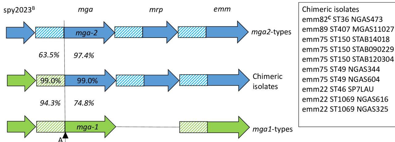
Fig 1. Schematic representation of the recombination event observed in the intergenic region of mga suggesting recombination of mga-2 into an mga-1 -type background ( n = 10 ). Numerical values represent both the intra-allele and inter-allele percentage nucleotide identities. Hatched fill = Intergenic regions, Blue = genes of mga-2 -type isolates, and Green = genes of mga-1 -type isolates. Notes A = recombination flank, B = SF370 spy locus tag, C = emm82 C chimeric emm gene.
