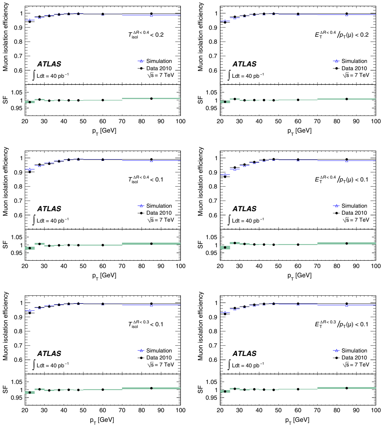
Fig. 14 Isolation efficiencies for muons from Z decays as a function of p_T , for track isolation (left) and calorimeter isolation (right) requirements with different isolation cone radii, \Delta R , as described in the legend.
