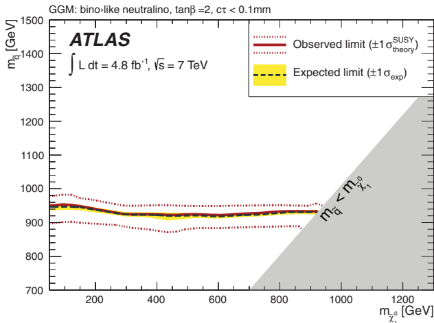
Figure 7: Expected and observed 95% CL lower limits on the squark mass as a function of the neutralino mass in the GGM model with a bino-like lightest neutralino NLSP (the grey area indicates the region for which the squark mass is less than the bino mass, which is not considered here). The other sparticle masses are assumed to be decoupled. Further model parameters are \tan\beta = 2 and c\tau_{\text{NLSP}} < 0.1 mm.
