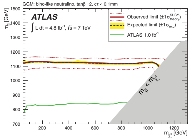
Figure 6: Expected and observed 95 % CL lower limits on the gluino mass as a function of the neutralino mass in the GGM model with a bino-like lightest neutralino NLSP (the grey area indicates the region for which the gluino mass is less than the bino mass, which is not considered here). The other sparticle masses are assumed to be decoupled. Further model parameters are \tan\beta = 2 and c\tau_{\text{NLSP}} < 0.1 mm. The previous ATLAS limit [1] is also shown.
