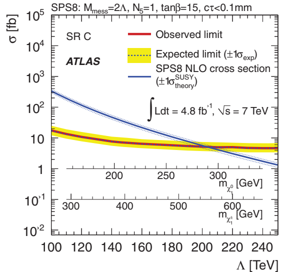
Figure 8: Expected and observed 95% CL upper limits on the sparticle production cross section in the SPS8 model, and the NLO cross-section prediction, as a function of \Lambda and the lightest neutralino and chargino masses. Further SPS8 model parameters are M_{\text{mess}} = 2\Lambda , N_5 = 1 , \tan\beta = 15 and c\tau_{\text{NLSP}} < 0.1 mm. Limits are set based on SR C.
