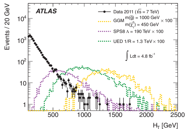
Figure 3: The H_T spectrum of \gamma\gamma candidate events in the data (points, statistical uncertainty only) together with the spectra from simulated GGM ( m_{\tilde{g}} = 1000 GeV, m_{\tilde{\chi}_1^0} = 450 GeV), SPS8 ( \Lambda = 190 TeV), and UED ( 1/R = 1.3 TeV) samples after the diphoton requirement. The signal samples are scaled by a factor of 100 for clarity.
