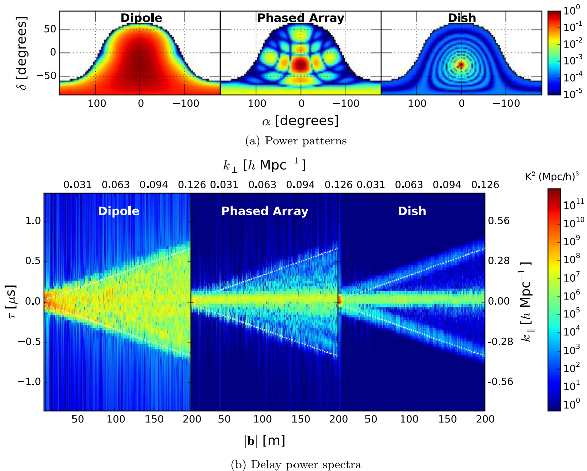
Figure 4. Power patterns (top panels) and simulated delay power spectra (bottom panels) for different antenna shapes at 185 MHz centered on zenith. Antenna shapes used are: dipole (left), phased array (middle), and dish (right). Refer to Section 4.1 for details of the antenna models. The strength and occupancy of the power patterns are correlated with those of delay power spectra. White dotted lines in the delay power spectra mark the boundaries of the foreground wedge determined by the horizon delay limit and antenna spacing. The foreground wedge and the EoR window are most severely contaminated in the case of the dipole while it is the least for the dish. The phased array has intermediate levels of contamination. Foreground power close to the horizon delay limits in all three cases is significant even on long baselines. The foreshortening of baselines toward the horizon makes them sensitive to foreground emission on large size scales. The amplitude of this feature strongly depends on the shape of the antenna element. It is highest for a dipole (which has a strong response near the horizon) and least for a dish.
