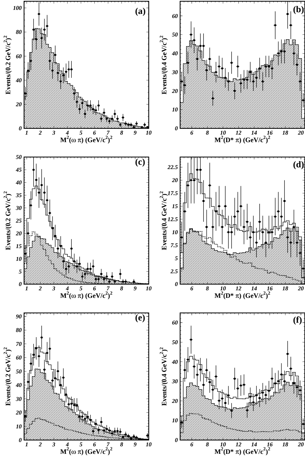
Figure 7: M^2(\omega \pi) and M^2(D^* \pi) distributions of the \bar{B}^0 \rightarrow D^{*+} \omega \pi^- candidates in the (\Delta E, M(\pi^+ \pi^- \pi^0)) sideband regions (a,b) IV, (c,d) III and (e,f) II. Points with error bars are data; hatched histograms correspond to the contribution from B_{IV}(\vec{x}) ; dotted histograms represent the component described by the function B_{III}(\vec{x}) in (c) and (d) and B_{II}(\vec{x}) in (e) and (f); open histograms correspond to the total fit results in Regions III and II.
