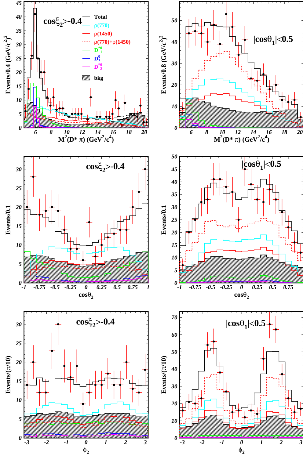
Figure 13: (color online). Distribution of three D^* \pi variables for D^{*+} \omega \pi^- candidates in two different subregions of the signal region (points with error bars), defined by \cos \xi_2 > -0.4 ( D^{**} enriched) and |\cos \theta_1| < 0.5 ( D^{**} depleted). The histograms represent the results of the fit (black), including the following components: \rho(770) (cyan), \rho(1450) (red), \rho(770) and \rho(1450) together (red dashed), D_1(2430)^0 (green), D_1(2420)^0 (blue), D_2^*(2460)^0 (magenta) and background (hatched).
