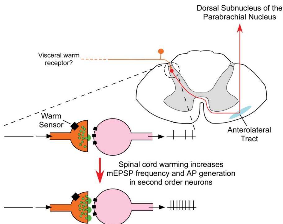
Figure 2. Spinal warm sensing. Diagram showing suggested mechanism whereby spinal warming generates action potentials in the secondary neurons of unidentified, possibly visceral, warm-sensing pathways. Abbreviations: mEPSP, miniature excitatory postsynaptic potential; AP, action potential.
