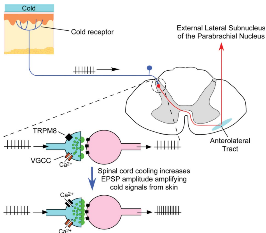
Figure 1. Spinal cold sensing. Diagram showing suggested mechanism whereby spinal cooling enhances neurotransmission at the first synapse of the cold afferent pathway, and spinal warming attenuates transmission. Abbreviations: TRPM8, transient receptor potential ion channel M8; VGCC, voltage-gated calcium channel; EPSP, excitatory postsynaptic potential.
