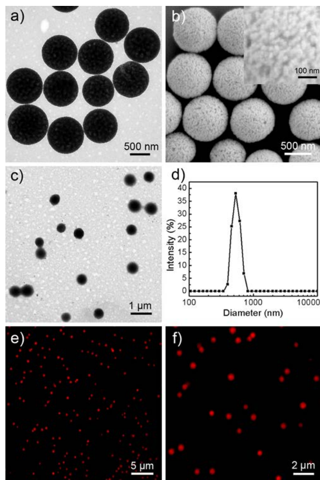
Figure 1. a) TEM and b) SEM images of MS particles. The inset in b) is a higher-magnification image of the surface of a MS particle. c) TEM image, d) size distribution, and e,f) CLSM images of PMA SH -Dox particles after removal of the MS spheres.
