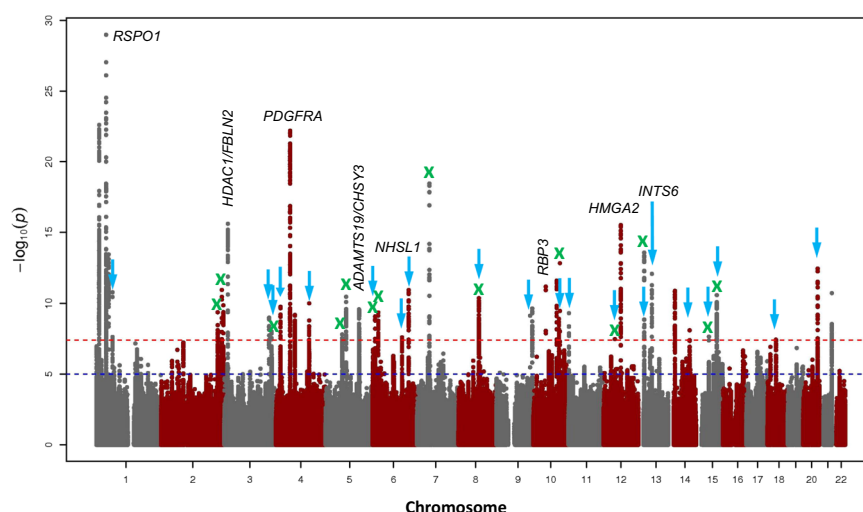
Fig. 1 Manhattan plot of trans-ethnic GWAS meta-analysis for corneal curvature. Both directly genotyped and imputed variants were meta-analysed for corneal curvature in 44,042 CREAM participants. The y-axis represents -\log_{10}P values for association with corneal curvature, and the x-axis represents genomic position based on human genome build 37, highlighting newly identified loci (arrows in blue; Table 1), loci associated with axial length (labelled with nearest gene names), and loci associated with spherical equivalent (cross in green). The horizontal red line indicates the genome-wide significance level of P < 5.0 \times 10^{-8} . The horizontal blue line indicates the suggestive significance level of P < 1.0 \times 10^{-5} .
