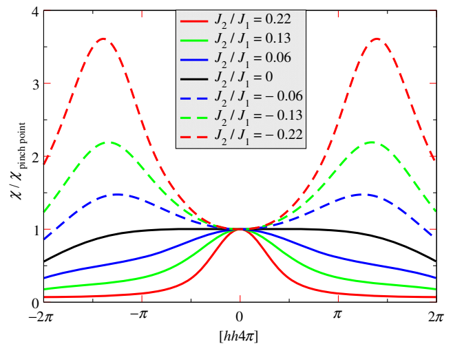
FIG. 20. For the S = 1/2 J_1 - J_2 model, the susceptibility plotted along the [hh4\pi] cut (white line in Fig. 18) evaluated at T/J = 1/100 for different J_2 .
