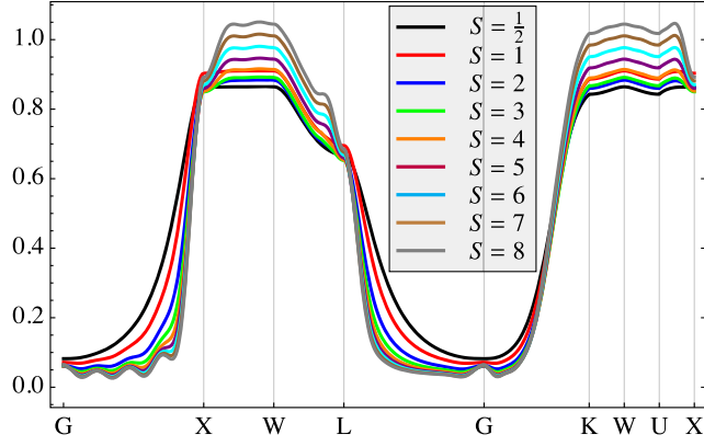
FIG. 14. The susceptibility of the isotropic nearest-neighbor Heisenberg antiferromagnet plotted along the high-symmetry path evaluated at the lowest simulated temperature ( T/J_1 = 1/100 ) for S = 1/2 and S = 1 and at the critical breakdown temperature ( T_c ) (marked by arrows) in the RG flows in Fig. 13 for S > 1 .
