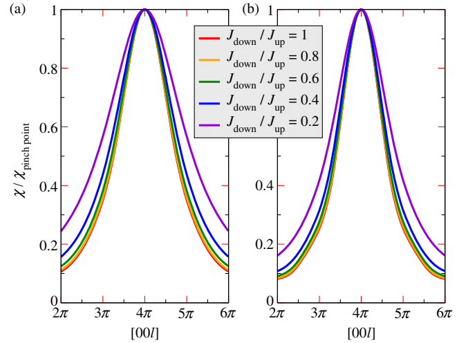
FIG. 12. For the breathing nearest-neighbor Heisenberg antiferromagnet, we plot the susceptibility along the 1D cut (see the white line in the T/J_1 = 1/100 panel in Fig. 6) at the lowest simulated temperature T/J_1 = 1/100 for (a) S = 1/2 and (b) S = 1 .
