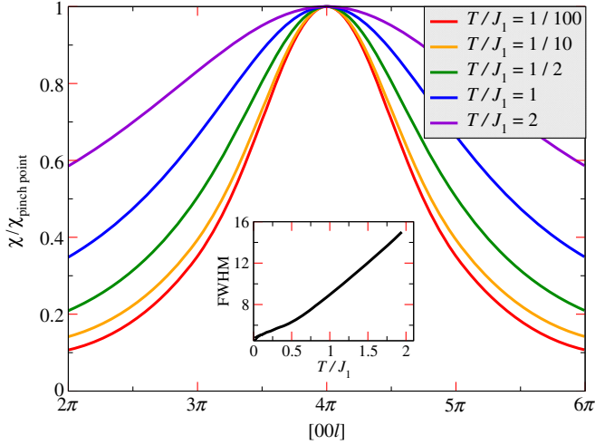
FIG. 8. The susceptibility of the S = 1/2 isotropic nearest-neighbor Heisenberg antiferromagnet plotted along the 1D cut (see the white line in the T/J_1 = 1/100 plot in Fig. 6) across the bow-tie width at different temperatures. The inset shows the FWHM of the curves as a function of the temperature.
