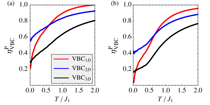
FIG. 9. The RG flows of the dimer response functions \eta_{\text{VBC}}^p [Eq. (15)] of different valence-bond crystals for (a) S = 1/2 and (b) S = 1 isotropic nearest-neighbor Heisenberg antiferromagnets.
