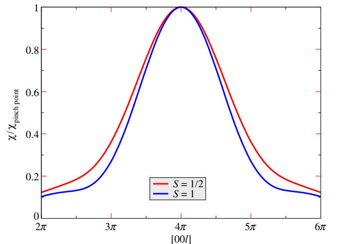
FIG. 7. The susceptibilities of the S = 1/2 and S = 1 isotropic nearest-neighbor Heisenberg antiferromagnet plotted along the 1D cut (see the white line in the T/J_1 = 1/100 plot in Fig. 6) across the bow-tie width at the lowest simulated temperature T/J_1 = 1/100 .
