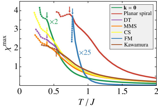
FIG. 21. RG flows of the spin susceptibility for S = 1/2 at the ordering wave vectors of the seven magnetically ordered phases evaluated at the data points marked by black disks in Fig. 16(a). The points at which the solid lines become dashed (marked by arrows) indicate an instability in the flow, indicating an onset of magnetic order.
