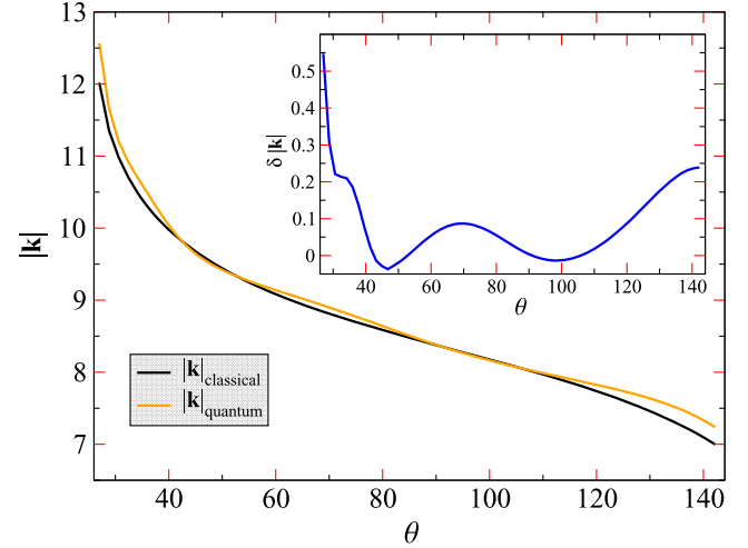
FIG. 22. The behavior of the classical |\mathbf{k}_{\text{cl}}| and quantum |\mathbf{k}_{\text{qu}}| ordering wave vectors as a function of \theta = \arctan(J_2/J_1) . Inset: Deviation |\delta\mathbf{k}| = |\mathbf{k}_{\text{qu}}| - |\mathbf{k}_{\text{cl}}| of the ordering wave vector \mathbf{k} from its classical value as a function of \theta .
