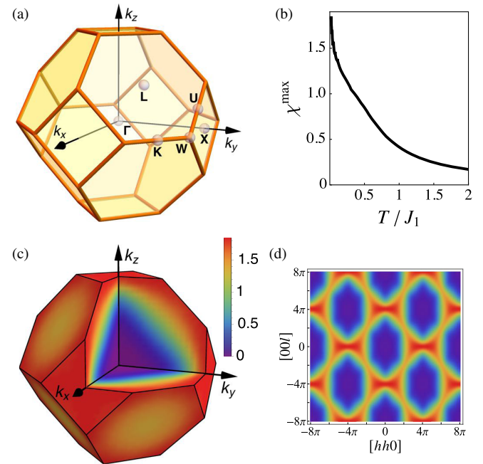
FIG. 5. (a) The EBZ (a truncated octahedron) of the pyrochlore lattice labeled with the high-symmetry points. (b)–(d) For the S = 1/2 isotropic nearest-neighbor Heisenberg antiferromagnet, the RG flow of the susceptibility evaluated at the W point (b), the \mathbf{k} -space-resolved magnetic susceptibility profiles (in units of 1/J_1 ) evaluated at T/J_1 = 1/100 and shown in the EBZ (c) and projected onto the [hhl] plane (d).
