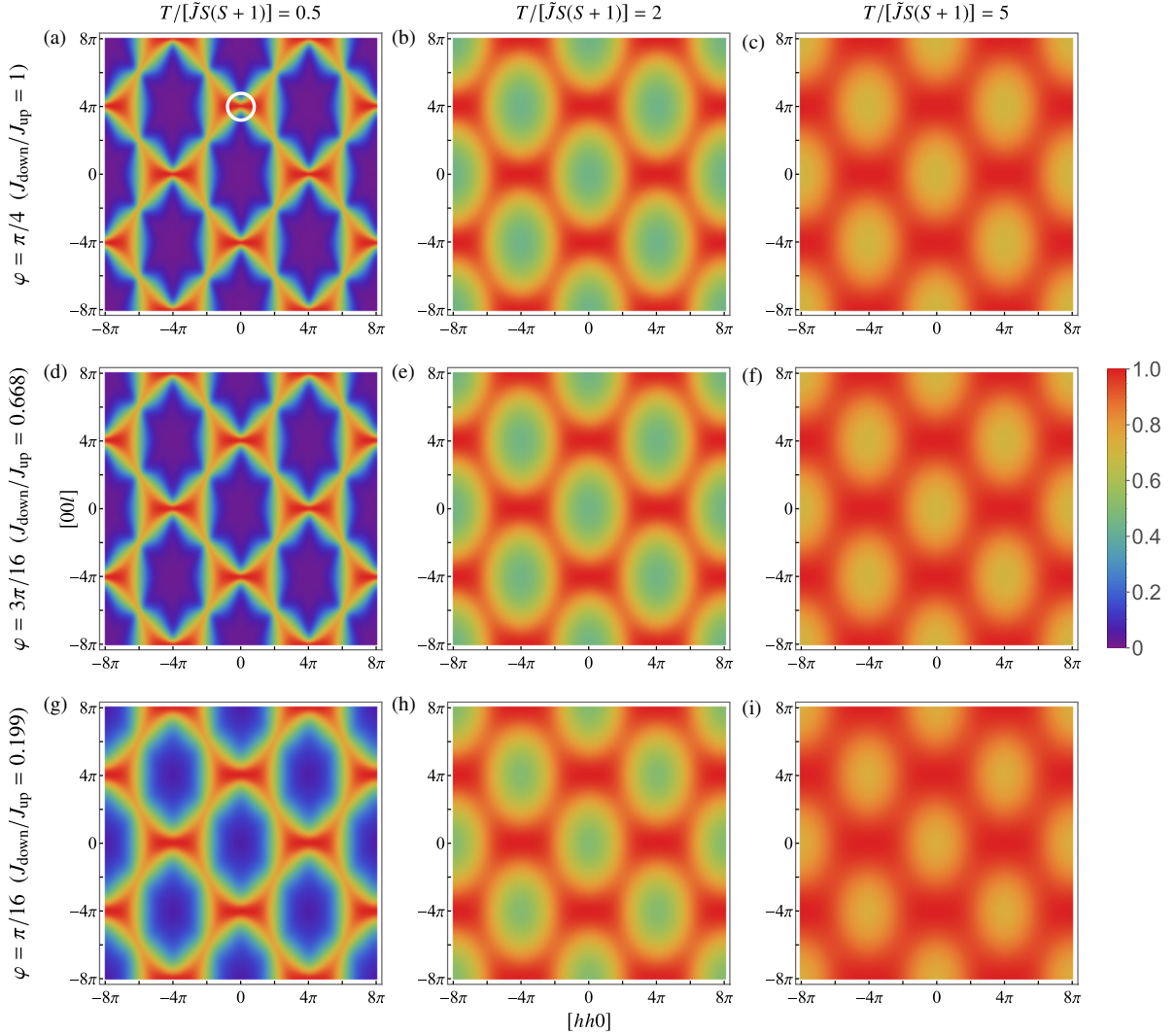
FIG. 3. For the classical ( S \rightarrow \infty ) nearest-neighbor Heisenberg antiferromagnet, the spin susceptibility profile (in units of 1/[\tilde{J}S(S+1)] ) in the [hhl] plane obtained using PFFRG and evaluated for (a)–(c) the isotropic model, (d)–(f) the breathing model for \varphi = 3\pi/16 , and (g)–(i) the breathing model for \varphi = \pi/16 at three different temperatures: T/[\tilde{J}S(S+1)] = 0.5 [(a),(d),(g)], T/[\tilde{J}S(S+1)] = 2 [(b),(e),(h)], and T/[\tilde{J}S(S+1)] = 5 [(c),(f),(i)]. In (a), we encircle the pinch point at \mathbf{k} = (0, 0, 4\pi) . Each plot has its own color scale, where the red corresponds to the maximum of each plot and blue is fixed to zero.
