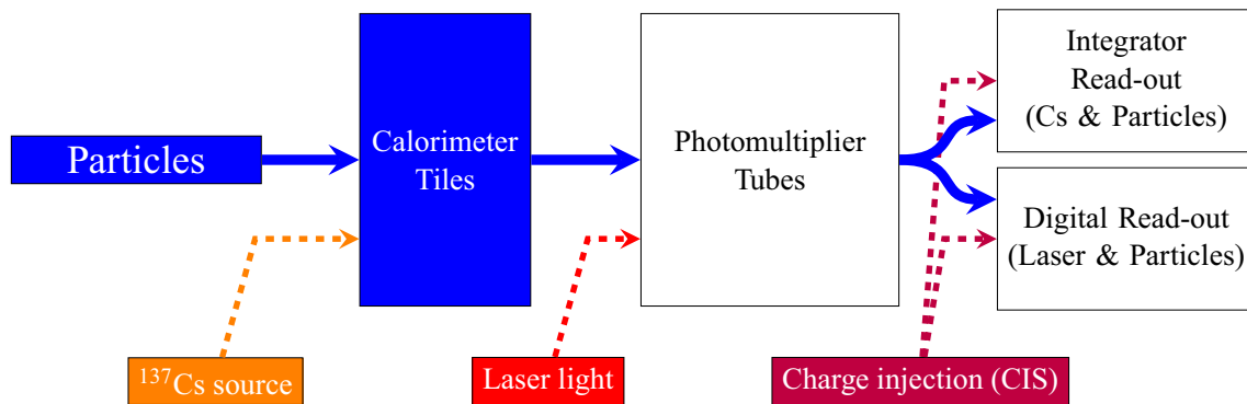
Fig. 13 The signal paths for each of the three calibration systems used by the TileCal. The physics signal is denoted by the thick solid line and the path taken by each of the calibration systems is shown with dashed lines
