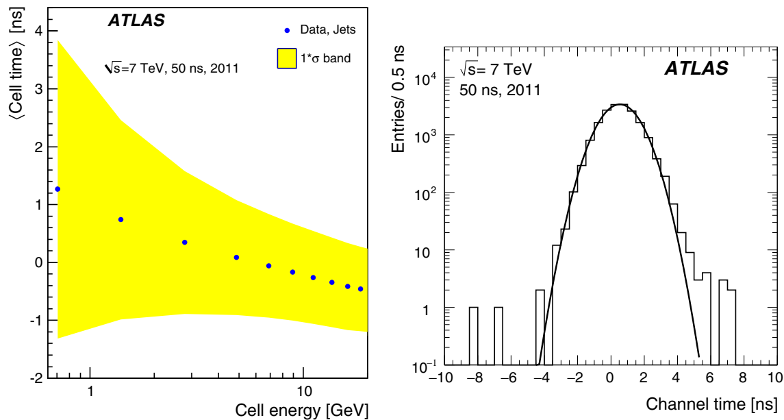
Fig. 5 Left: the mean cell reconstructed time (average of the times in the two channels associated with the given cell) as measured with jet events. The mean cell time decreases with the increase of the cell energy due to the reduction of the energy fraction of the slow hadronic
