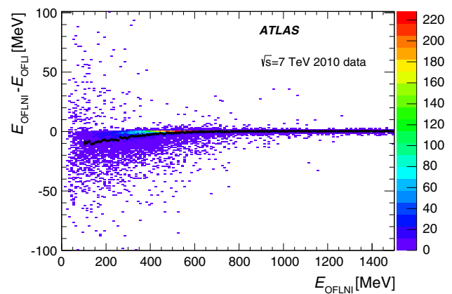
Fig. 4 The absolute difference between the energies reconstructed using the optimal filtering reconstruction method with the non-iterative ( E_{\text{OFLNI}} ) and iterative ( E_{\text{OFLI}} ) signal reconstruction methods as a function of energy. The black markers represent mean values of E_{\text{OFLNI}} - E_{\text{OFLI}} per a bin of E_{\text{OFLNI}} . The parabolic correction is applied to E_{\text{OFLNI}} . The data shown uses high p_T ( > 20 GeV) isolated muons from \sqrt{s} = 7 TeV collisions recorded in 2010
