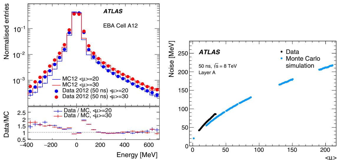
Fig. 12 The area-normalised energy spectra in cells A12 over all TileCal modules for two different pile-up conditions \langle\mu\rangle = 20, 30 (left) and the total noise, computed as the standard deviation of the energy
