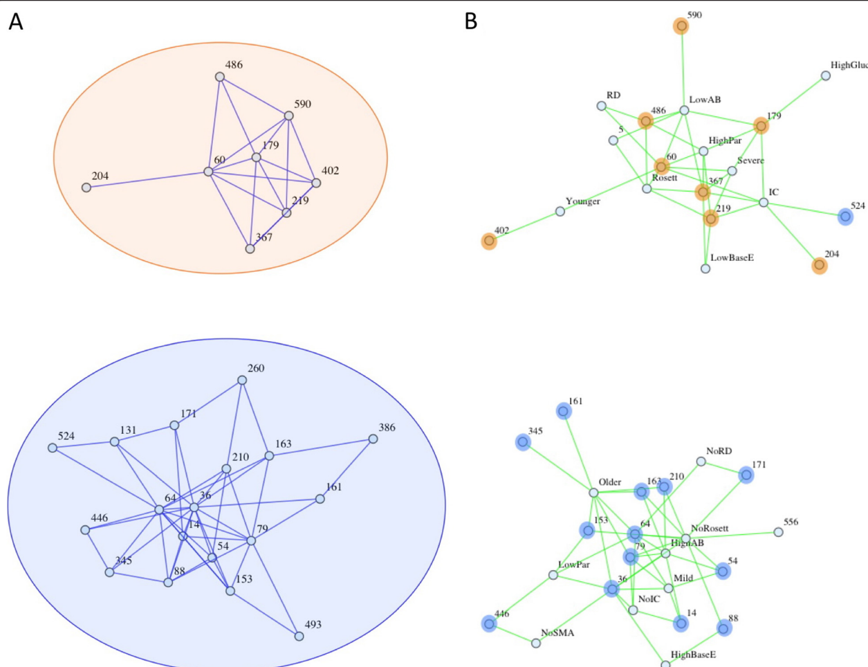
Figure 3 Two HB subnetworks: associated with severe versus mild spectrum disease. HB networks reveal two discrete HB subsets—one being associated with severe spectrum phenotypes (orange) and the other being associated with mild spectrum phenotypes (blue). (A) The network of significant positive linkage disequilibrium coefficients (D) among HBs in the genomic dataset, based on a one-tailed significance threshold of p \leq .025 , reveals two subnetworks of linked HBs. (B) The network of significant associations between HB expression rates and phenotypes ( p \leq 0.05 ) with nodes colored according to the subnetworks of A. The HBs in the orange subnetwork are generally associated with severe disease spectrum phenotypes, whereas those in the blue subnetwork are generally associated with mild. The lack of connectivity between the severe and mild spectrum phenotypes in A is highly significant: even just considering the nodes of degree 3 or less, p < 0.0001 for the fact that each HB in the network is associated with mild or severe spectrum phenotypes, but not both. SMA = severe malarial anemia, Rosett = rosetting, RD = respiratory distress, Severe = severe disease, Mild = mild disease, Older = high host age, Younger = low host age, Par = parasitemia, BGlu = blood glucose (low levels indicate hypoglycemia), BaseE = base excess (low levels indicate metabolic acidosis), AB = antibody response.
