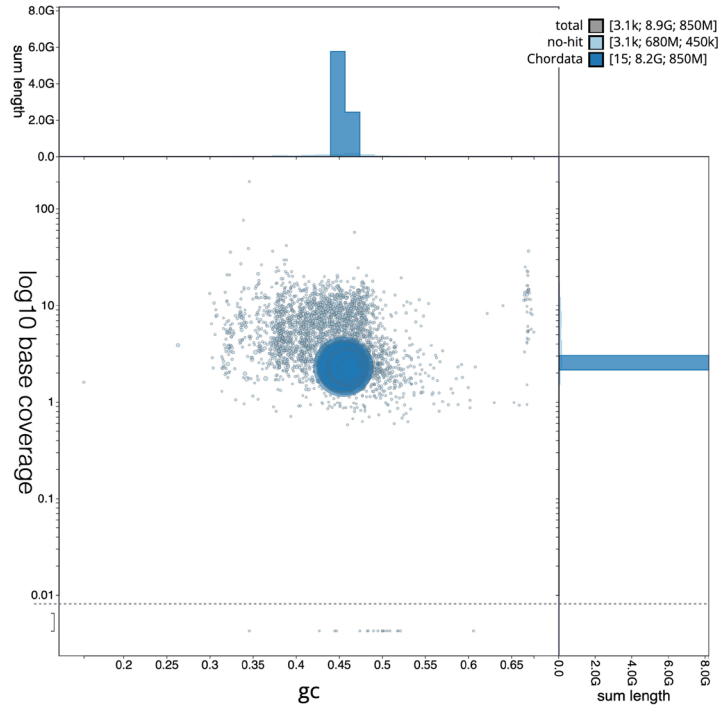
Figure 3. BlobToolKit plot of base against GC proportion for genome assembly Pseudophryne corroboree , aPseCor3.hap2. Circles are sized in proportion to sequence length. Histograms show the distribution of sequence length sum along each axis. Base coverage values are log10 transformed. An interactive version of this figure is available at: https://blobtoolkit.genomehubs.org/view/GCA_028390025.1/dataset/GCA_028390025.1/blob?plotShape=circle .
