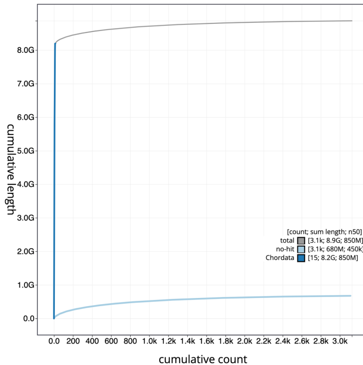
Figure 4. Genome assembly of Pseudophryne corroboree , aPseCor3.hap2: BlobToolKit cumulative sequence plot. The grey line shows cumulative length for all sequences. Coloured lines show cumulative lengths of sequences assigned to each phylum using the buscogenes taxrule. An interactive version of this figure is available at: https://blobtoolkit.genomehubs.org/view/GCA_028390025.1/dataset/GCA_028390025.1/cumulative .
