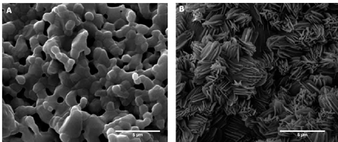
Figure 3. Calcium phosphate based ceramics attract natural apatite deposition on its surface after immersion in physiological solutions. This occurs through an ion exchange reaction between the calcium phosphate in the ceramic coating and the ions and proteins in the surrounding solution. SEM images of BCP (bi-phasic calcium phosphates) scaffolds before and after immersion in phosphate buffered saline (PBS). (A) HA/TCP scaffolds before immersion in PBS; (B) HA/TCP scaffolds after immersion in PBS for 2 weeks. Note the deposition of apatite crystals on the scaffold surface. Reprinted from [82] with permission from Bentham Open, copyright 2010.
