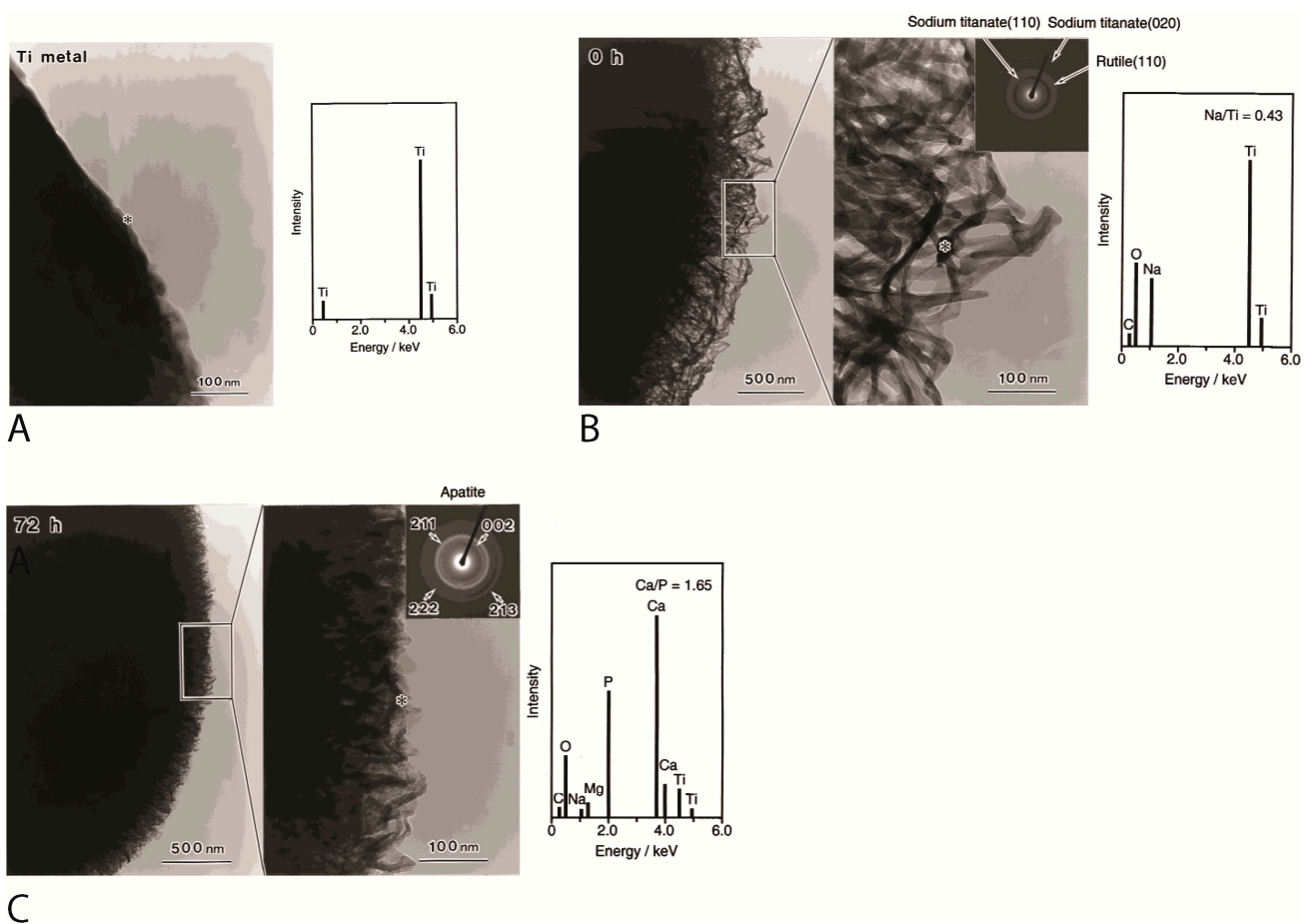
Figure 4. Functionalization of Titanium surfaces with hydroxyl ( \text{OH}^- ) groups enhanced nucleation of bone like apatite on the metal surface when it is submerged in physiological solutions. The figure shows transmission electron microscopy (TEM) images and energy dispersive X-ray spectrometry (EDX) results of titanium surfaces treated with NaOH and heat followed by immersion in physiological solution. (A) Titanium surface before NaOH and heat treatment; (B) Titanium surface after NaOH and heat treatment. Note the layer of amorphous sodium titanate that forms on the titanium surface; and (C) NaOH and heat-treated titanium surface after 72 h immersion in physiological solution. Note the deposition of natural apatite on the implant surface. * Center of electron diffraction and EDX analysis. Reprinted from [62] with permission from John Wiley & Sons, Inc., Copyright 2014.
