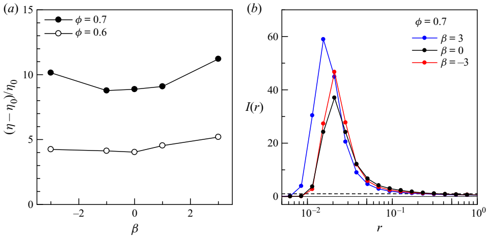
Figure 4. Effect of the swimming mode \beta on the viscosity ( Sq = 1 ). (a) Excess apparent viscosity with \phi = 0.6 and 0.7 . (b) Normalised probability density function distribution of squirmers with \beta = 3, 0 and -3 ( \phi = 0.7 ).
