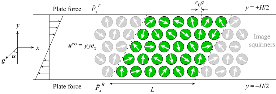
Figure 10. A suspension of N = n_x n_y = 132 spherical squirmers, subject to a background shear flow \mathbf{u}^\infty = \gamma y \mathbf{e}_x between two parallel plates. The position, \mathbf{x}_i , and orientation, \mathbf{e}_i , of each squirmer are confined to lie in the x - y plane. The direction of gravity is \mathbf{g} = -g(\sin \alpha, \cos \alpha, 0) .
