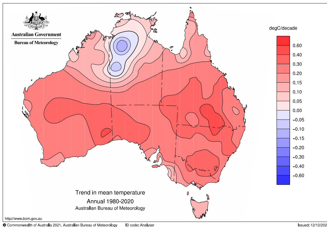
Figure 2. Trend in mean temperature – Annual 1980-2020
