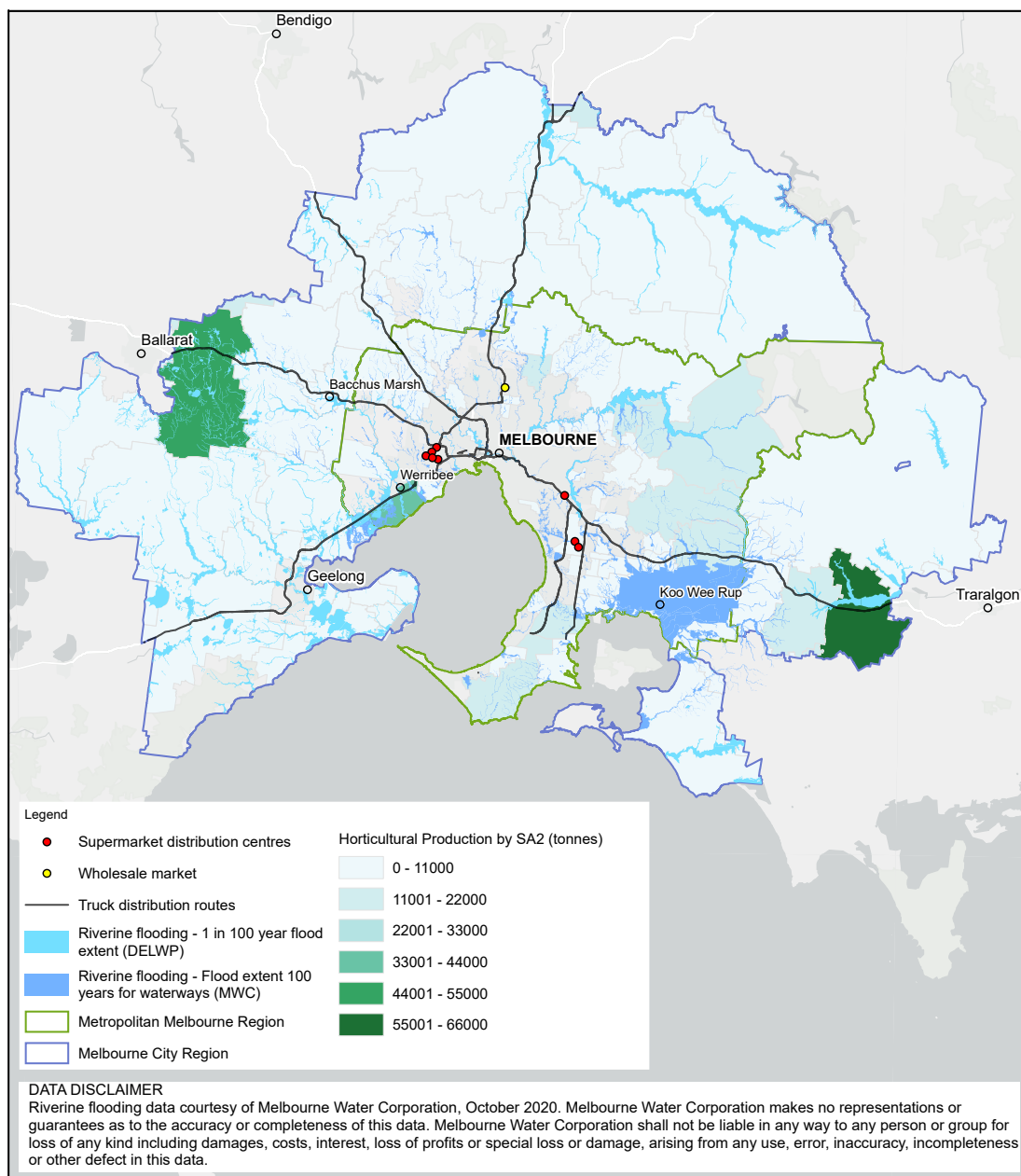
Figure 5. Areas at risk of riverine flooding in Melbourne's city region
