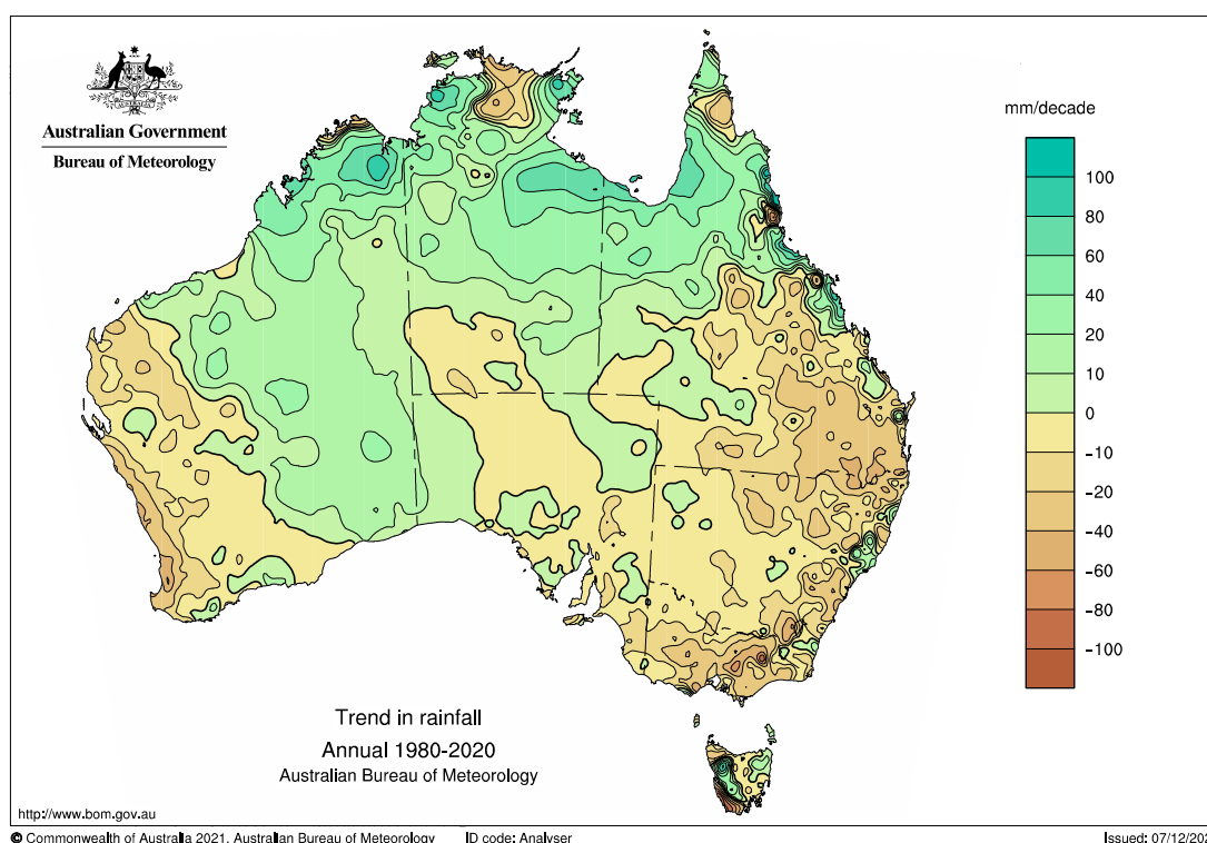
Figure 4. Trend in total rainfall - Annual 1980-2020
