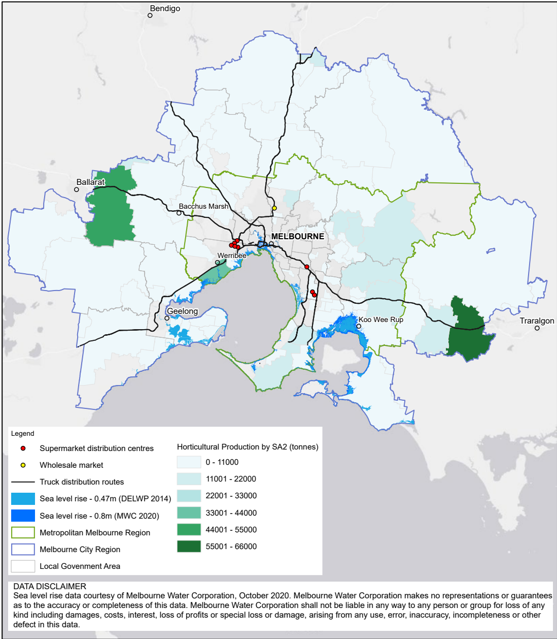
Figure 6. Areas at risk of sea level rise in Melbourne's city region
