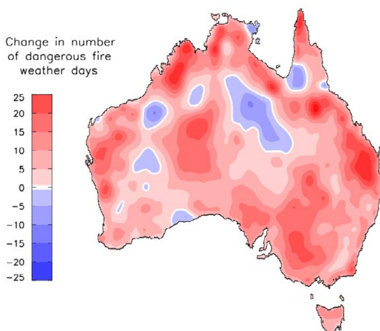
Figure 3. Change in the number of dangerous fire weather days 1950 – 2020 (source: Bureau of Meteorology)
