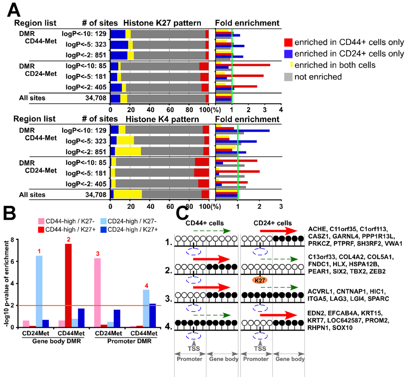
Figure 7. Integrated view of genome-wide gene expression and DNA and histone methylation patterns. (A) Genomic regions ( \pm 5 kb and \pm 0 kb from DMR for K27 and K4, respectively) associated with DMRs in one cell type (e.g., CD44+ cells) are enriched for K4 or K27 mark in the other (e.g., CD24+ cells). Bar chart shows observed/expected ratio of the indicated MSDK sites with the designated K27 and K4 patterns between CD44+ and CD24+ cells. (B) Associations between gene expression and histone and DNA methylation patterns. Y-axis shows the -\log_{10} p-value of enrichment for genes with the indicated expression and histone modification pattern in gene body and promoter DMRs. Orange line indicates -\log_{10} (p value) of statistical significance, numbers 1–4 mark significantly enriched patterns. (C) Schematic models depicting possible changes in DNA methylation and K27 enrichment during CD44+ to CD24+ cell differentiation and their effect on gene expression based on data presented in panel B. Examples of genes within each group are listed. White (unmethylated) and black (methylated) circles indicate potential DNA methylation sites (i.e., CpG) in the promoter and gene body, blue and orange ovals represent lack and presence of K27 mark, respectively. Red and dashed green arrows indicate increased and decreased gene expression, respectively. doi:10.1371/journal.pgen.1001369.g007
