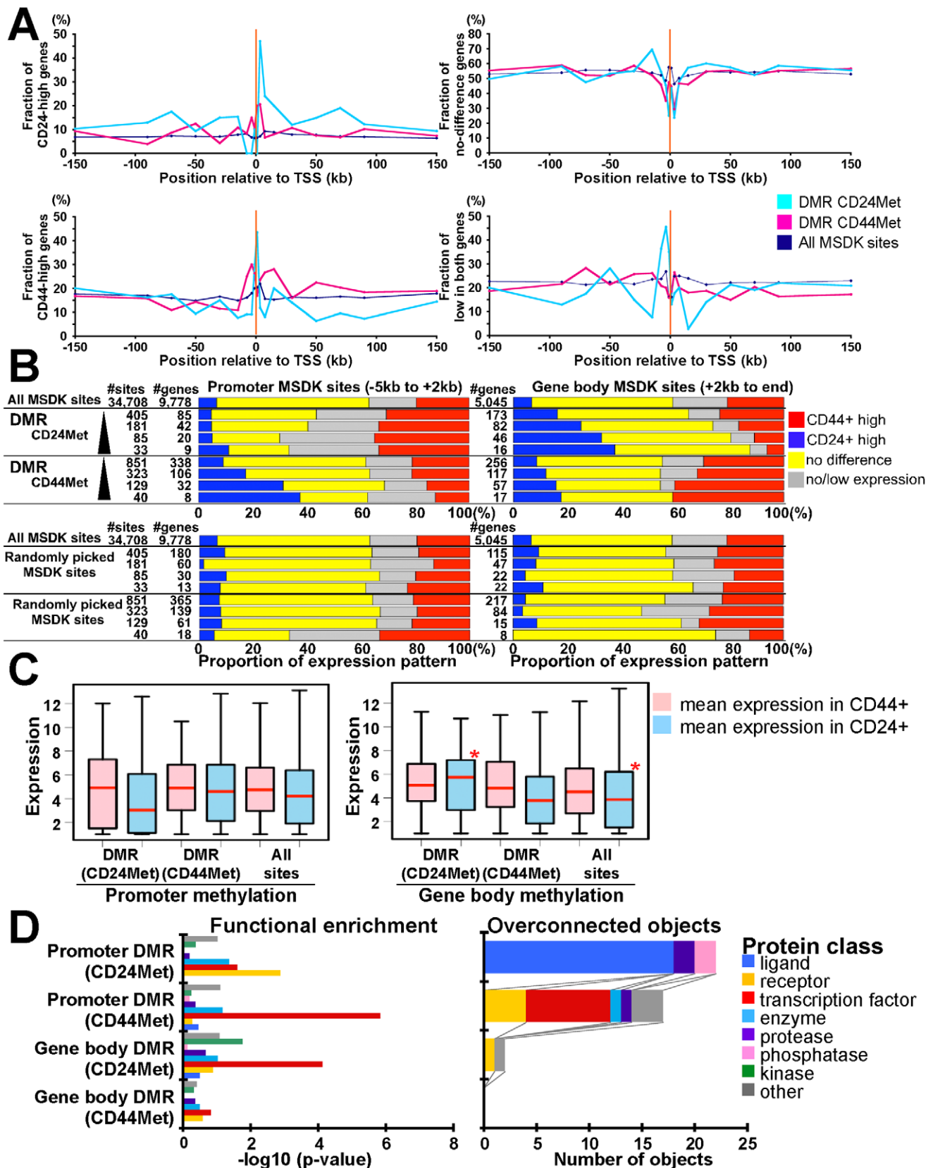
Figure 6. Combined view of DNA methylation and gene expression patterns. (A) Associations between fraction of genes highly expressed in CD24+ or CD44+ cells and the location of DMRs ( p < 10^{-5} ) in the two cell types relative to TSS. Y-axes show fraction of genes in the four different gene expression groups (i.e. CD24-high, CD44-high, no difference, and not expressed) relative to the location of DMRs hypermethylated in CD24+ (blue line) or CD44+ (red line) cells and all MSDK sites used as control. (B) Differentially ( \geq 2 -fold difference) expressed genes are enriched in DMRs. Bar
