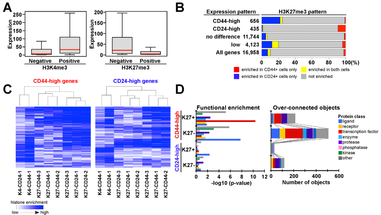
Figure 3. Associations between chromatin and cell type-specific expression patterns. (A) Overall correlation between histone methylation (K4, K27) and gene expression in CD44+ progenitors from sample 1. Box plot shows distribution of gene expression of corresponding genes in each category. Red bar: median, box: interquartile ranges and whisker; most extreme value within 1.5 times of box length. (B) Bar chart shows the correlation between cell type-specific K27 enrichment and gene expression patterns. Blue and red: K27-enriched only in CD24+ and CD44+ cells, respectively, yellow and gray: K27 enriched in both and neither cell type. (C) Differences in K27 patterns between CD24+ and CD44+ cells are consistent in three individual samples and distinct from that of K4 profiles. Heatmap depicting unsupervised clustering of histone modification patterns of genes highly expressed in CD44+ (656 genes) and CD24+ (435 genes) cells. Blue color indicates the level of enrichment for the indicated histone modification based on the ranking of ChIP-Seq read counts for each gene in each sample. (D) Differentially expressed genes that are enriched (K27+) or not enriched (K27-) for K27 were analyzed for relative enrichment with the indicated protein classes (left panel) and for relative connectivity (right panel). X-axes indicate -\log_{10} p-values for enrichment with the listed protein classes (left panel) and the number of overconnected objects, defined as proteins with higher than expected number of interactions, in each functional category within each group (right panel), respectively. doi:10.1371/journal.pgen.1001369.g003
