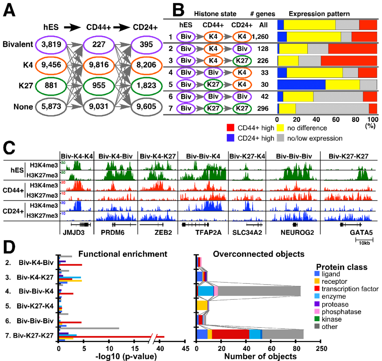
Figure 5. Changes in chromatin state and cell type-specific gene expression patterns. (A) Number of genes for each of the four possible chromatin states (i.e., bivalent – purple, K4 only – orange, K27 only – green, and neither – gray) in the indicated three cell types. (B) Potentially interesting differences in chromatin patterns. Bar chart shows associations between changes in chromatin-state and gene expression patterns. Each row indicates the type of chromatin-state change and the number of genes in each category. Blue and red: genes highly expressed in CD24+ and CD44+ cells, respectively ( \geq 2 -fold change). Yellow and gray: genes with \leq 2 -fold difference between CD24+ and CD44+ cells and with low/no detectable expression in either cell type, respectively. (C) Representative examples of genes in each category. ChIP-Seq tag counts for K4 and K27 modification in hES, CD44+, and CD24+ cells are shown. Total aligned tag count was scaled to 10 million and tag counts were averaged over a 10 bp window. (D) Functional enrichment analysis of genes within each chromatin pattern category (left panel) and the number of overconnected objects in each functional category within each group (right panel). X-axis indicates -\log_{10} p-values for enrichment with the indicated protein class (left panel) and the number of overconnected objects (right panel), respectively. Definitions are the same as described in Figure 3D. doi:10.1371/journal.pgen.1001369.g005
