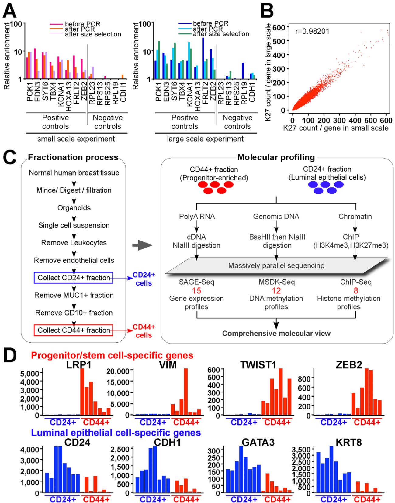
Figure 1. Overview of experimental design and data analysis. (A) qPCR validation steps during ChIP-Seq library preparation using small and large scale protocols. Several regions known to be K27-enriched (positive controls) or not-enriched (negative controls) in MCF-7 cells were tested by qPCR using DNA templates before and after linker-mediated PCR amplification and after size-selection. Y-axis indicates enrichment relative to averaged negative controls. (B) Comparison of small-scale and standard ChIP-Seq experiments. Scatter plots depict the counts of ChIP-Seq reads for each gene. X and Y-axes indicate mapped read counts around promoter regions ( \pm 5 kb from TSS) for each gene in small-scale and in standard
