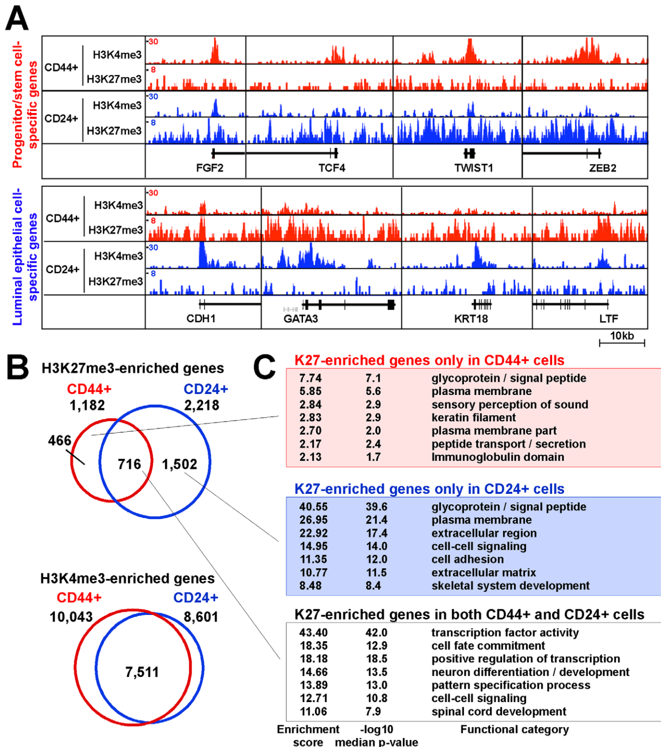
Figure 2. Distinct histone methylation profiles of human CD44+ mammary epithelial progenitors and CD24+ differentiated luminal epithelial cells. (A) Examples of histone modification patterns of genes known to be expressed in stem or luminal cells. Total aligned tag count in each ChIP-Seq library was scaled to 10 million, Y-axis shows tag counts averaged over a 10 bp window. (B) Comparison of genes enriched for the indicated histone marks in CD44+ and CD24+ cells. Venn diagram depicts the number of unique and overlapping genes. (C) Functional enrichment analysis of K27-enriched genes using DAVID Functional Annotation Tool. doi:10.1371/journal.pgen.1001369.g002
