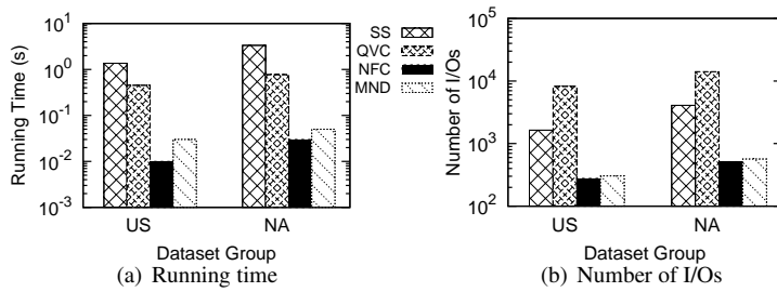
Fig. 13 Performance comparison on real datasets
