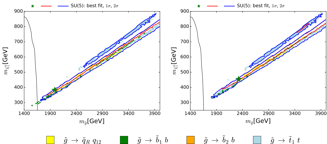
Fig. 2 The solid lines show the CMS 95% CL exclusion in the (m_{\tilde{g}}, m_{\tilde{\chi}_1^0}) plane [9], assuming a simplified model with heavy squarks and 100% BR for \tilde{g} \rightarrow q\tilde{q}\tilde{\chi}_1^0 . The left (right) panel shows the best-fit point (green star), 68 and 95% CL contours (red and blue lines, respectively) for (m_{\tilde{g}}, m_{\tilde{\chi}_1^0}) obtained without (with) the CMS 13-TeV
