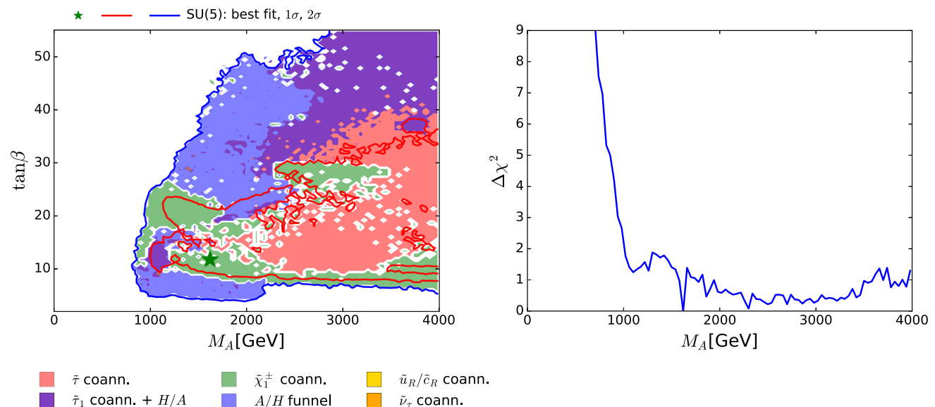
Fig. 9 On the left the (M_A, \tan\beta) plane in the SUSY SU(5) GUT model. The line colours and shadings are the same as in Fig. 4. On the right the \chi^2 likelihood function for the pseudoscalar mass
