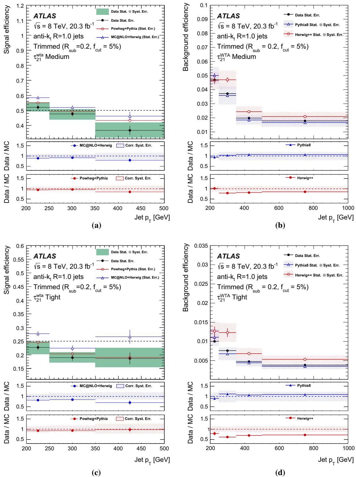
Fig. 24 W boson tagging efficiencies in ranges of jet p_T for (left) signal W -jets in t\bar{t} events and (right) multijet background. The \epsilon_W^{\text{G}\&\text{T}} \sim 50\% working points obtained with the combined mass window and \tau_{21}^{\text{WTA}} requirements are shown in a and b , and the \sim 25\% working points are shown in c , d . The deviations from 50 and 25 % in a and c respec-
