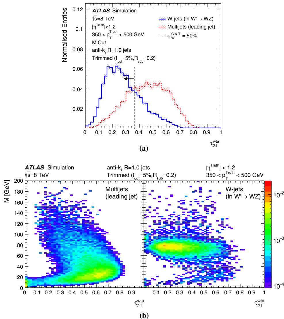
Fig. 12 The \tau_{21}^{wta} variable, for R2-trimmed jets: a distributions in signal (blue solid line) and background (red dashed) in MC in the range 350 < p_T < 500 GeV, obtained after applying the 68 % signal efficiency mass window requirement (discussed in Sect. 6.1); b correlation with the leading jet's mass in (left) multijet background and (right)
