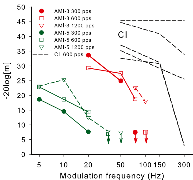
FIG. 5. Results of experiment 2, showing TMTFs of AMI-3 (red) and AMI-5 (green) along with the TMTFs of five CI users re-plotted from Fraser and McKay (2012). The measurement techniques were identical in the two studies. m is the modulation index, where m=1 corresponds to 100 % modulation ( 20 \log[m]=0 ). The symbols with downward arrows indicate conditions in which the subject could not detect the largest modulation depth used of 50 CL.
