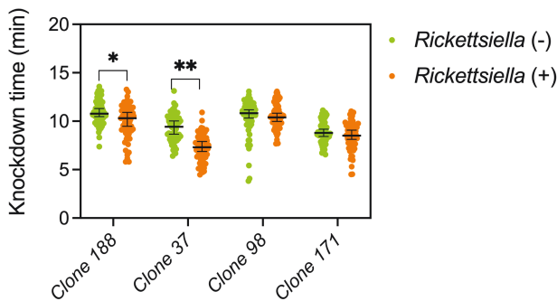
Fig. 4. Effects of Rickettsiella infection on heat tolerance in four clones of M. persicae . Heat knockdown time was tested at a constant 41.5 °C across all Rickettsiella (-) and Rickettsiella (+) M. persicae lines. Dots represent data from 60 individual aphids, while vertical lines and error bars are medians and 95% confidence intervals, respectively. Significant differences are marked with * and ** above the dots, representing P < 0.05 and P < 0.01 by independent t-tests between Rickettsiella (-) and Rickettsiella (+) M. persicae , respectively.
