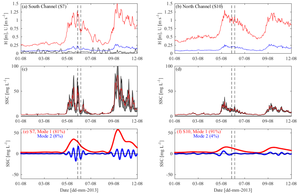
Figure 9. Incident incident ( H_{m0,sw} , red) and infragravity ( H_{m0,ig} , blue) wave forcing, and the absolute current ( U , black)(a) in the south channel (S7) and (b) in the north channel at (S10). Note: the current was not measured in the at S10. Hourly mean SSCs are shown in red (c) in the south channel at S7, (d) in the north channel at S10. The lower limit represents the 1 st quartile while the upper limit indicates the 3 rd quartile for each hourly burst of data. The bottom row shows the decomposed SSC time-series indicating the first (red) and second (blue) modes, which explained the majority of the signal variance, at (e) S7 and (f) S10. The vertical dashed lines indicate a high and low tide.
