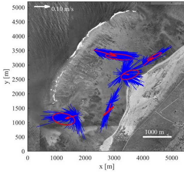
Figure 4 Hourly mean depth-averaged current data (blue), with the experiment-averaged mean current vector indicated by the arrows. The ellipses (red) indicate the direction of the major and minor semi-axes of variability. The scale of the ellipse represents one standard deviation.
