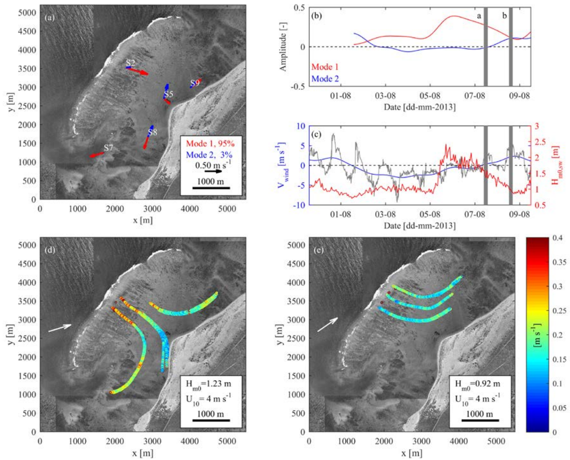
Figure 5. (a) The first (red) and second (blue) 36-hour empirical mode of subtidal current variability along with (b) the amplitude of the first (red) and second (blue) modal amplitude time-series from the EOF analysis. To facilitate comparison of the two modes, the amplitude of the arrows and amplitude time-series have been scaled (factor=0.64) so that the arrows are equal in magnitude at S8. (c) The alongshore wind speed V_{wind} averaged over 10 min (grey) and at subtidal temporal scales (blue). The fore reef incident wave height ( H_{m0,sw} ) is shown in red. The grey shading indicates the drifter experiments shown in (d) that started at 09:32 on 7 August 2013 and (e) that started at 12:40 on 8 August 2013. (d-e) Surface current
