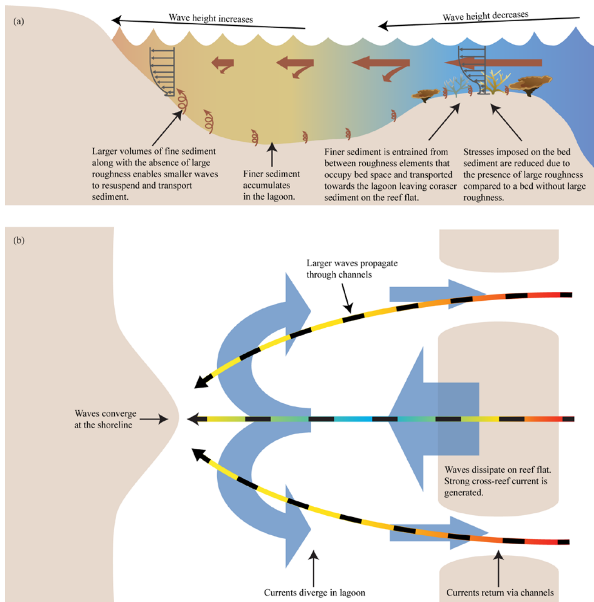
Figure 11 Conceptual model of sediment transport processes in a fringing coral reef-lagoon system. (a) Cross section of waves, currents, and sediment processes across a reef and lagoon. Brown arrows indicate the direction of sediment transport by currents and the upward arrows indicate sediment resuspension. Note that an increase in suspended sediment concentration is indicated by brown shading. (b) Plan view of the wave rays (colored lines) and current
