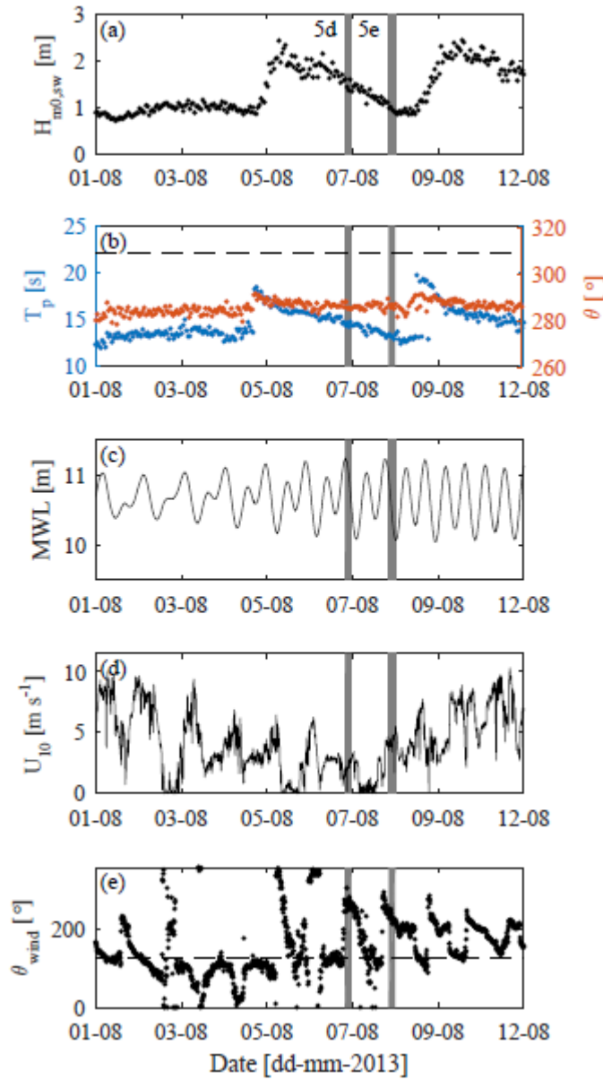
Figure 2. The offshore (a) swell wave height H_{m0,sw} ; (b) peak wave period T_p and peak incident wave direction \theta with cross-reef direction denoted by the horizontal dashed line; (c) water depth measured on the fore reef at S1; (d) The 10 min mean wind speed; and (e) the direction \theta_{wind} measured in Nautical convention ( 0^\circ and 360^\circ indicates a southerly wind) at
