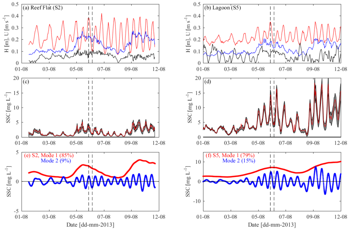
Figure 8. Incident incident ( H_{m0,sw} , red) and infragravity ( H_{m0,ig} , blue) wave forcing, and the absolute current ( U , black)(a) on the reef flat at (S2) and (b) in the lagoon at S5. Hourly mean SSCs are shown in red (c) on the reef flat at S2, (d) in the lagoon at S5. The lower limit represents the 1 st quartile while the upper limit indicates the 3 rd quartile for each hourly burst of data. The bottom row shows the decomposed SSC time-series indicating the first (red) and second (blue) modes, which explained the majority of the signal variance, at (e) S2 and (f) S5. The vertical dashed lines indicate a high and low tide.
