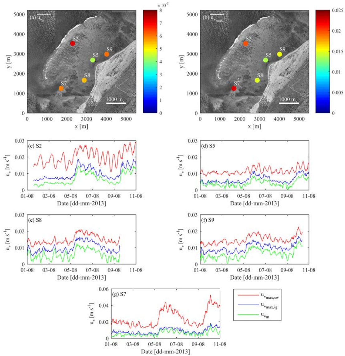
Figure 7. The experiment averaged near bed (a) mean wave-current shear velocity \overline{u_{*m}} and the (b) maximum wave-current shear velocity \overline{u_{*max}} . The colorbars (with different scales) denote the shear velocities in \text{m s}^{-1} . The shear velocities near the bed (c) on the reef flat at S2, (d) in the lagoon near the tip of the salient at S5, (e) south of the salient at S8, (f) north of the salient at S9 and (g) in the southern channel at S7, generated by incident wave-current
