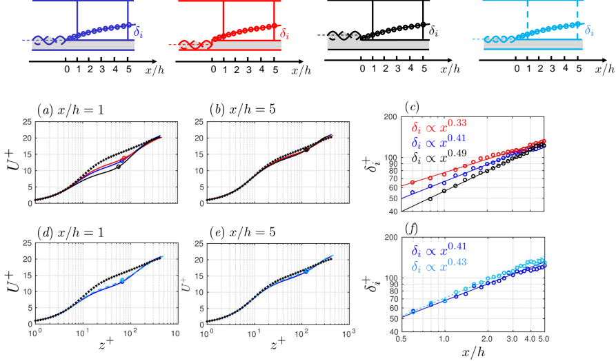
Fig. 3 Roughness origin effect on (a,b) U^+ profiles and (c) IBL thicknesses \delta_i^+ . Roughness size effect on (d,e) U^+ profiles and (f) \delta_i^+ . \delta_i^+ is also marked on the profiles. The quantities in plus units are normalized by the local u_\tau and \nu . Fully developed open-channel flow at Re_\tau = 437 (+).
