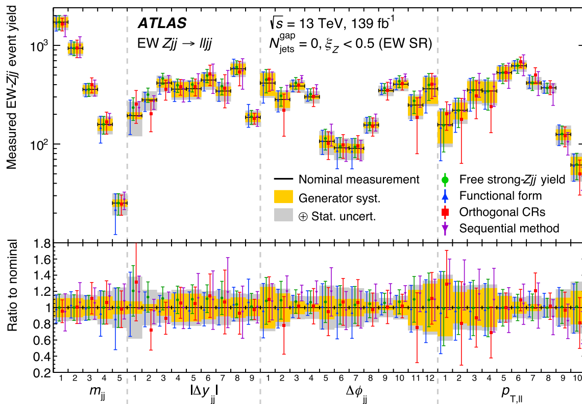
Fig. 12 Extracted EW Zjj event yields in bins of the four observables measured using five different methods. The nominal measurements with their associated uncertainties are shown as bands, while the measurements based on the four variations to the EW Zjj extraction methodology are shown as points with error bars corresponding to their associated total uncertainty (excluding the experimental systematics, that tend to be significantly smaller)
