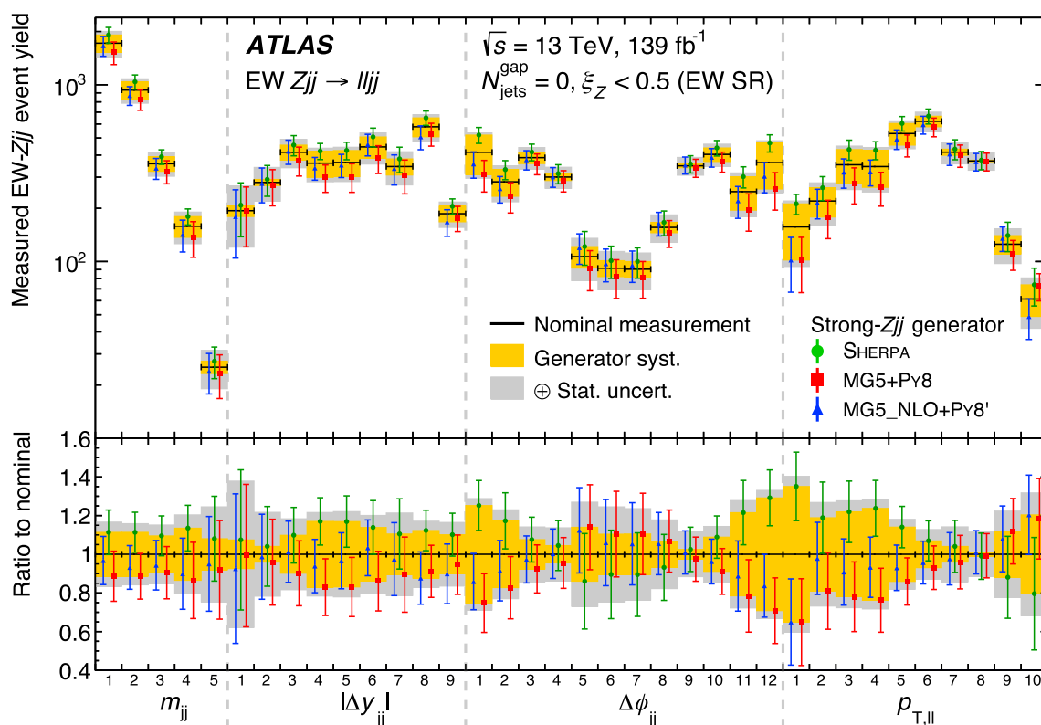
Fig. 11 EW Zjj event yields obtained when using the SHERPA, MG5_NLO+PY8' and MG5+PY8 predictions for the strong Zjj process. The extracted EW Zjj yields are presented for each bin of the four observables ( m_{jj} , |\Delta y_{jj}| , \Delta\phi_{jj} and p_{T,\ell\ell} ). The nominal EW Zjj measurement is defined as the midpoint of the three generator-specific measurements, with a 'generator choice' systematic defined by the envelope. Experimental systematic uncertainties are not shown (they tend to be small as can be seen in Fig. 6)
