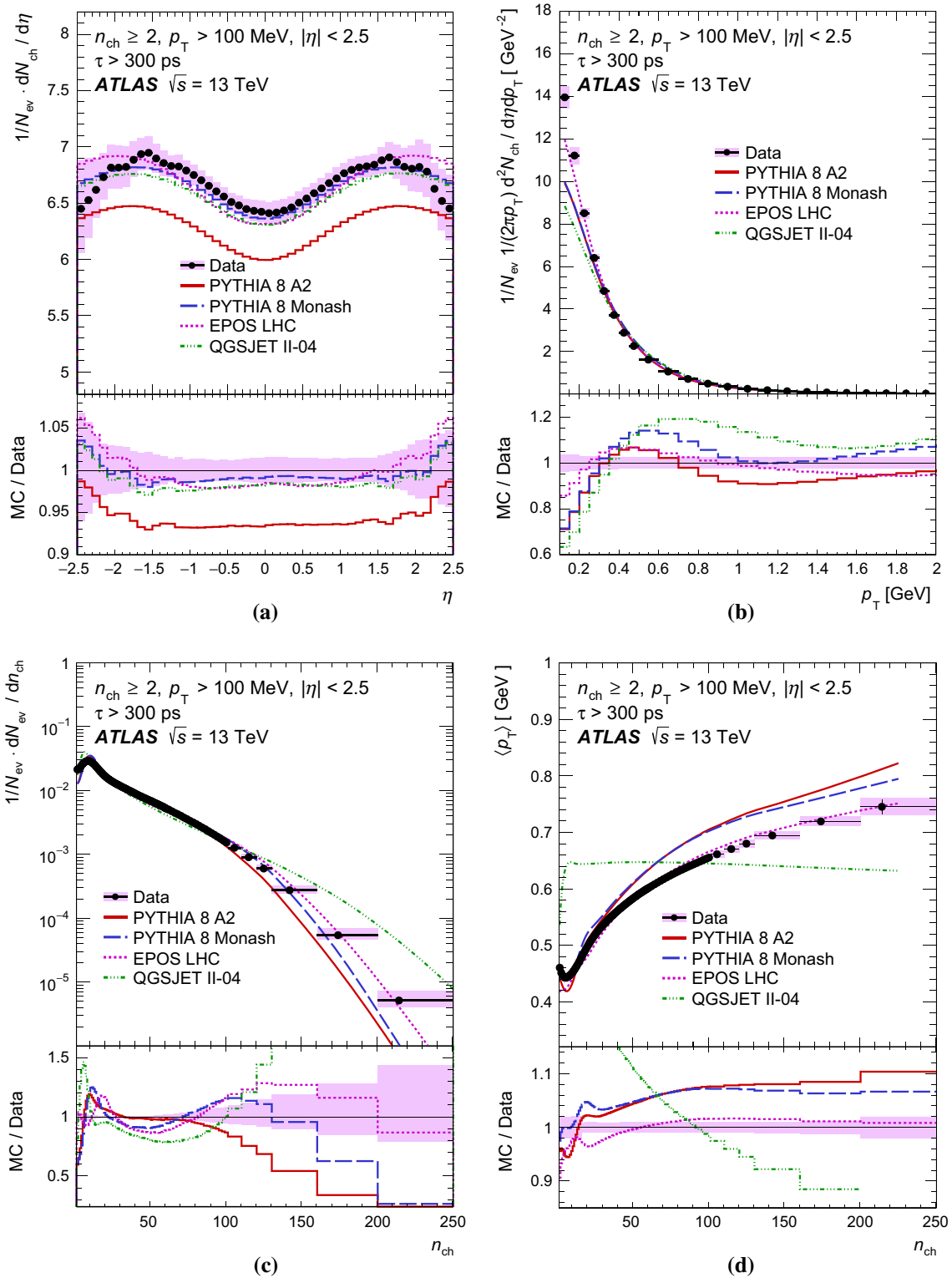
Fig. 4 Primary charged-particle multiplicities as a function of a pseudorapidity \eta and b transverse momentum p_T , c the primary charged-particle multiplicity n_{\text{ch}} and d the mean transverse momentum \langle p_T \rangle versus n_{\text{ch}} for events with at least two primary charged particles with p_T > 100 MeV and |\eta| < 2.5 , each with a lifetime \tau > 300 ps. The black dots represent the data and the coloured curves the different MC
