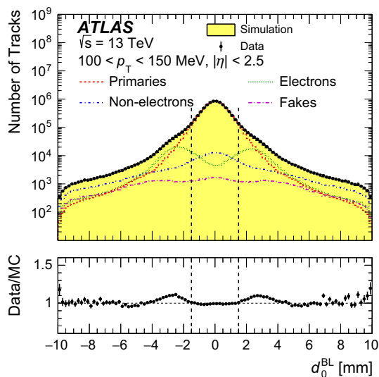
Fig. 2 Comparison between data and PYTHIA 8 A2 simulation for the transverse impact parameter d_0^{\text{BL}} distribution. The d_0^{\text{BL}} distribution is shown for 100 < p_T < 150 MeV without applying the cut on the transverse impact parameter. The position where the cut is applied is shown as dashed black lines at \pm 1.5 mm. The simulated d_0^{\text{BL}} distribution is normalised to the number of tracks in data and the separate contributions from primary, fake, electron and non-electron tracks are shown as lines using various combinations of dots and dashes . The secondary particles are scaled by the fitted fractions as described in the text. The error bars on the points are the statistical uncertainties of the data. The lower panel shows the ratio of data to MC prediction
