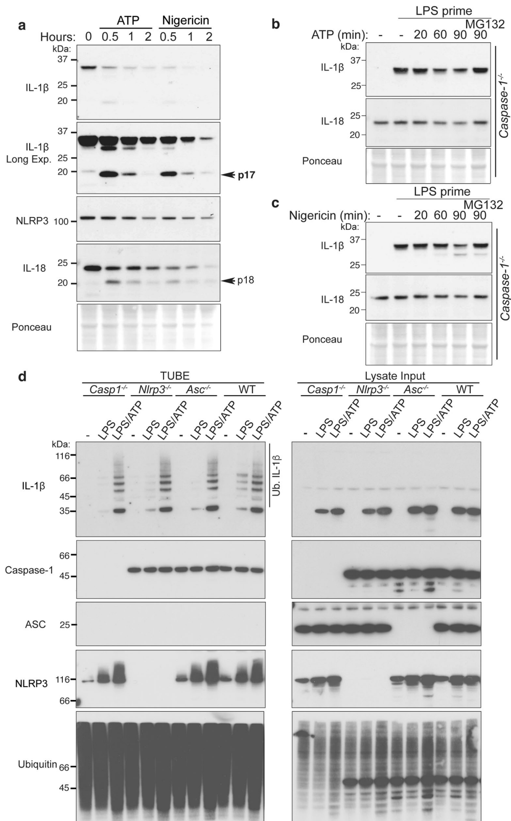
Fig. 3 ATP and nigericin can augment proteasomal-mediated IL-1β degradation. a BMDMs were primed with Lipopolysaccharide (LPS, 50 ng/ml) for 3 h and stimulated with ATP (5 mM) and Nigericin (10 μM) for up to 2 h. Total cell lysates were analyzed by immunoblot. One of three experiments. b, c Caspase-1 -/- BMDMs were primed with LPS (50 ng/ml) for 3 h, and in the last 30 min of priming treated with MG132 (20 μM), as indicated. Cells were treated with b ATP (5 mM) and c Nigericin (10 μM) for up to 90 min. Immunoblots were performed on total cell lysates to detect the specified proteins. One of three experiments. d WT, Nlrp3 -/- , Asc -/- and Caspase-1 -/- BMDMs were primed with LPS (50 ng/ml) for 3 h and stimulated with ATP for 20 min. Ubiquitylated (Ub.) proteins were purified from cell lysates by Tandem Ubiquitin Binding Entities (TUBEs). Immunoblots were performed on cell lysates and TUBE isolated ubiquitylated proteins for the indicated proteins. One of two experiments.
