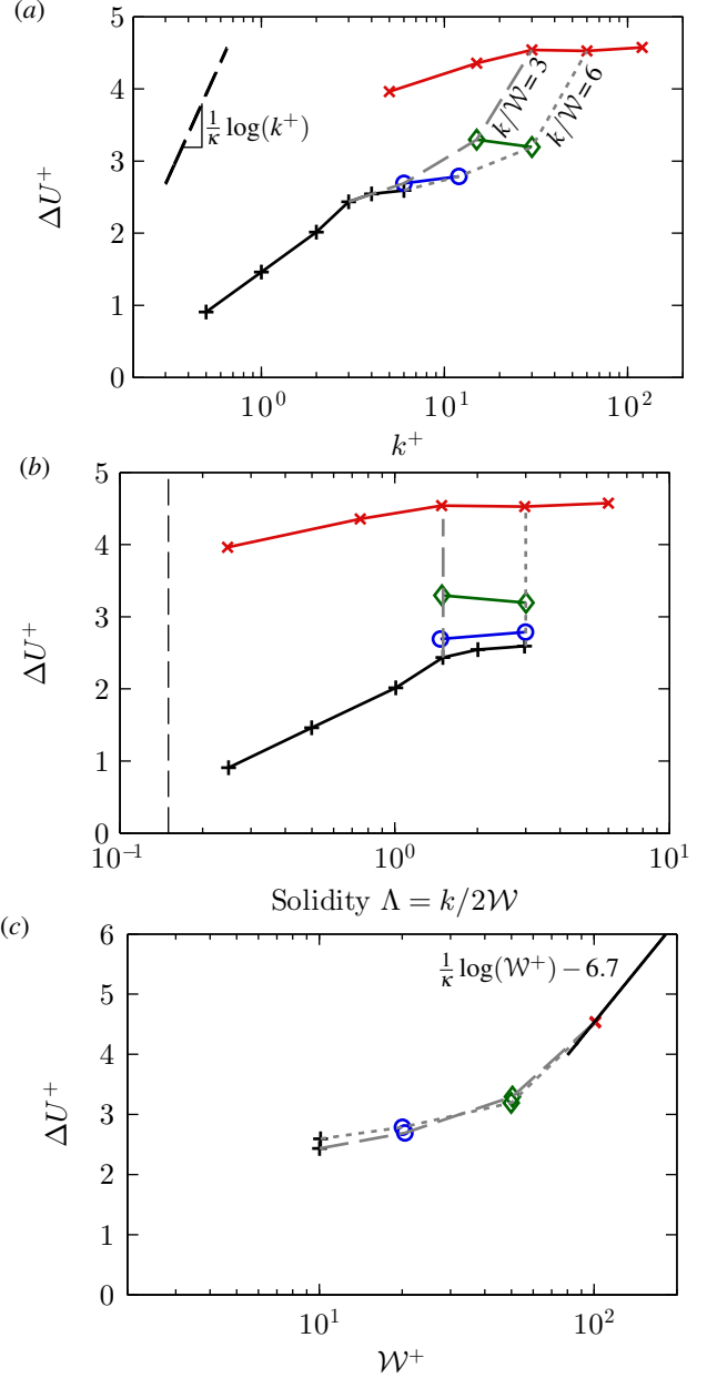
Figure 6. Roughness function, \Delta U^+ , plotted against (a) roughness height, k^+ , (b) solidity, \Lambda , and (c) fluid gap, W^+ . Symbols: +, W^+ = 10 ; ○, W^+ = 20 ; ◇, W^+ = 50 ; ×, W^+ = 100 . Dashed and dotted lines correspond to k/W = 3 and k/W = 6 , respectively.
