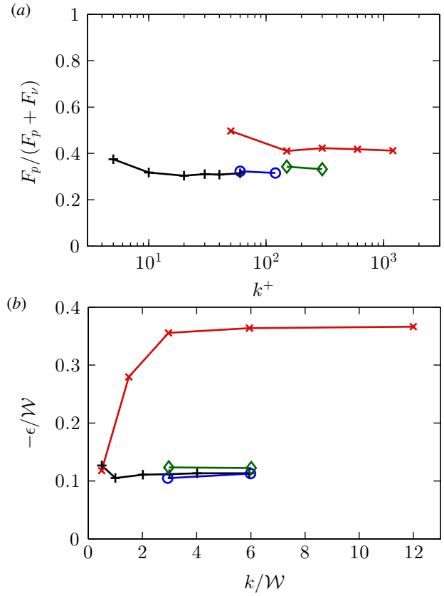
Figure 4. (a) Ratio of pressure to total (viscous + pressure) drag and (b) virtual origin \epsilon normalised on fluid gap W . Symbols: + , W^+ = 10 ; \circ , W^+ = 20 ; \diamond , W^+ = 50 ; \times , W^+ = 100 .
