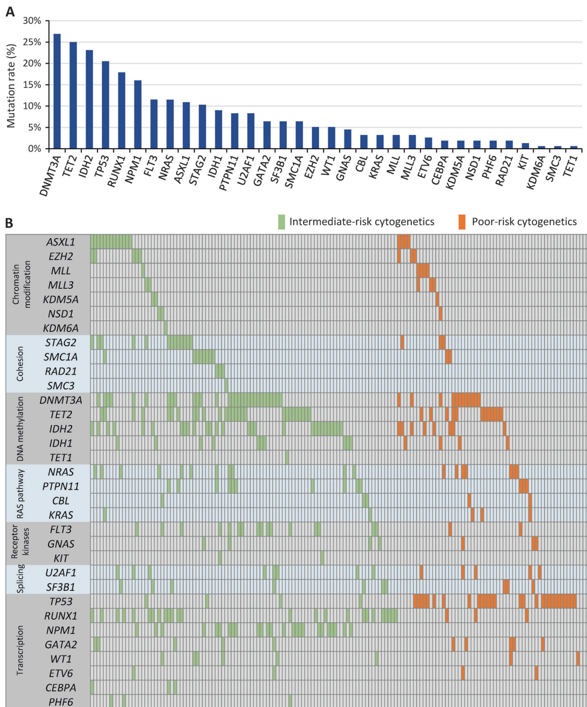
Fig. 4 a Proportions of patients with specific gene mutations. b OncoPrint showing gene mutations in individual patients with intermediate-/III risk (green) or poor-risk (orange) cytogenetics
