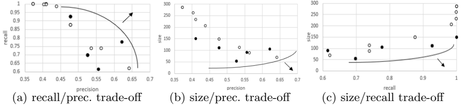
Fig. 11: BPIC 2013 Pareto fronts: IM–AOL nets (“●”) and AM–AOL MAS nets (“○”).
