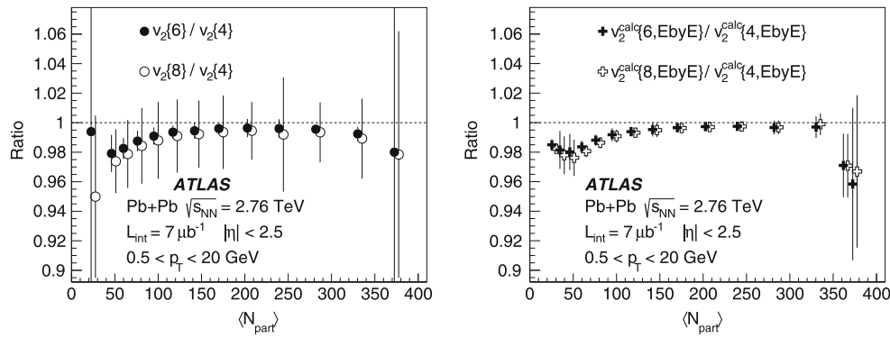
Fig. 9 The ratio of v_2\{6\} and v_2\{8\} to v_2\{4\} as a function of the average number of participating nucleons, \langle N_{\text{part}} \rangle , for elliptic flow coefficients obtained from the cumulant method ( left ) and calculated from the mea-
