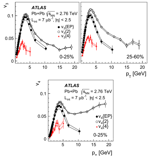
Fig. 5 The transverse momentum dependence of v_3 calculated with two- and four-particle cumulants and with the event-plane method v_3\{EP\} for the centrality interval 0–25 % (top left plot) and 25–60 % (top right plot). The bottom plot shows the same results for v_4 for the centrality interval 0–25 %. Statistical errors are shown as bars and systematic uncertainties as bands. The highest p_T measurement for v_n\{4\} ( v_n\{EP\} ) is integrated over the p_T range 4–20 (8–20) GeV
