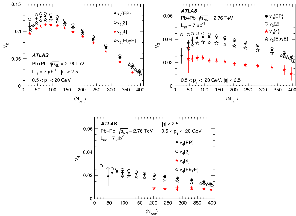
Fig. 10 Comparison of the \langle N_{\text{part}} \rangle dependence of the v_2 ( top left ), v_3 ( top right ) and v_4 ( bottom ) harmonics measured with different methods, with v_n\{\text{EbyE}\} denoting the mean value of the corresponding p(v_n) . The error bars denote statistical and systematic uncertainties added in quadrature
