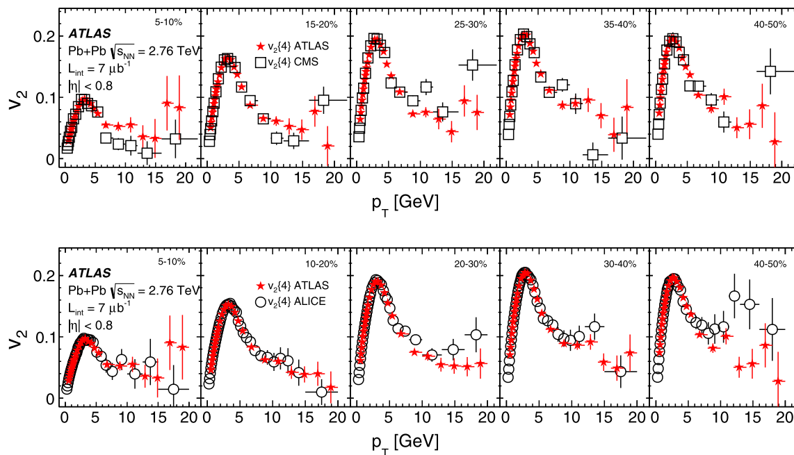
Fig. 4 Comparison of the ATLAS and CMS [20] (top panel), and ATLAS and ALICE [9] (bottom panel) measurements of v_2\{4\} for selected centrality intervals at |\eta| < 0.8 . The error bars denote statistical and systematic uncertainties added in quadrature
