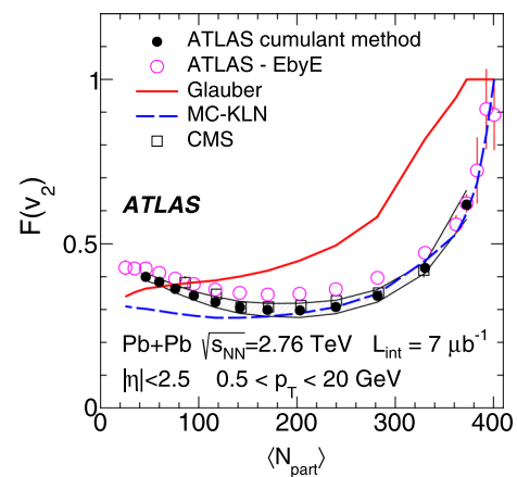
Fig. 13 The relative elliptic flow fluctuations, F(v_2) , as a function of \langle N_{\text{part}} \rangle , from this analysis (filled circles) with v_2\{EP\} substituted for v_2\{2\} . Statistical errors are shown as bars and systematic uncertainties as shaded bands. F(v_2) obtained from the measured v_2 distribution [17] is shown as open circles (marked in the legend as “EbyE”) with the error bars denoting statistical and systematic uncertainties added in quadrature. The same quantity calculated from the initial eccentricity distributions obtained from the Glauber [37] and MC-KLN [46] models is shown by curves. Open squares show the CMS measurement of F(v_2) [23]
