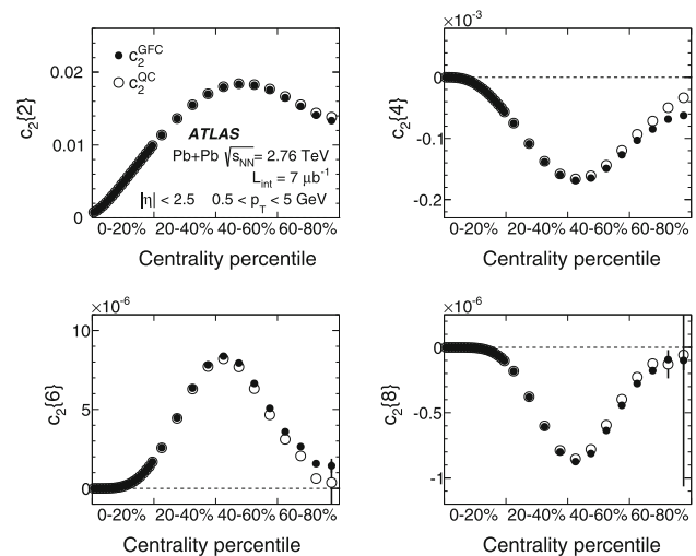
Fig. 1 Multi-particle cumulants for the second-order flow harmonic, c_2\{2k\} for k = 1, 2, 3, 4 , obtained with the GFC [29] and QC [30] methods shown as a function of centrality. The horizontal axis ranges from central collisions (0–20 %) to more peripheral collisions (60–80 %)
