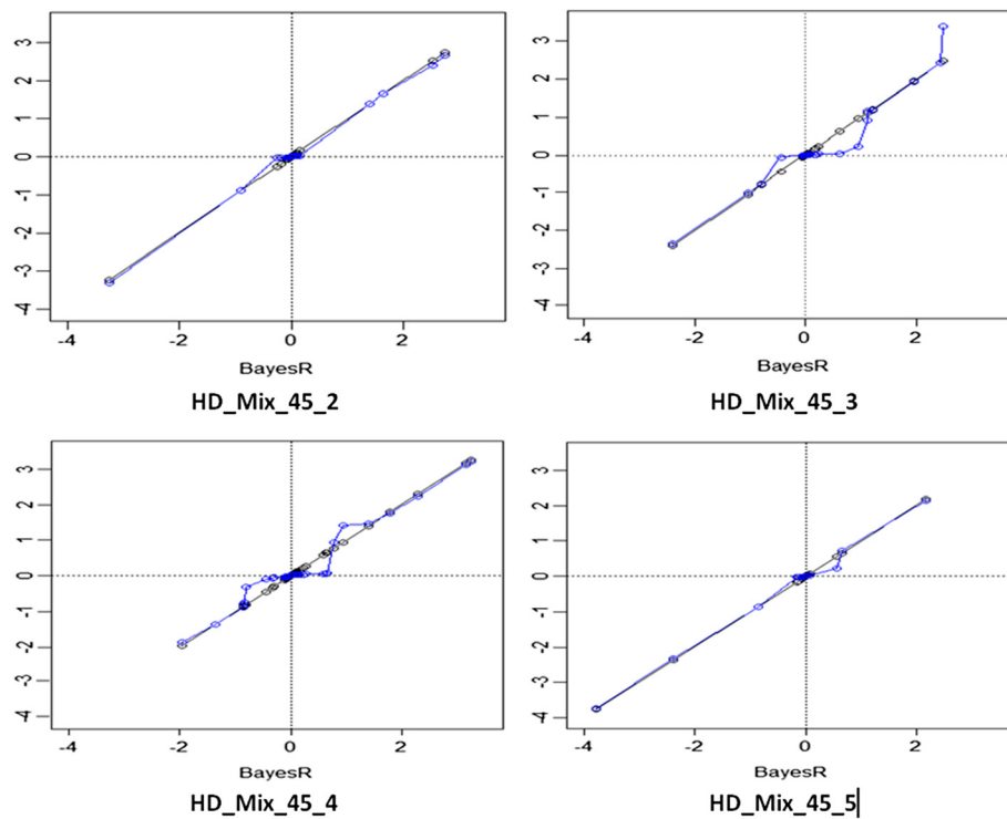
Figure 2 Correlation between SNP effects from BayesR and emBayesR SNP effects in four replicates of HD_Mix_45 ( h^2 = 0.45 ). The x axis represents the BayesR estimates of SNP effect; blue line plots emBayesR estimates of SNP effects on BayesR estimates of SNP effects; black line plots BayesR estimates of SNP effects on themselves for four replicates of HD_Mix with a heritability of 0.45.
