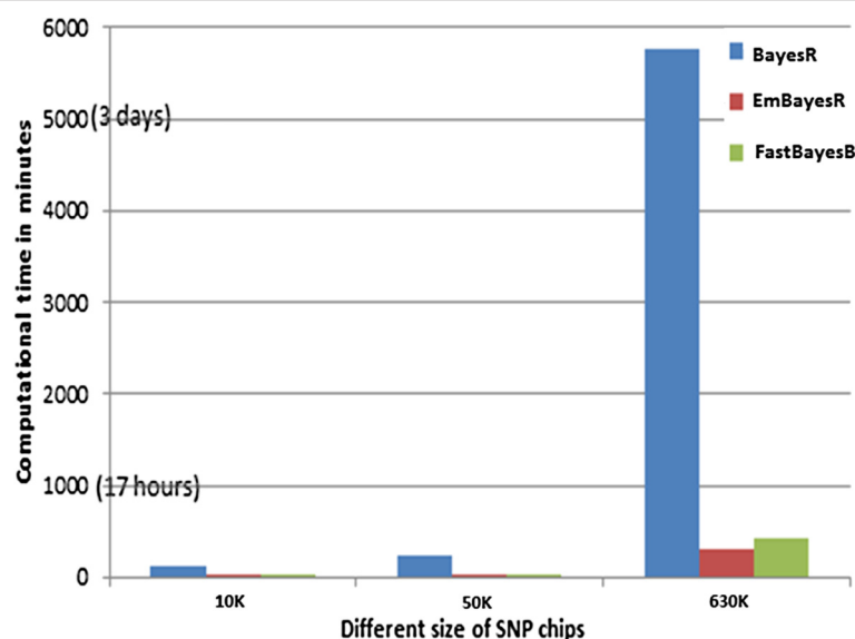
Figure 7 Computational time required for BayesR, emBayesR and FastBayesB on a range of SNP chips (10 K, 50 K and 630 K). The x axis represents the different sizes of the SNP chips, y axis is the computational time in minutes; blue bar is BayesR's running time; red bar is emBayesR's; green bar is FastBayesB's computing time.
