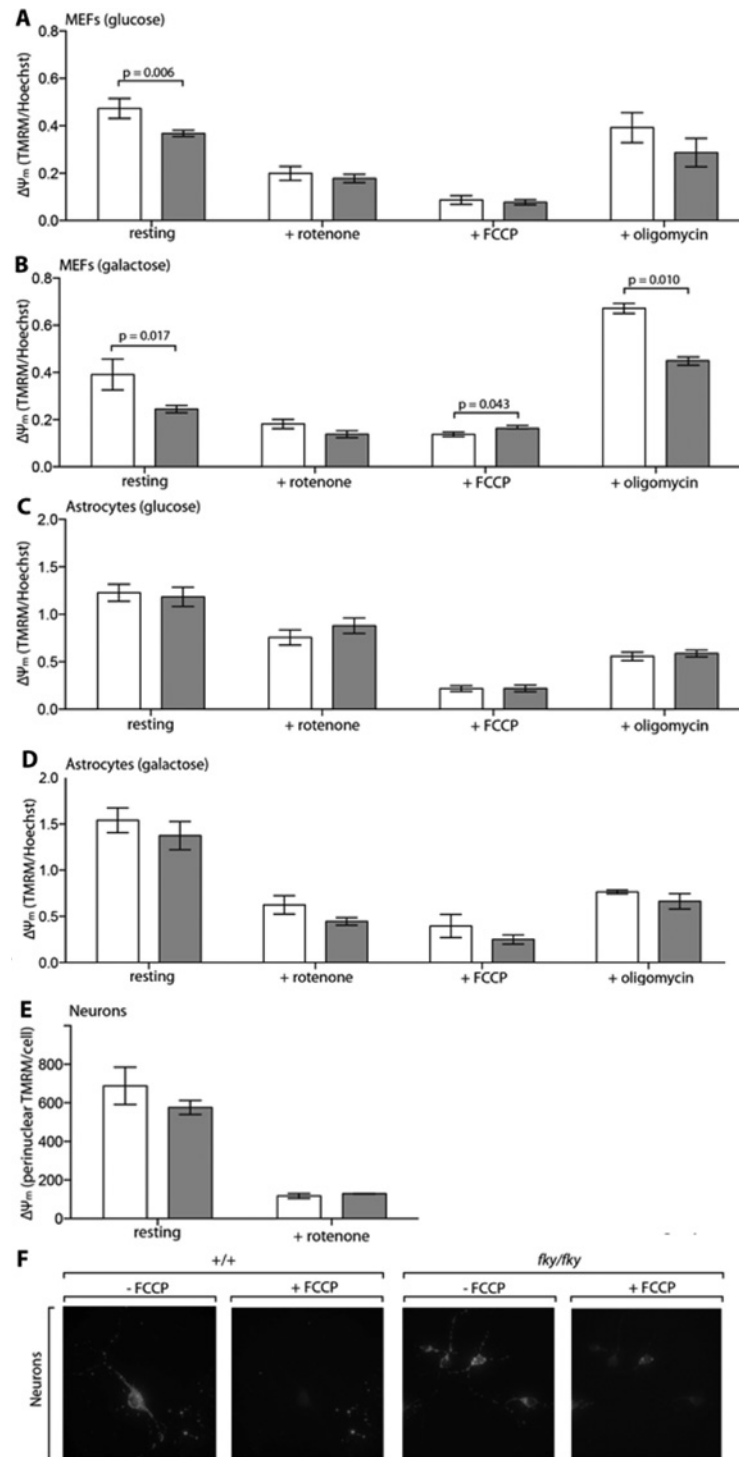
Figure 3 Analysis of the \Delta\Psi_m in Ndufs4 flky/flky cell lines
