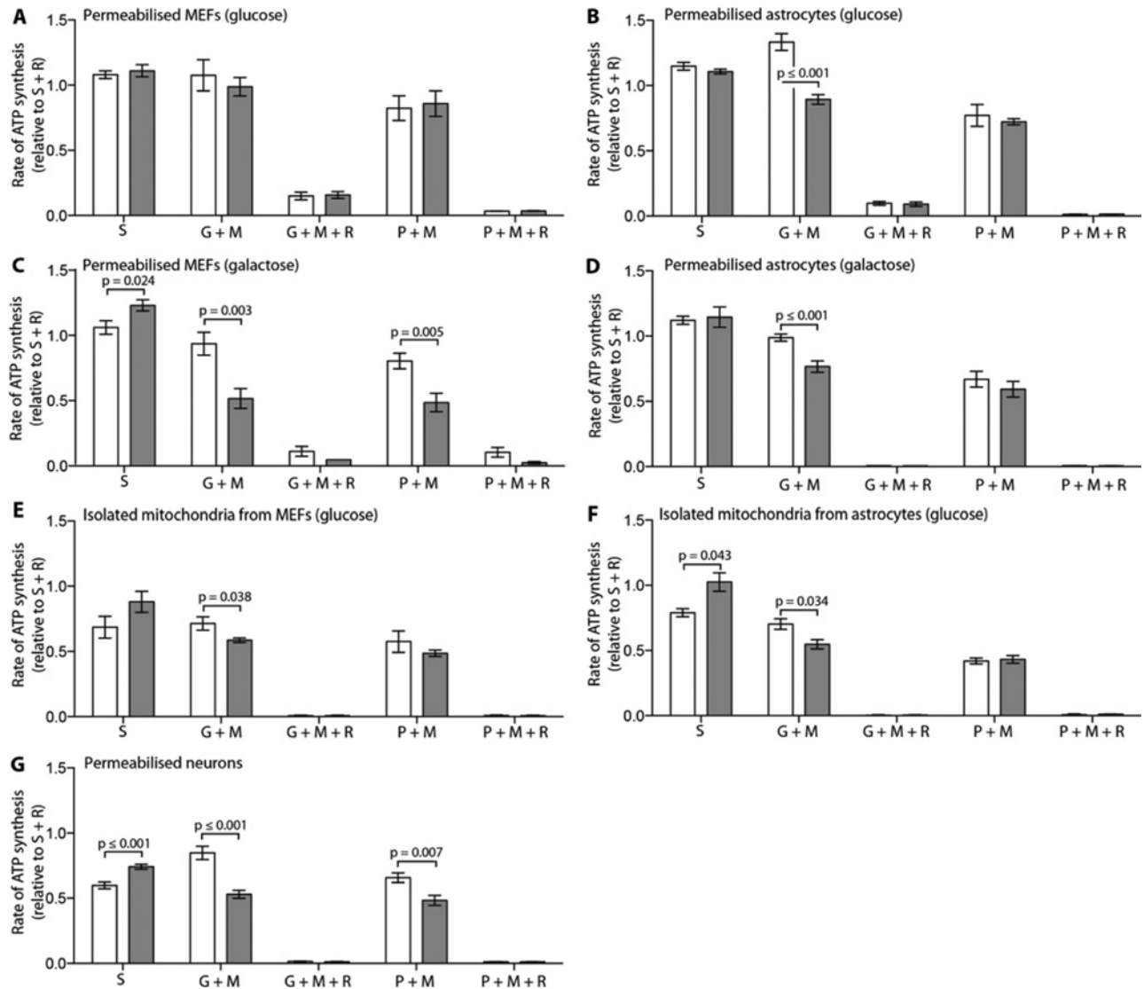
Figure 4 Rates of ATP synthesis in Ndufs4 flky/flky cell lines, expressed relative to the CII-dependent rate determined using succinate + rotenone (S + R)
