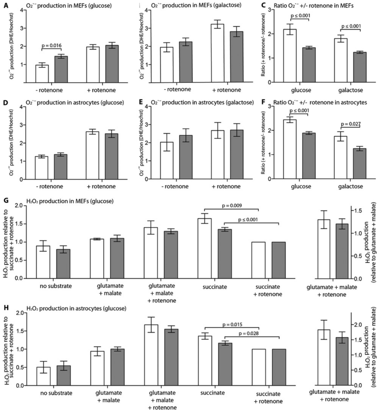
Figure 5 O_2^{\bullet-} and H_2O_2 production in Ndufs4 fky/fky cell lines
