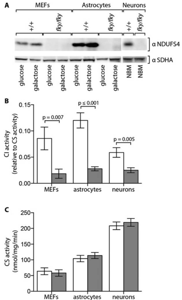
Figure 1 CI activity in Ndufs4 fky/fky cell lines
