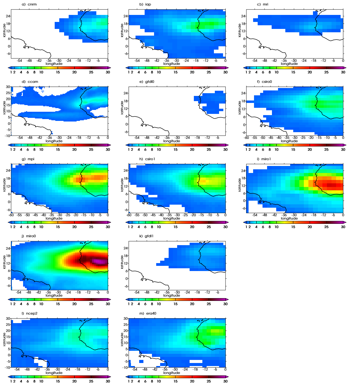
Figure 3: As in Fig. 2, except for 3-5 day Bandpass filtered variance of the meridional wind ( m^2/s^2 ) at 850 mb and l) for ncep2, m) for era40.
