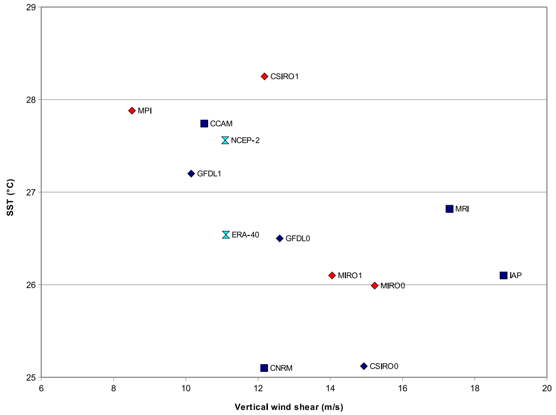
Figure 9: As in Fig. 5 except for SST (C) versus wind shear (m/s) between 850 hPa and 200 hPa. Red (resp. dark blue) points denote simulations with a high (resp. low to moderate) AEW activity. Light blue double triangles represent reanalyses.
