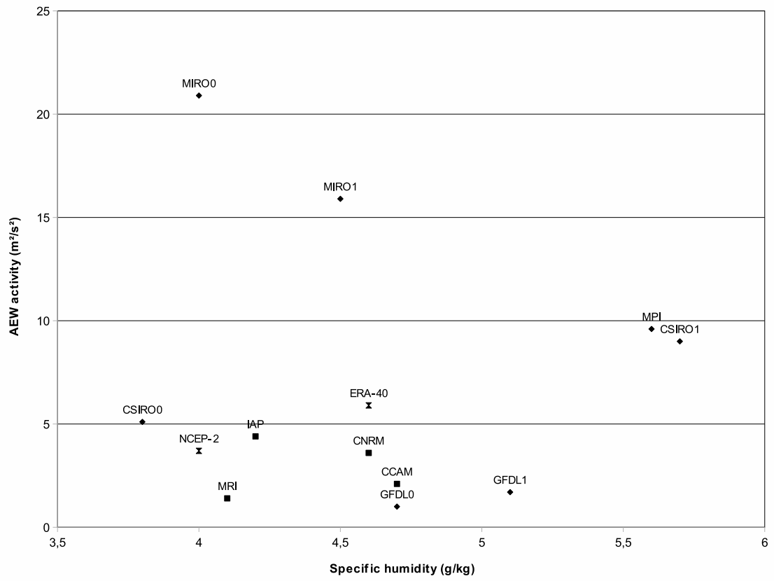
Figure 8: As in Fig. 5 except for AEW activity (m 2 /s 2 ) versus specific humidity at 600 hPa (g/kg; 5N-15N, 15W-30W).
