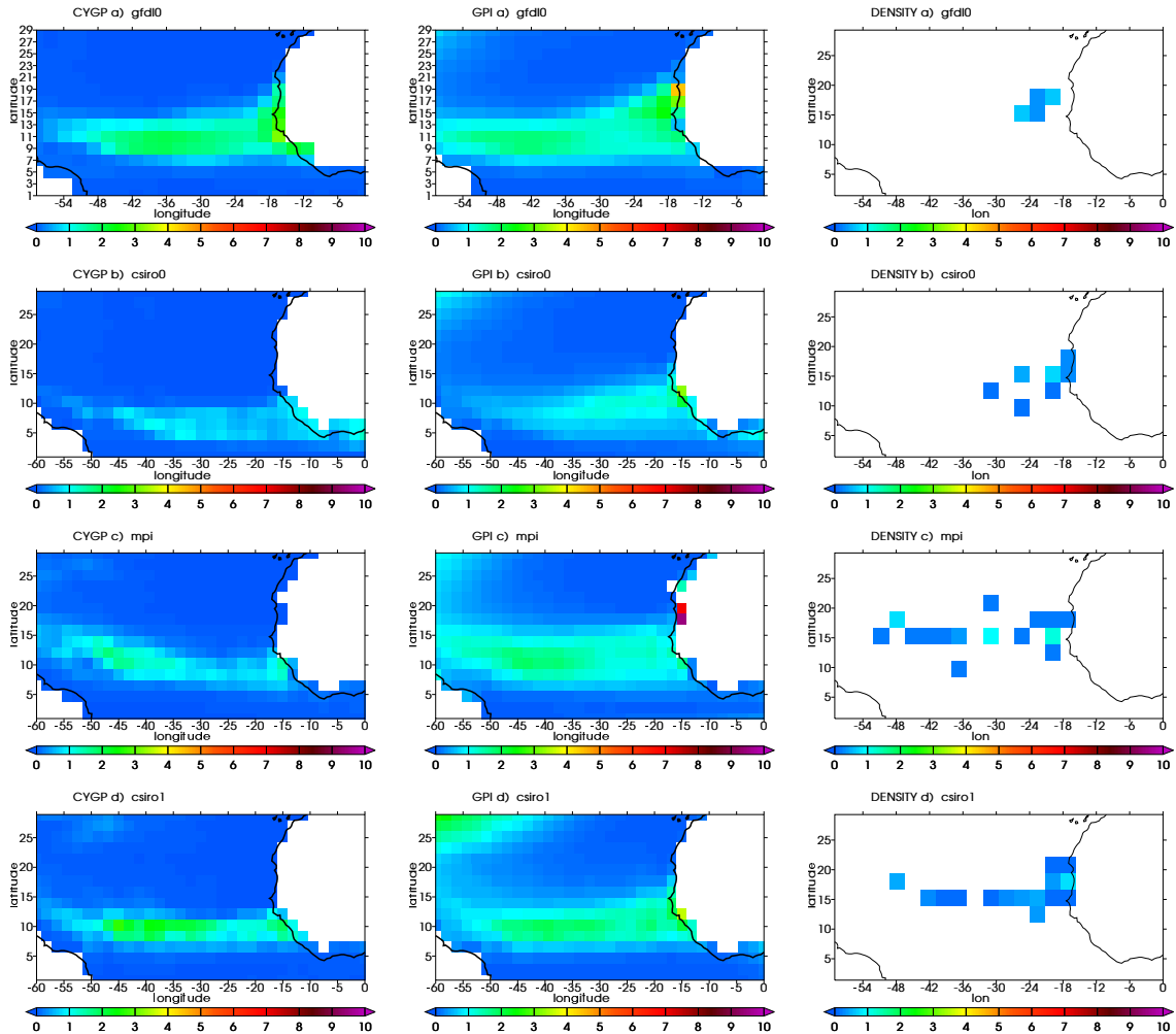
Figure 11: As in Fig. 10 except for simulations with moderate TC activity: a) gfdl0, b) csiro0, c) mpi and d) csiro1. All these models have a moderate TC activity (cf. Table 2).
