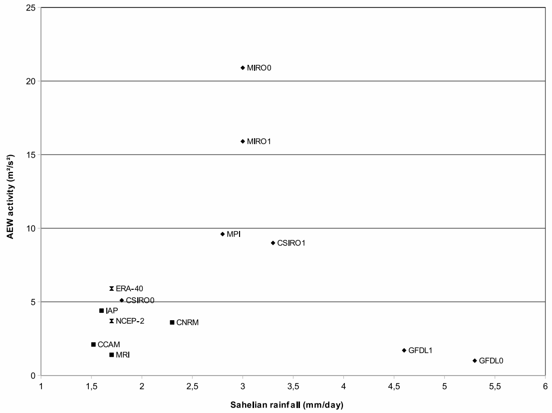
Figure 5: Scatter plot of the AEW activity ( m^2/s^2 ) versus Sahelian rainfall for JAS 1980-1998. Diamonds represent simulations producing TCs, squares those not producing TCs and double triangles represent reanalyses.
