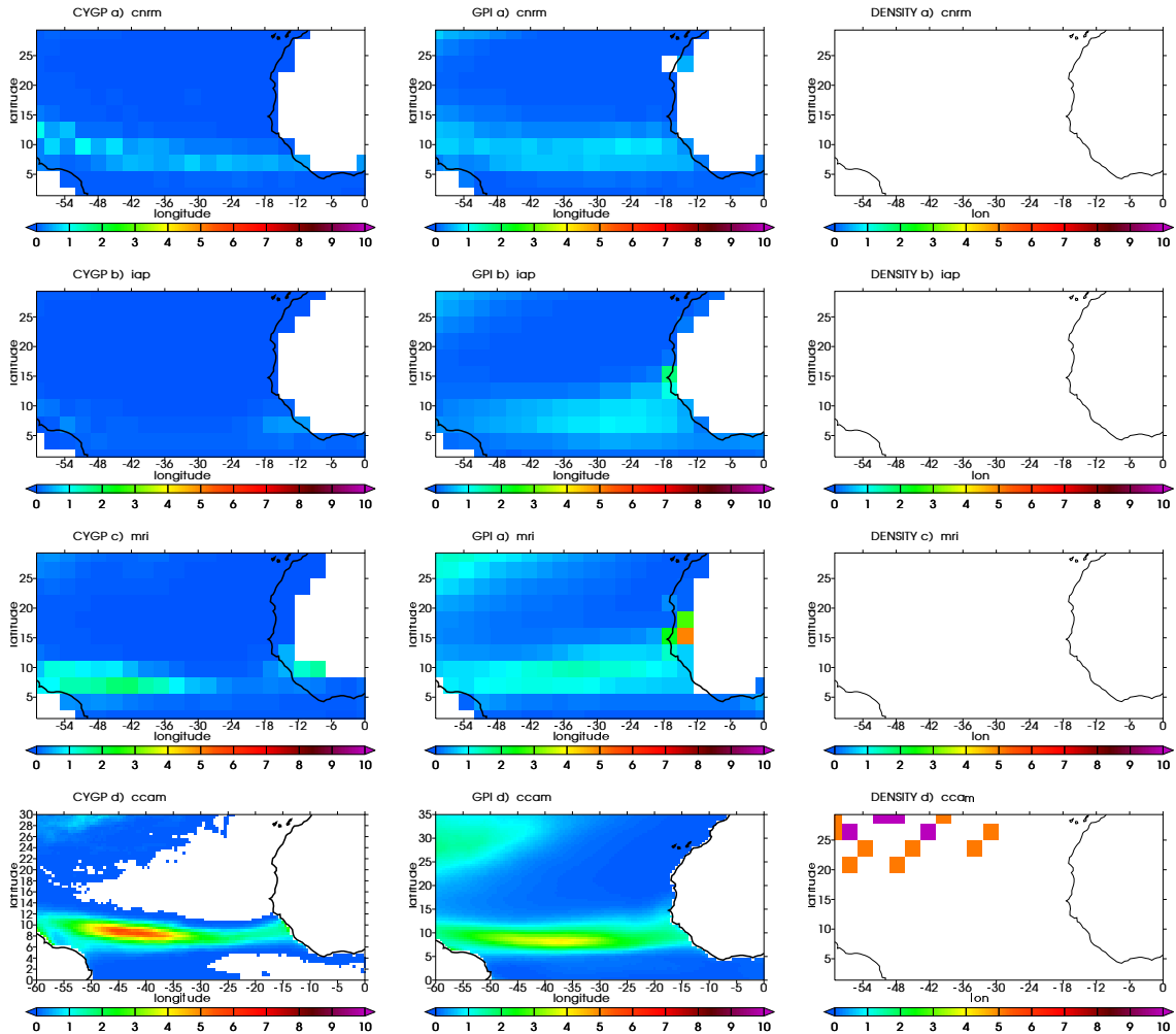
Figure 10: CYGP (left column), GPI(middle column) and density of genesis of TCs per 20 years per 5 degrees by 5 degrees boxes (right column) for simulations with low TC activity : a) cnrm, b) iap, c) mri and d) ccam.
