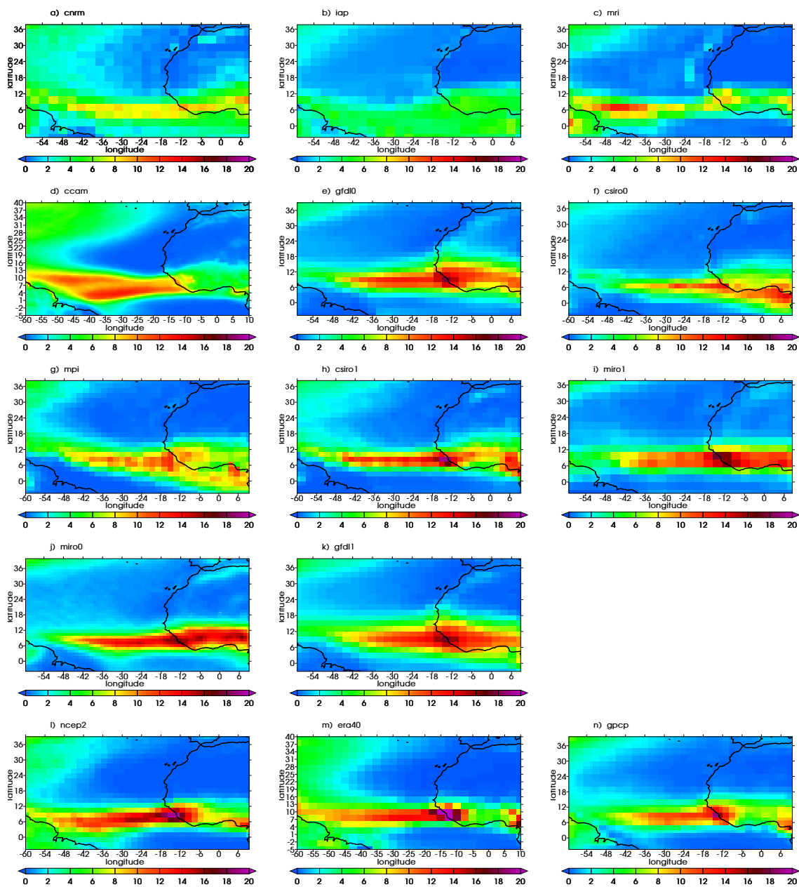
Figure 4: As in Fig. 3 except for total precipitation (mm/day), and n) for gpcp.
