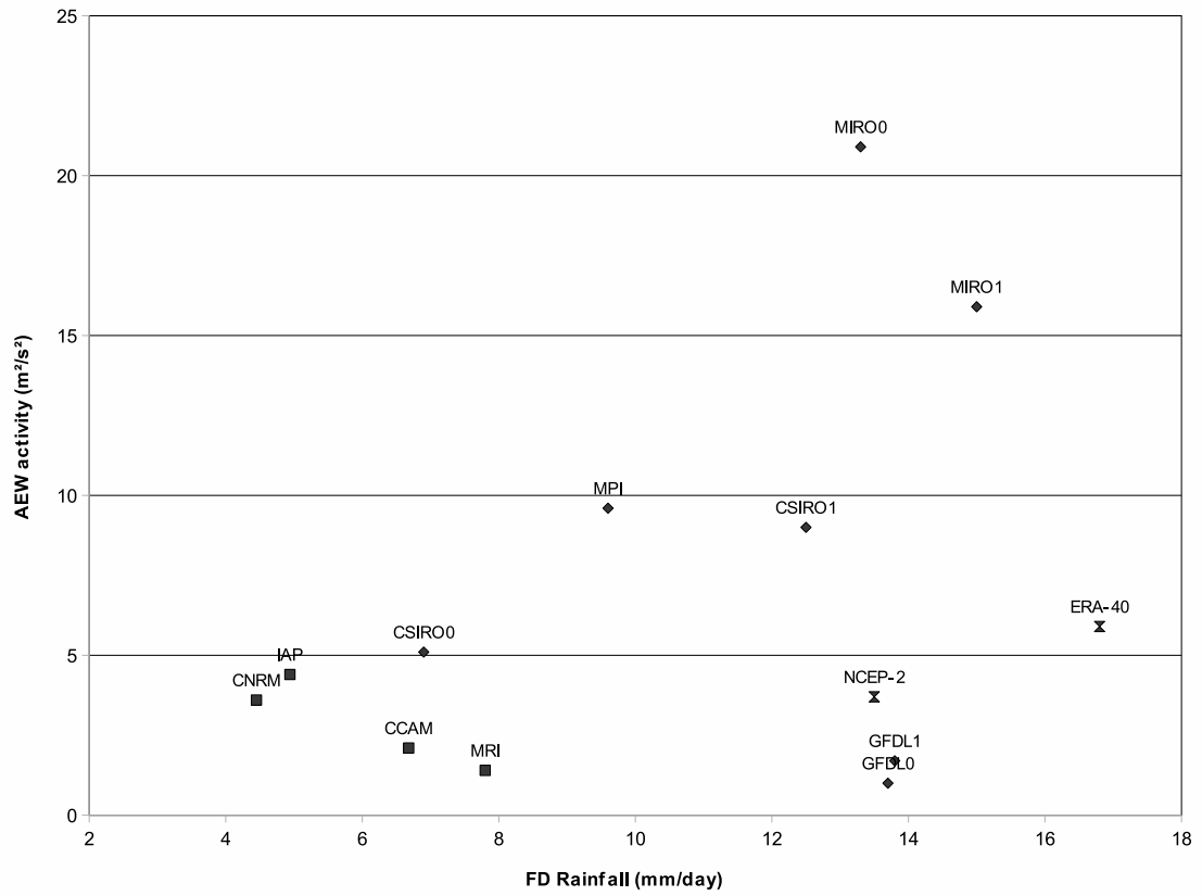
Figure 7: As in Fig. 5 except AEW activity (m 2 /s 2 ) versus the Fouta Djallon rainfall (mm/day).
