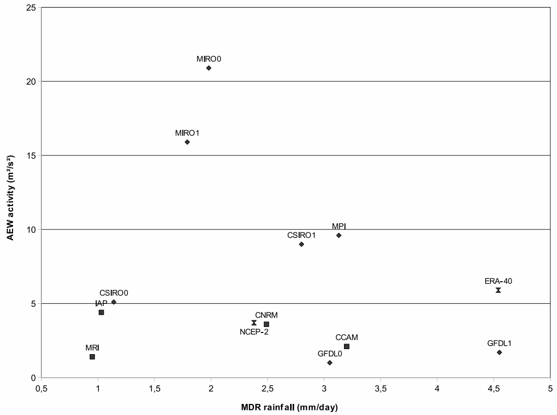
Figure 6: As in Fig. 5 except for AEW activity (m 2 /s 2 ) versus MDR rainfall (mm/day).
