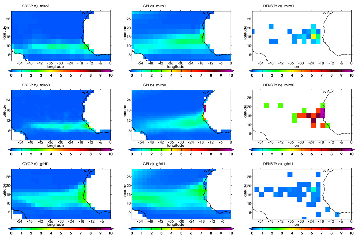
Figure 12: As in Fig. 10, except for simulations with high TC activity : for a) miro1, b) miro0 and c) gfdl1.
